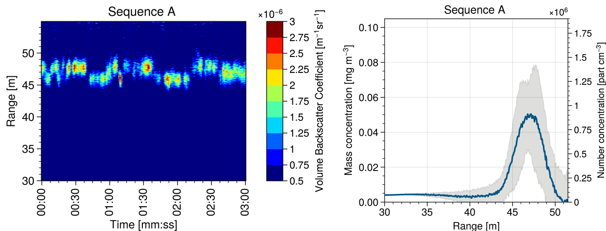
Figure 3. Time-range map of the volume backscatter coefficient (left). Retrieved nvPM mass and number concentration profiles.
