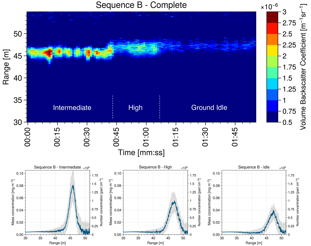
Figure 4. Time-range map of the volume backscatter coefficient (top) and retrieved nvPM mass and number concentration profiles (bottom) under three engine thrust conditions: intermediate, high, and idle.
