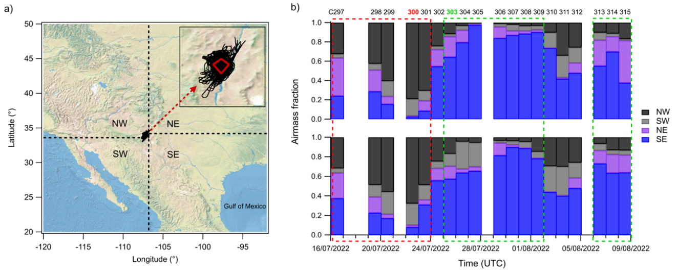
290 Figure 1. a) Flight tracks during the DCMEX aircraft campaign (designated flight labels from C297 to C315). Each flight followed a designated kite-shaped pattern (red solid lines) over the Magdalena Mountains, New Mexico, USA. Black dashed lines represent four different regions used for air mass source classification. b) Fractional contributions of different source regions to the air parcels arriving at the sampling area throughout the field experiment. The bottom plot represents low-level simulations, and the upper plot represents high-level simulations. The dashed red box represents flights included in Period 1, and the green boxes represent flights included in Period 2. The corresponding flight numbers are indicated in the plot, and the two flights (C300 and C303) used for case 295 simulations with bin microphysics parcel model are highlighted in red and green colours.
