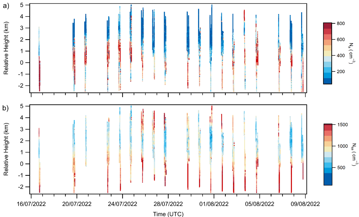
Figure 3. Vertical profiles of out-of-cloud a) N_a (0.1 to 3 \mu\text{m} ) from PCASP measurements and b) N_{sa} (2.5 nm to 1 \mu\text{m} ) from CPC measurements, for each flight. The y-axis is the relative height with respect to the LCL height.
