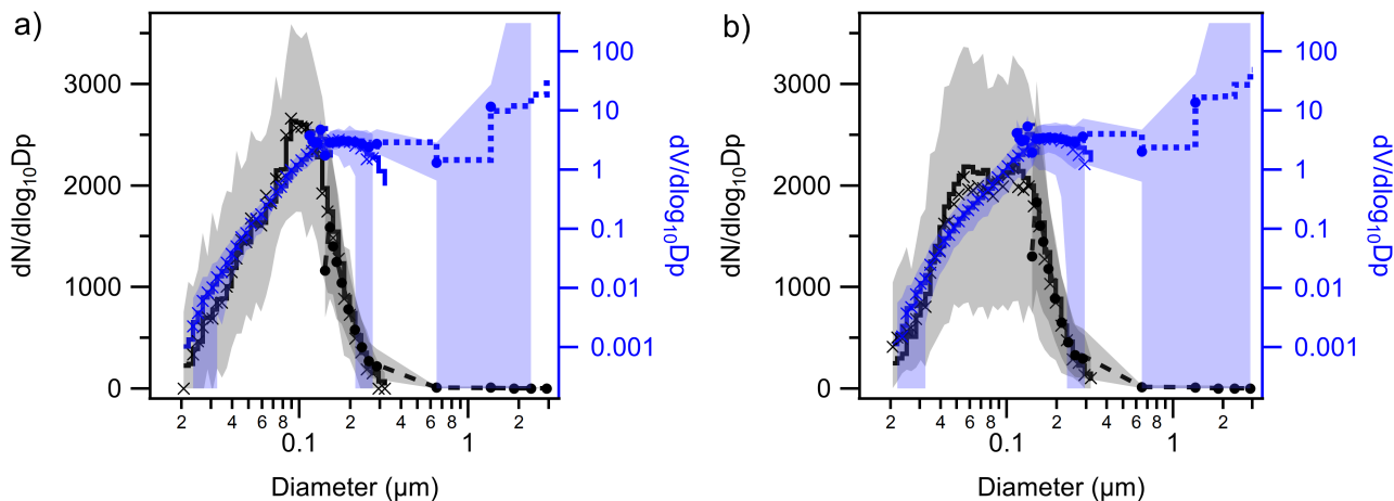
Figure 4. Aerosol size distributions over near cloud-base SLRs for a) Period 1 and b) Period 2. The black lines, markers, and shades show mean, median, and 10 to 90 percentiles of number size distributions (left axis). The blue lines, markers, and shades show mean, median, and 10 to 90 percentiles of volume size distributions (right axis). The solid lines and cross markers represent results from SMPS; dashed lines and circle markers represent results from PCASP.
