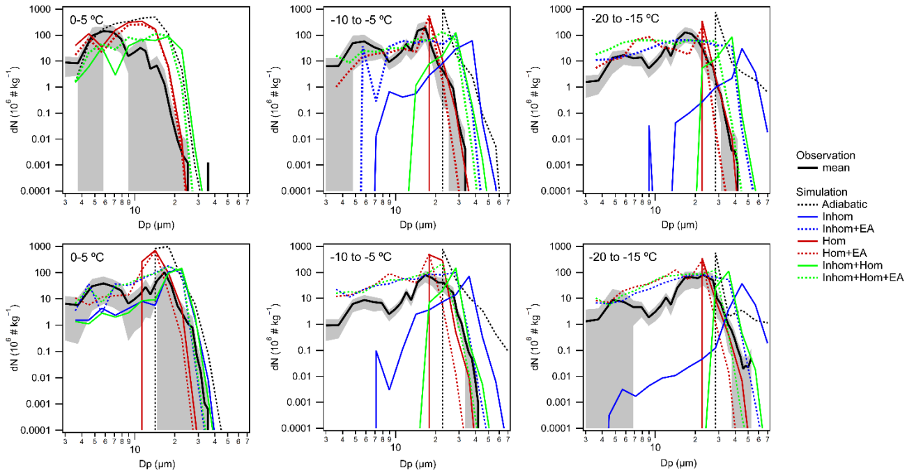
620 Figure 8. Observed and simulated cloud droplet size distributions for the Period 1-C300 case (upper plots) and the Period 2-C303 case (bottom plots), as a function of T ranging from near cloud base to high level. The black solid lines and shades represent mean values and standard deviations of observed values within specific T ranges. The black dashed, blue, red, and green lines represent simulations under different scenarios.
