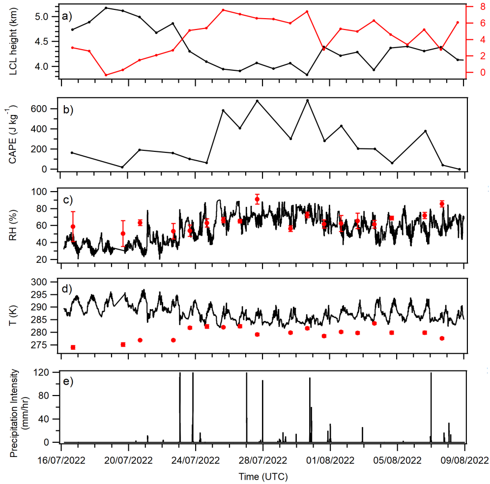
Figure 2. From the top to the bottom: a) Daily LCL (left axis) height and T_{LCL} (right axis) during the DCMEX campaign, which is estimated from Magdalena observations (15:00–16:00 UTC period). b) The calculated convective available potential energy (CAPE), based on dropsonde observations in each flight. c, d) Time series of surface RH and T observed at Langmuir Laboratory, along with the corresponding near cloud-base RH and T for each flight, the red markers and error bars represent mean values and standard deviations within 200 m below the LCL height. e) Time series of precipitation intensity observed at Langmuir Laboratory.
