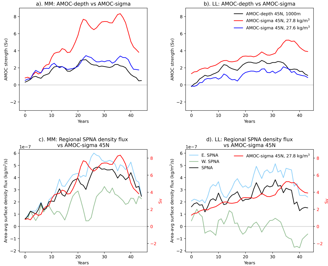
Figure 7. Panels a). and b). show the time series of the anomalous AMOC strength at 45°N, at depth of 1000m (AMOC-depth 45°N, black), the timeseries of the maximum anomaly of the AMOC in density space at 45°N (AMOC-sigma 45°N) at density of 27.8 kg/m 3 (red), and AMOC-sigma 45°N) at density of 27.6 kg/m 3 (blue), for the MM and LL models respectively. Panels c). and d). show the time series of annual-mean anomalies of area-averaged surface density fluxes across the subpolar North Atlantic (SPNA, black) and contributions from the eastern (blue) and western (green) portion of the SPNA for the N216 and N96 models, respectively. The SPNA region is defined as (45°N-65°N,65°W-0°W) and shown by black box in Figure 9. The eastern and western portions are separated at Cape Farewell, shown by grey dashed line in Figure 9. All variables are smoothed by a 5-year running mean.
