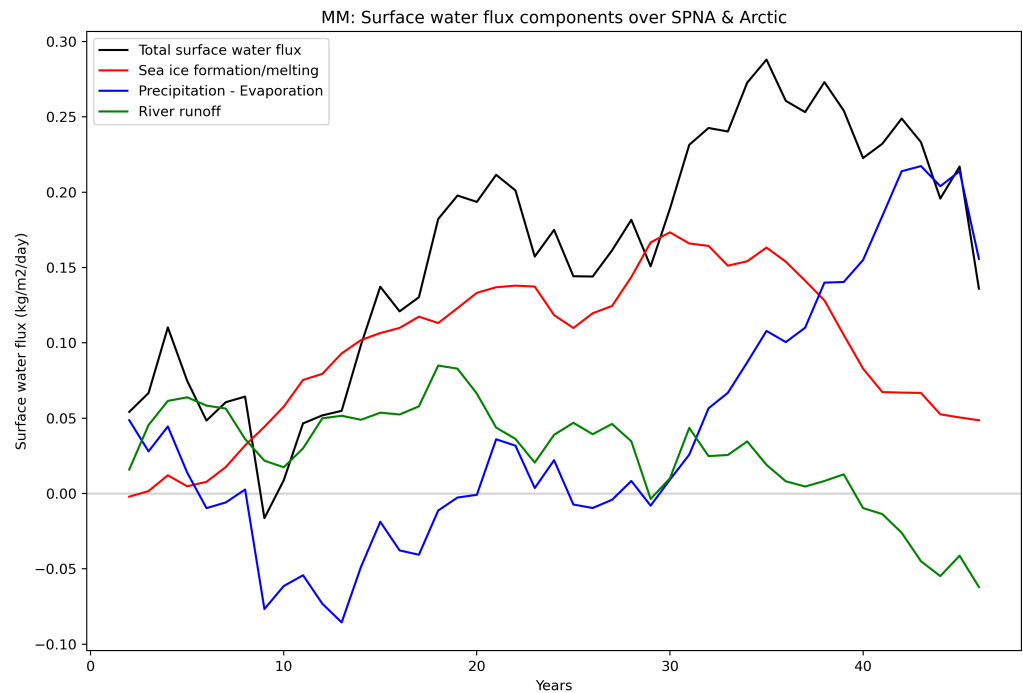
Figure C1. Time series of the anomalous total surface water flux (black) averaged across the Arctic and subpolar North Atlantic (45°N to 65°N, 85°W to 35°E) alongside its decomposition; water flux due to sea ice melt/formation (red), precipitation minus evaporation (blue) and river runoff (green). Positive denotes anomalous surface water flux into the ocean. Only MM is shown. All variables are smoothed by a 5-year running mean.
