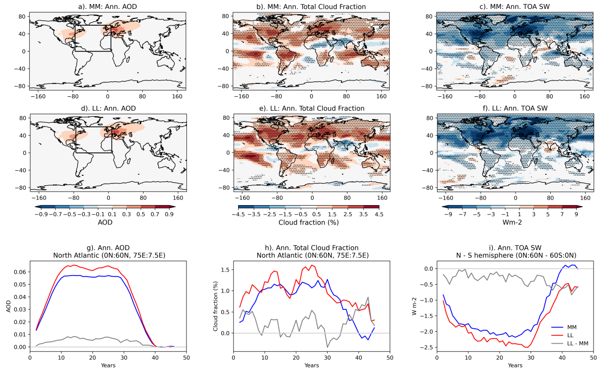
Figure 2. Spatial pattern and timeseries of the forced changes in aerosol optical depth (AOD), total cloud fraction and top-of-atmosphere net downward shortwave radiation (TOA SW). Panel a). shows the spatial pattern of anomalous AOD averaged across years 10-30 of the forced simulation for MM. Panel b). shows the same as a). but for the total cloud fraction. Panel c). shows the same as a). but for TOA SW. Stippling indicates where the response is significant at the 10% level, based on a two-tailed Student's t-test. Panels d), e), and f) shows the same as a), b), and c) but for LL. Panel g). shows the timeseries of area-averaged annual-mean aerosol optical depth (AOD) taken across the North Atlantic basin (0°N to 60°N, 7.5°E to 75°E). Panel h). shows the same as g). but for the total cloud fraction instead of AOD. Panel i). shows the interhemispheric difference (0°N to 60°N minus 0°S to 60°S) in downwards top-of-atmosphere net shortwave radiation (TOA SW) for MM (blue) and LL (red). The difference between the two models is shown in grey. All timeseries are smoothed by a 5-year running mean.
