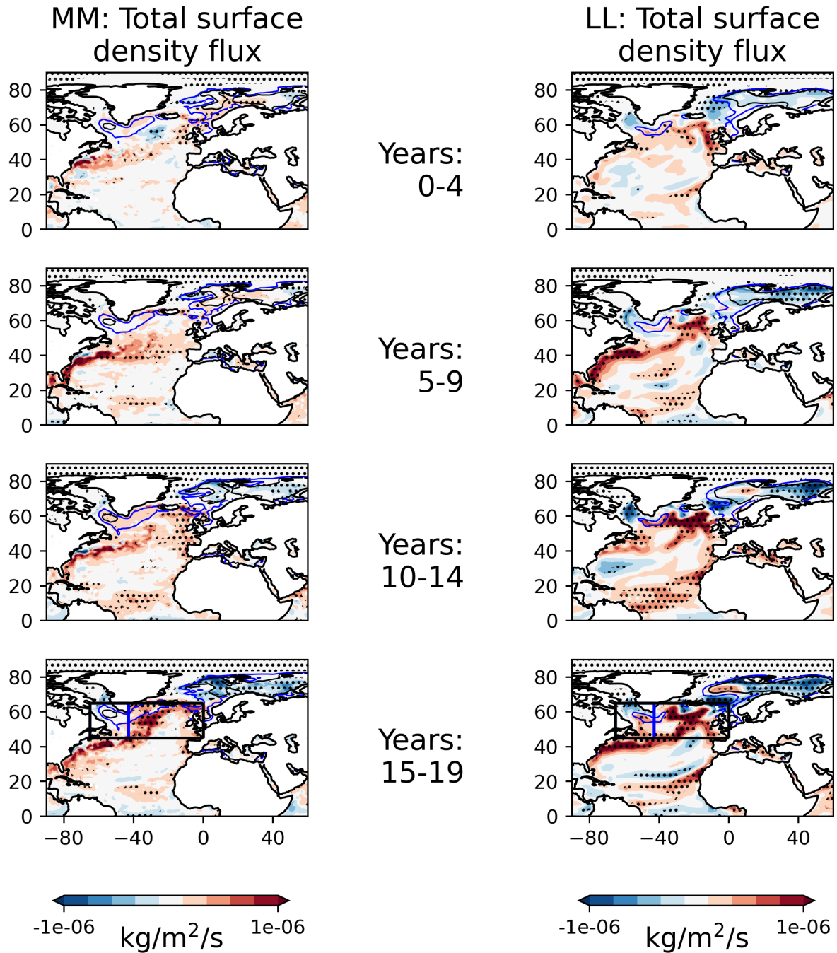
Figure 8. Spatial pattern and evolution of total surface density flux. Contours mark areas where key isopycnals outcrop to the surface in oceanic winter. The blue and black contours regions show where the isopycnals of 27.6 \text{ kg/m}^3 and 27.8 \text{ kg/m}^3 respectively, outcrop to the surface in the extended late-winter months (January-February-March-April, JFMA). All variables are smoothed by a 5-year running mean. MM is shown on the left and LL is shown on the right. The black box in the bottom panels denote the subpolar North Atlantic (SPNA) region defined as ( 45^\circ\text{N} - 65^\circ\text{N} , 65^\circ\text{W} - 0^\circ\text{W} ). Stippling indicates where the response is significant at the 10% level, based on a two-tailed Student's t-test
