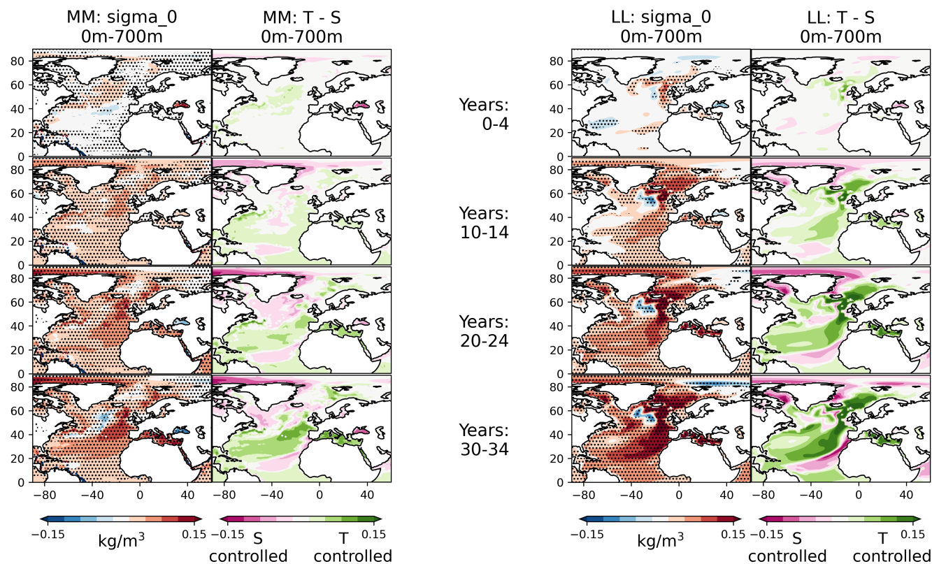
Figure 11. Spatial pattern and evolution of the annual-mean, ensemble-mean upper-ocean (0m-700m) potential density anomalies referenced to the ocean surface ( \sigma_0 ) alongside the relative importance of the thermal and haline components. Pink denotes that the density anomaly is dominated by the haline component and green denotes a thermal dominance. MM is shown on the left and LL is shown on the right. Stippling indicates where the response is significant at the 10% level, based on a two-tailed Student's t-test.
