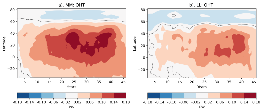
Figure 5. Hovmöller plot of northward OHT anomalies in the North Atlantic basin. Hovmöller diagrams of annual-mean, ensemble-mean anomalies of ocean heat transport (OHT) by latitude and time. Panels a). shows the MM version of the model and panel b). shows LL. All variables are smoothed by a 5-year running mean. All shaded regions are significant at the 10% level based on a two-tailed Student’s t-test. Stippling is left out for clarity.
