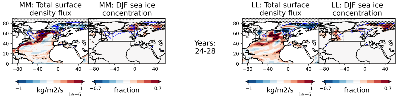
Figure 9. Spatial pattern of the annual-mean, ensemble-mean anomalies of surface density fluxes and December-January-February sea ice concentration (DJF SIC). All variables are smoothed by a 5-year running mean such that Years:24-28 represents the mean value between years 24 and 28. MM is shown on the left and LL is shown on the right. The blue and black contour lines represent the surface density levels of 27.6 \text{ kg/m}^3 and 27.8 \text{ kg/m}^3 respectively. The black box denotes the subpolar North Atlantic (SPNA) region. The eastern and western portions are separated at the cape of Greenland, shown by grey dashed line. Stippling indicates where the response is significant at the 10% level, based on a two-tailed Student's t-test.
