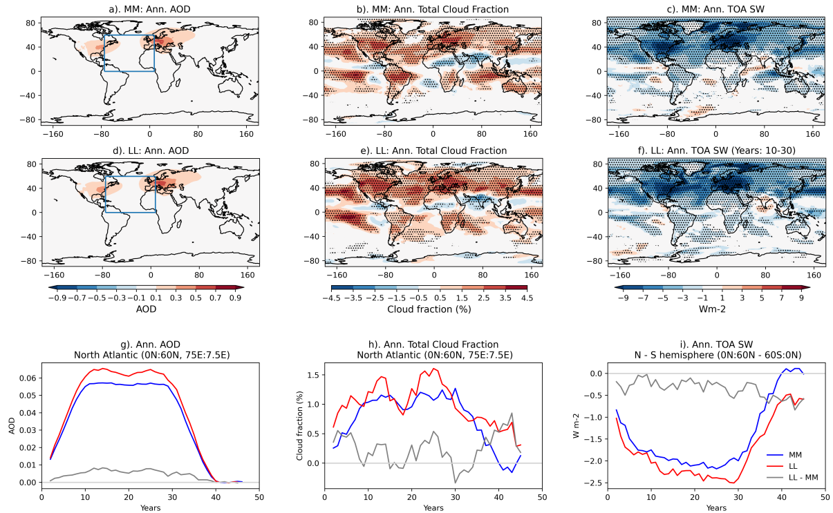
Figure 2. Spatial pattern and timeseries of the forced changes in aerosol optical depth (AOD), total cloud fraction and top-of-atmosphere net downward shortwave radiation (TOA SW). Panel a). shows spatial pattern of anomalous AOD averaged across years 10-30 of the forced simulation for MM. Panel b). shows the same as a). but for total cloud fraction. Panel c). shows the same as a). but for TOA SW. Stippling indicates where the response is significant at the 10% level, based on a two-tailed Student's t-test. Panel d), e), and f) shows the same as a), b), and c) but for LL. Panel g). shows the timeseries of area-averaged annual-mean aerosol optical depth (AOD) taken across the North Atlantic basin (0°N to 60°N, 7.5°E to 75°E). Panel h). shows the same as g). but for the total cloud fraction instead of AOD. Panel i). shows the interhemispheric difference (0°N to 60°N minus 0°S to 60°S) in downwards top-of-atmosphere net shortwave radiation (TOA SW) for MM (blue) and LL (red). The difference between the two models are shown in grey. All timeseries are smoothed by a 5-year running mean.
