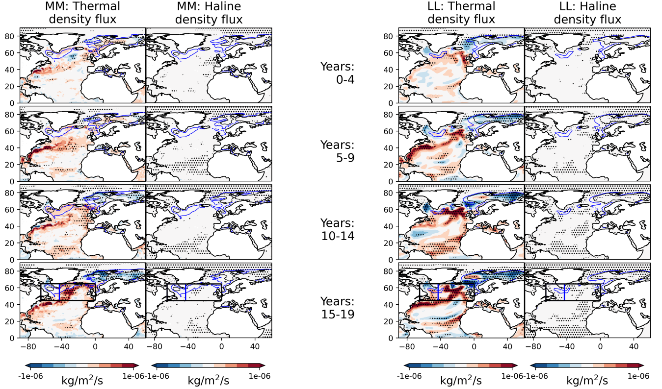
Figure B1. Spatial pattern and evolution of the decomposition of surface density flux into contributions from the haline and thermal components. Contours mark areas where key isopycnals outcrop to the surface in oceanic winter. The blue and black contours regions show where the isopycnals of 27.6 \text{ kg/m}^3 and 27.8 \text{ kg/m}^3 respectively, outcrop to the surface in the extended late-winter months (January-February-March-April, JFMA). All variables are smoothed by a 5-year running mean. MM is shown on the left and LL is shown on the right. The black box in the bottom panels denote the subpolar North Atlantic (SPNA) region defined as ( 45^\circ\text{N} - 65^\circ\text{N} , 65^\circ\text{W} - 0^\circ\text{W} ). Stippling indicates where the response is significant at the 10% level, based on a two-tailed Student's t-test
