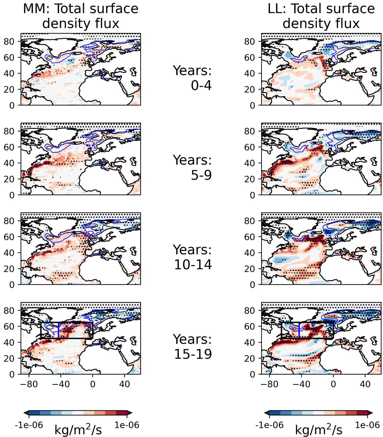
Figure 8. Spatial pattern and evolution of total surface density flux and its decomposition into contributions from the haline and thermal components . Contours mark areas where key isopycnals outcrop to the surface in oceanic winter. The blue and black contours regions show where the isopycnals of 27.6 \text{ kg/m}^3 and 27.8 \text{ kg/m}^3 respectively, outcrop to the surface in the extended late-winter months (January-February-March-April, JFMA). All variables are smoothed by a 5-year running mean. The MM model is shown on the left and the LL model is shown
