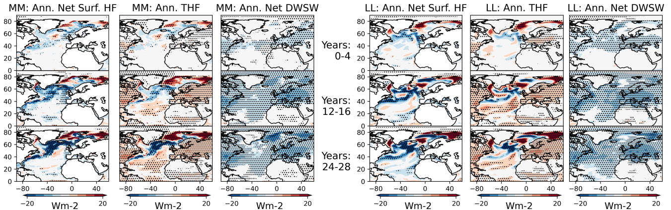
Figure 4. Spatial pattern and evolution of the annual-mean, ensemble-mean anomalies of net surface heat flux, turbulent heat flux (THF) and net downward shortwave radiation (DWSW). The MM model on the left and the LL model on the right. All variables are smoothed by a 5-year running mean. Stippling indicates where the response is significant at the 10% level, based on a two-tailed Student's t-test.
