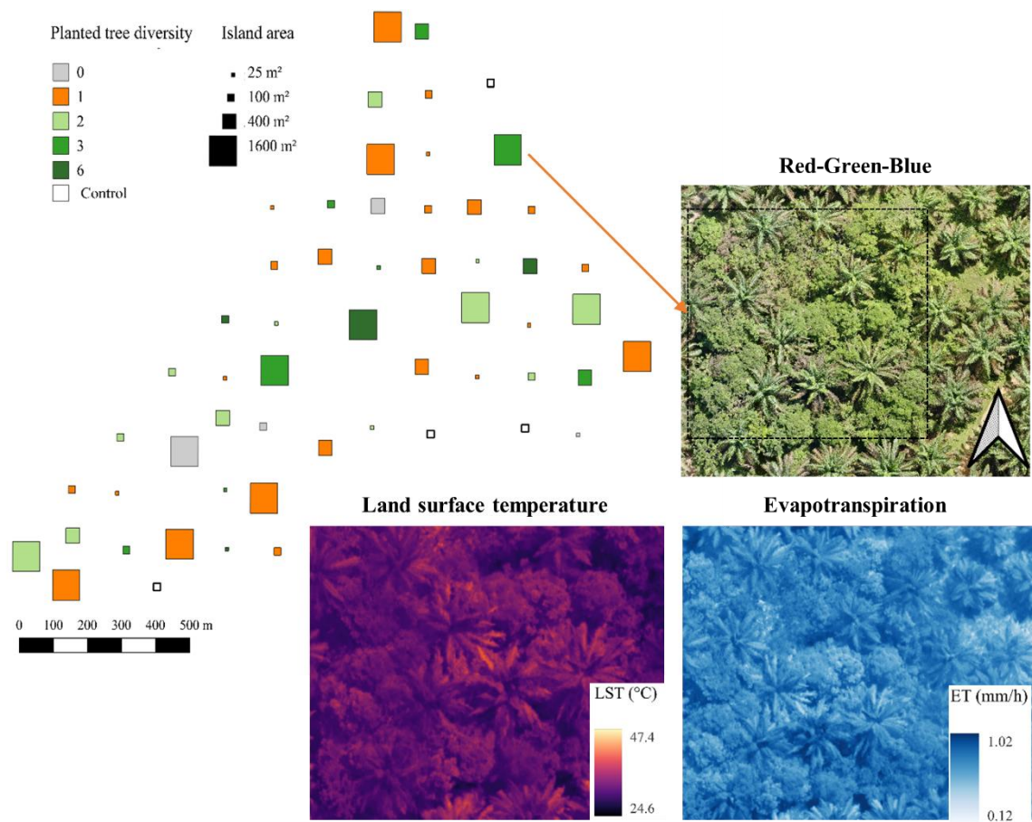
Figure 1: The experimental design of EFForTS-BEE with 52 tree islands varying in planted tree diversity and island area (island size not drawn to scale). The islands are dispersed in a monocultural oil palm plantation of 140 ha. Red-Green-Blue (RGB), land surface temperature (LST, °C) and evapotranspiration (ET, mm h -1 ) of one large tree island (1600 m 2 ) with three planted tree species.
