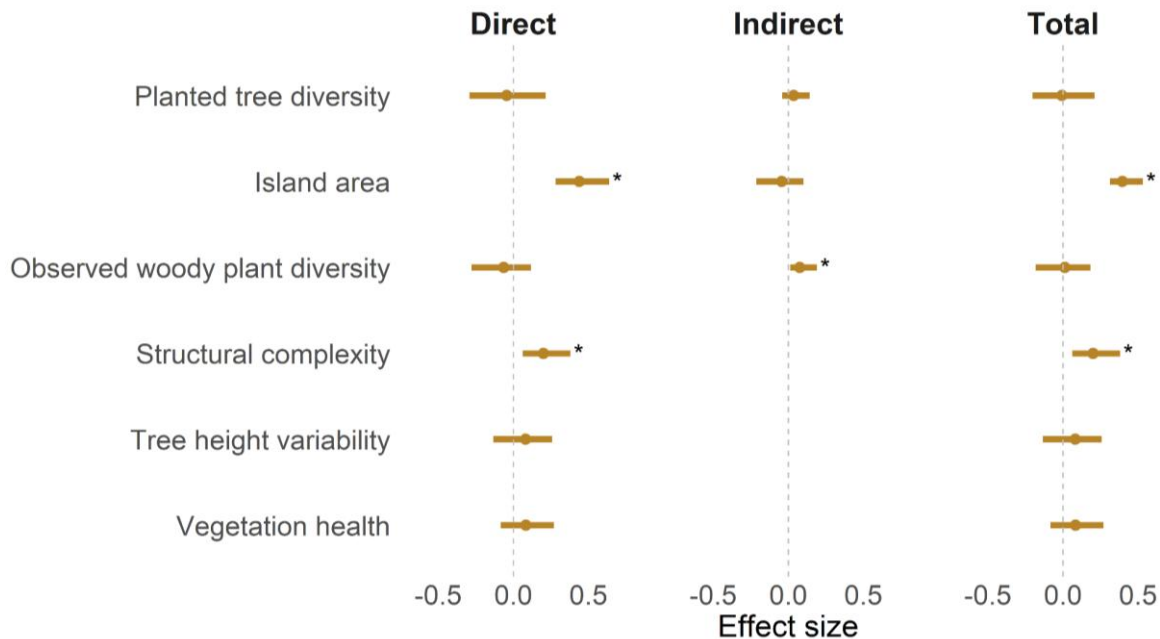
395 Figure 4: Standardized direct, indirect and total effect sizes of predictors on evaporative fraction in SEM. Error bars show 95% CI, derived through bootstrapping with 1000 iterations. Symbols indicate p-value level: * p < 0.05 .
