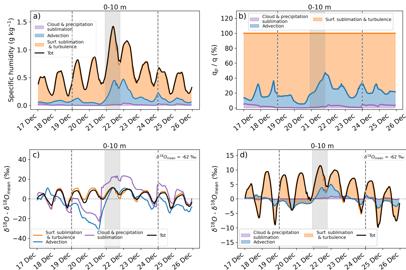
Figure 11. Temporal evolution of the positive contributions of different processes to the surface specific humidity (6.7 m AGL) (a) and their respective percentages (b). Evolution of the \delta^{18}\text{O} anomaly relative to the mean clear-sky diurnal cycle value ( \delta^{18}\text{O}_{\text{mean}} = -62 \text{‰} ), associated with different processes (c). Positive contributions of different processes to the surface \delta^{18}\text{O} anomaly relative to this mean diurnal value (d). The black line represents the signal obtained from total specific humidity and \delta^{18}\text{O} . Individual contributions to specific humidity and \delta^{18}\text{O} are shown in colour: orange for surface sublimation and vertical turbulent diffusion, blue for advection, and purple for cloud and precipitation sublimation. Vertical dashed lines mark the AR period (December 19-23), while the shaded area highlights the peak of the event, reached on December 21 at 09:30 UTC.
