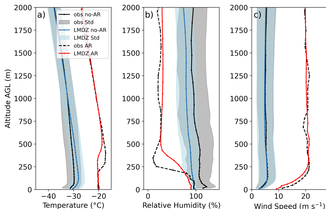
Figure 5. Vertical profiles of (a) temperature ( ^{\circ}\text{C} ), (b) relative humidity with respect to ice (%) and (c) wind speed ( \text{m s}^{-1} ) from the surface to 2000 m AGL, based on average radiosonde measurements at the Concordia station during December 2018 excluding the event (December 19-23) (twice per day, black solid lines) and during the AR event (22 December 2018 at 11:00 UTC, black dashed lines). Corresponding LMDZ model output at the nearest grid point for the same times are shown in blue lines (December averages) and red lines (AR event). The standard deviation is shown in gray for observations and in blue for LMDZ for 52 radiosondes during December 2018 outside the AR event.
