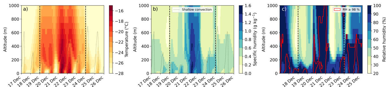
Figure 8. Modelled vertical profiles of a) temperature ( ^{\circ}\text{C} ), b) specific humidity ( \text{g kg}^{-1} ), and c) relative humidity with respect to ice (%) at Concordia. The red outline indicates regions where the relative humidity is higher than 98 %. The dotted lines indicate the height of the mixed layer during shallow convection. The dashed vertical lines delineate the boundaries of the atmospheric river. All times are given in UTC; local time at Concordia is UTC+8, with maximum and minimum solar insolation occurring at 3 am and 3 pm local time, respectively.
