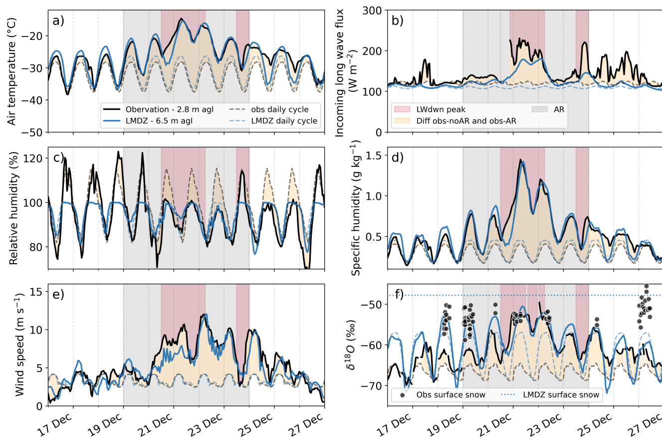
Figure 4. Evolution of (a) air temperature ( ^{\circ}\text{C} ) from the first level of the Concordia meteorological tower (2.8 m AGL), (b) incoming longwave flux from the Baseline Surface Radiation Network, (c) relative humidity with respect to ice (%), (d) specific humidity ( \text{g kg}^{-1} ), (e) wind speed ( \text{m s}^{-1} ) from the first level of the Concordia meteorological tower (3.0 m AGL) and (f) \delta^{18}\text{O} (‰) from the Concordia Picarro instrument (1.0 m AGL). The grey rectangle indicates the period of the AR. The blue line represents the model output (first level: 6.7 m AGL), while the black line corresponds to the observations. The grey and blue dashed lines represent the mean diurnal cycle calculated over the entire month of December 2018, excluding the event (December 19–23), for observations and the model, respectively. The orange shading indicates the difference between the mean clear-sky diurnal cycle and the observations during the event, while the red shading highlights the peaks in downward longwave radiation. Observed surface snow is shown as black dots, while modelled surface snow is represented by a dotted line.
