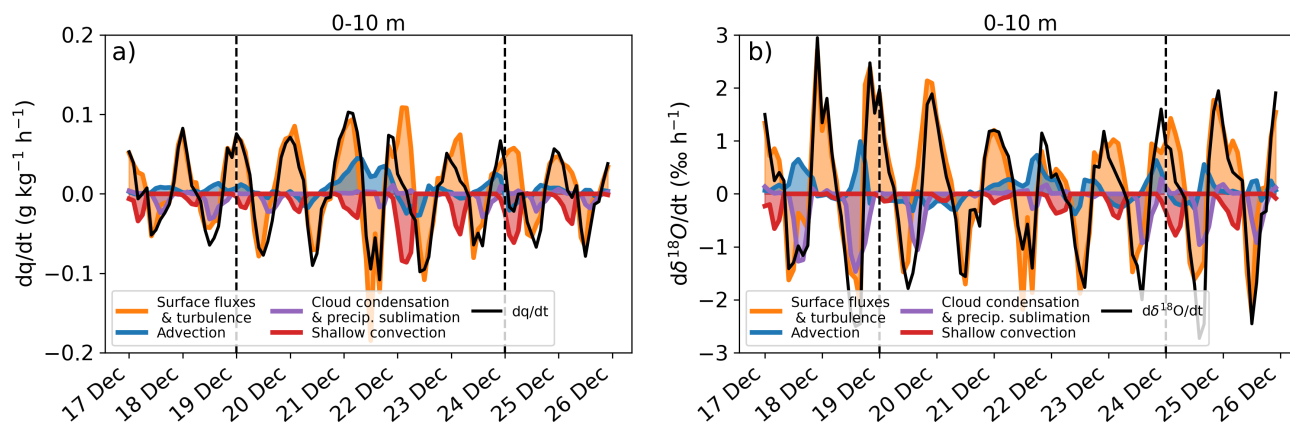
Figure 10. Rate of temporal change of the different surface processes contributing to the (a) specific humidity tendency ( \text{g kg}^{-1} \text{h}^{-1} ) and (b) vapour \delta^{18}\text{O} tendency ( \text{‰ h}^{-1} ) at Concordia station. The black line represents the signal obtained from the first level model output, while the dashed line represents the sum of the different model processes. The individual contributions to the rate of change of humidity and \delta^{18}\text{O} are shown in colour: orange for vertical turbulent diffusion and surface sublimation, blue for advection, purple for cloud condensation and precipitation sublimation and red for shallow convection. It should be noted that the sign of changes is relative to water vapour so the surface sublimation is positive (increase in water vapour) and the cloud condensation is negative (decrease in water vapour). The dashed vertical lines delineate the boundaries of the atmospheric river.
