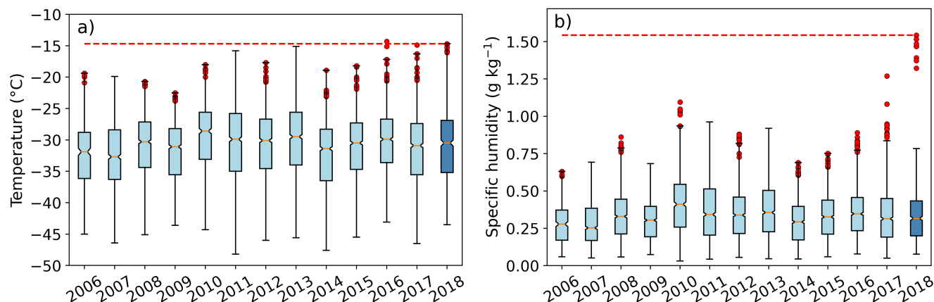
Figure 3. Hourly temperatures (a) and specific humidity (b) recorded at Dome C during summers (December-January) from December 2006 to January 2019 from the AWS. The year of interest, 2018 (December 2018 - January 2019), is coloured in dark blue. Each box is delimited by the 0.25 and 0.75 percentiles and the orange bar represents the median. Black bars indicate the values outside 1.5 times the inter-quartile range. Red circles indicate values outside the 0.99 percentiles. The dotted red line indicate the value reached during the December 2018 AR.
