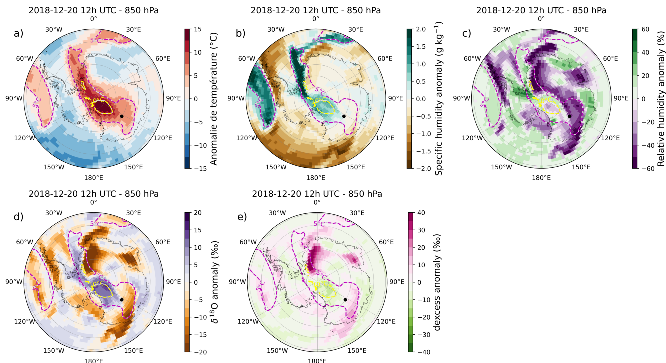
Figure 7. Anomalies at 850 hPa model equivalent level of a) temperature ( ^{\circ}\text{C} ), b) specific humidity ( \text{g kg}^{-1} ), c) relative humidity (%), d) \delta^{18}\text{O} (‰), and e) d-excess (‰), calculated on December 20, 2018 at 12:00 UTC relative to the December average (1980-2021). The purple contour represents the 5^{\circ}\text{C} anomaly boundary, while the yellow contour indicates the 10^{\circ}\text{C} anomaly boundary. The black dot indicates Concordia station.
