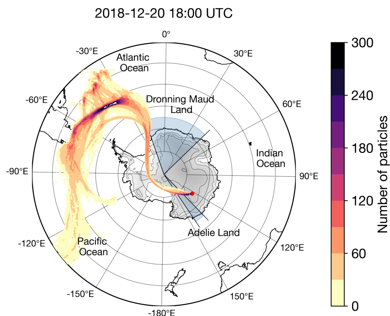
Figure 1. Total footprint, i.e. particles density partition during FLEXPART 10-days back-trajectories (Pisso et al., 2019) starting the 20th of December 2018 and released at a 1500 m altitude. The red dot indicates the location of the French-Italian Concordia station (123.4 °E, 75.1 °S, 3 233 m above sea level) at Dome C, on the East Antarctic Plateau. The light blue pie charts correspond to the Dronning Maud Land and Adelie Land regions.
