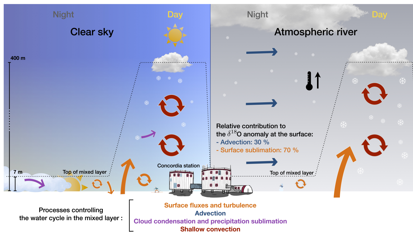
Figure 12. Summary of the processes controlling the modelled isotopic composition of surface vapour at Concordia during classical diurnal cycle (left) and during the AR (right). The processes of surface fluxes and turbulent mixing are shown in orange, cloud condensation and precipitation sublimation is shown in purple, shallow convection is shown in red and advection is in blue.
