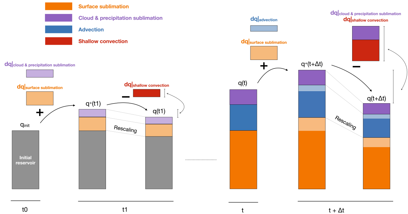
Figure 2. Schematic representation of the methodology used to determine the origin of atmospheric water sources. Each bucket corresponds to a specific water source and is represented by a distinct colour: the initial bucket, consisting of the water already present in the atmosphere, is shown in grey; the orange bucket corresponds to water originating from surface snow through surface sublimation; the blue bucket represents water transported by atmospheric dynamics (advection); and the purple bucket accounts for water from cloud and precipitation sublimation. In this example, shallow convection, represented in red, does not correspond to a bucket, as it only removes water from the atmosphere. Paler colours indicate newly added water contributions.
