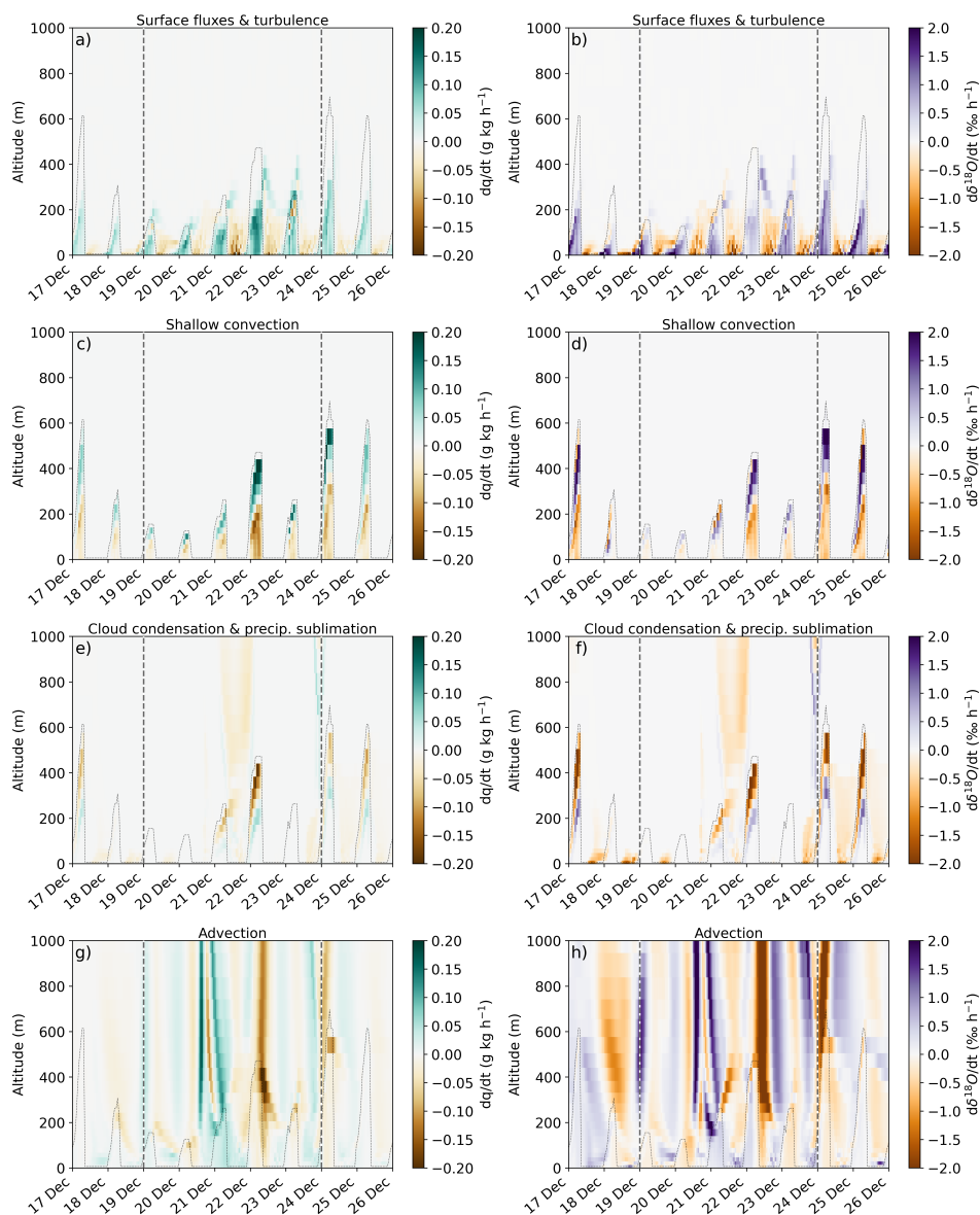
Figure 9. Decomposition of the rate of change of the different processes controlling specific humidity (left column: a, c, e, g) and vapour \delta^{18}\text{O} (right column: b, d, f, h) as a function of time at Concordia station. a) and b) correspond to surface sublimation and turbulent mixing, c) and d) to shallow convection, e) and f) to cloud condensation and precipitation sublimation and g) and h) to advection. It should be noted that the sign of changes is relative to water vapour so the surface sublimation is positive (increase in water vapour) and the cloud condensation is negative (decrease in water vapour). The dotted lines indicate the height of the mixed layer during shallow convection. The dashed vertical lines delineate the boundaries of the atmospheric river. All times are given in UTC; local time at Concordia is UTC+8, with maximum and minimum solar insolation occurring at 3 am and 3 pm local time, respectively.
