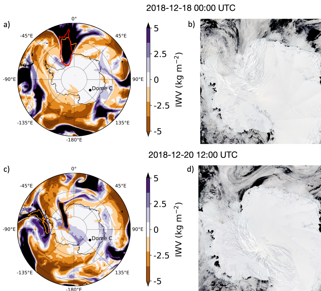
Figure 6. Atmospheric river on (a, b) 18 December 2018 at 00:00 UTC, before the AR crossed the Antarctic Plateau, and (c, d) 20 December 2018 at 12:00 UTC, after the AR had reached Dome C. (a, c) Shape of the detected AR, with anomalies in integrated water vapour transport (IWV) relative to the December climatology (1980-2021) shown in shading. Red and orange contours correspond to ARs detected using the vIVT and IWV based detection methods, respectively. (b, d) MODIS satellite imagery illustrating the progression of the AR across the Antarctic Plateau. Satellite images were obtained from the NASA MODIS instrument via the NASA Worldview application ( https://worldview.earthdata.nasa.gov ).
