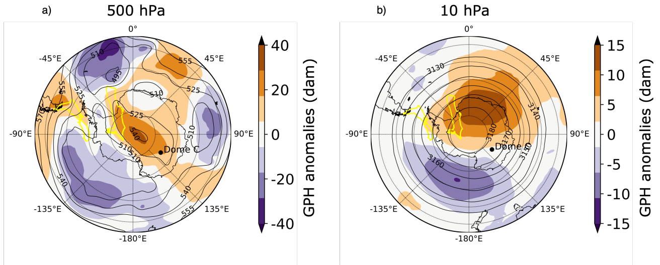
Figure S5. MERRA-2 geopotential height anomalies for 2018-12-20 12:00 UTC at a) 500 hPa and b) 10 hPa. Monthly anomalies are with respect to the corresponding 1980-2018 monthly mean. The yellow outlines corresponds with the atmospheric rivers detected using the IWV AR detection scheme.
