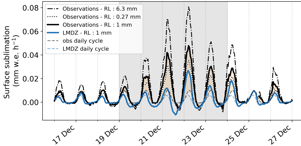
Figure S2. Water vapour flux at Dome C during December 2018 (positive for sublimation, negative for condensation) from observations (black lines) and model simulations (blue line). The solid black line corresponds to the reference configuration, using the H88 stability function with a roughness length z_0 = 1 mm (default value in LMDZ). The black broken lines show sensitivity tests with z_0 = 0.27 mm (dotted line) and z_0 = 6.3 mm (dashdot line). The grey rectangle indicates the period of the AR. The grey and blue dashed lines represent the mean diurnal cycle calculated over the entire month of December 2018 excluding the event (December 19-23), for observations and the model, respectively. The orange shading indicates the difference between the mean clear-sky diurnal cycle and the observations during the event.
