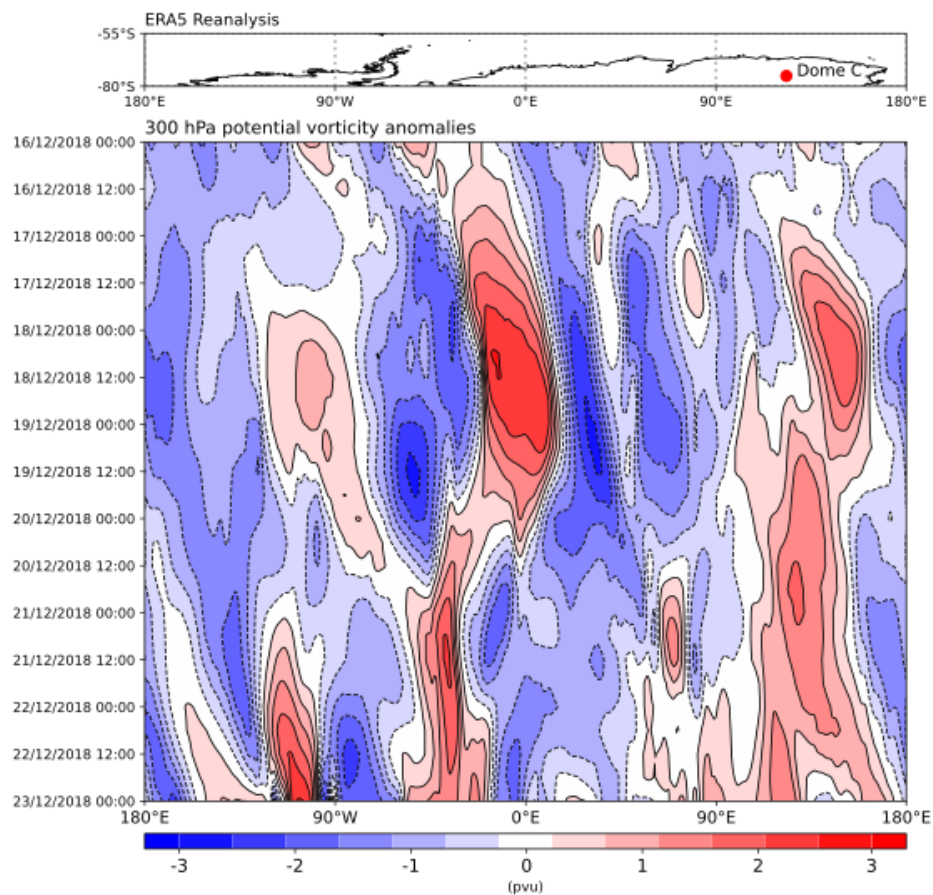
Figure S6. Hovmoller diagram showing 300 hPa potential vorticity anomalies from 2018-12-16 00:00 UTC - 2018-12-23 00:00 UTC with values averaged between 55 ° - 80 °S. Monthly anomalies are with respect to the corresponding 1980-2020 monthly mean.
