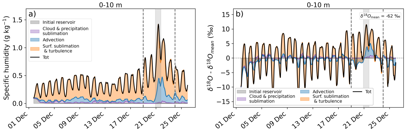
Figure S9. (a) Temporal evolution of the positive contributions of different processes to the surface specific humidity (6.7 m AGL) during December 2018. (b) Anomaly of the positive contributions of different processes to the surface \delta^{18}\text{O} signal relative to the mean \delta^{18}\text{O} during the diurnal cycle during December 2018 ( \delta^{18}\text{O}_{\text{mean}} = -62 \text{ ‰} ). The black line represents the signal obtained from total specific humidity and \delta^{18}\text{O} . Individual contributions to specific humidity and \delta^{18}\text{O} are shown in colour: orange for surface sublimation and vertical turbulent diffusion, blue for advection, and purple for cloud and precipitation sublimation. Vertical dashed lines mark the AR period (December 19-23), while the shaded area highlights the peak of the event, reached on December 21 at 09:30 UTC.
