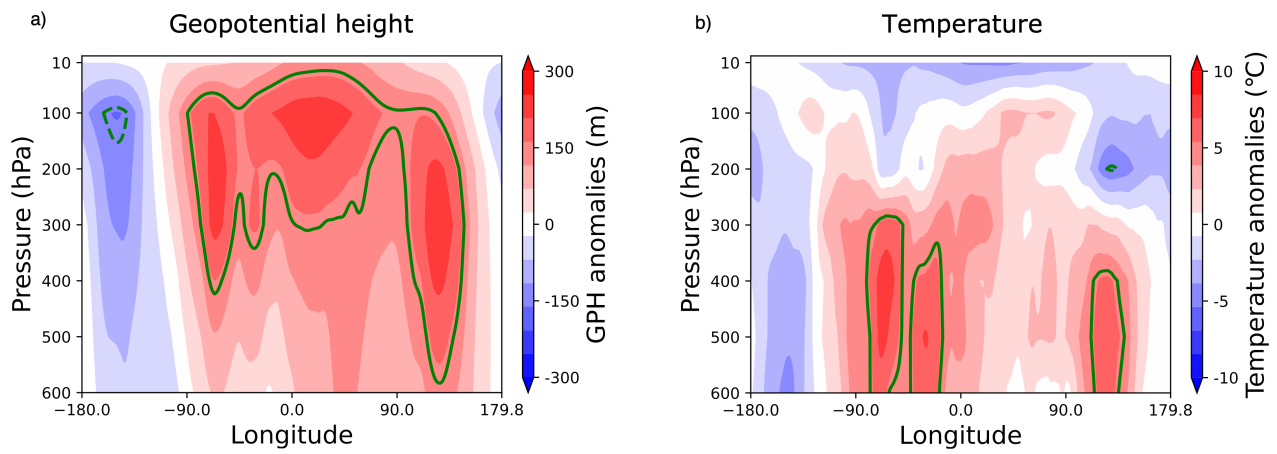
Figure S7. MERRA-2 a) geopotential height and b) temperature anomalies over the Antarctic continent from 10 - 600 hPa averaged between 55 ° - 90 °S. Solid green lines denote anomalies exceeding a) 150 m and b) 5 °C. Monthly anomalies are with respect to the corresponding 1980-2018 monthly mean.
