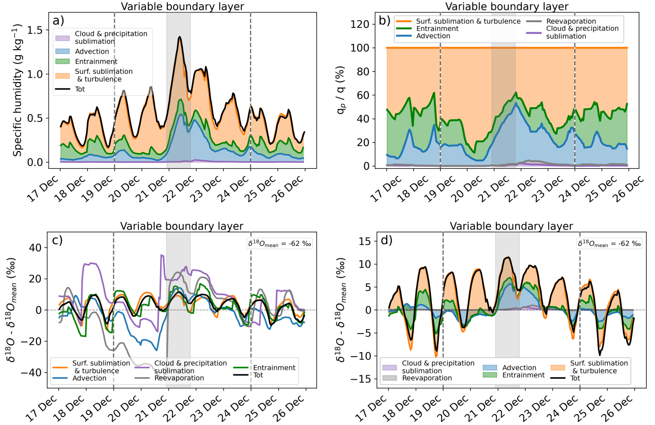
Figure S11. Temporal evolution of the positive contributions of different processes to the specific humidity in the mixed layer (a) and their respective percentages (b). Evolution of the \delta^{18}\text{O} anomaly relative to the mean clear-sky diurnal cycle value ( \delta^{18}\text{O}_{\text{mean}} = -62 ‰), associated with different processes (c). Positive contributions of different processes to the surface \delta^{18}\text{O} anomaly relative to this mean diurnal value (d). The black line represents the signal obtained from the model output, while the dashed line represents the sum of the different model processes. Individual contributions to specific humidity and \delta^{18}\text{O} are shown in colour: orange for vertical turbulent diffusion and surface sublimation, blue for advection, and purple for cloud condensation and precipitation sublimation. Vertical dashed lines mark the AR period (December 19-23), while the shaded area highlights the peak of the event, reached on December 21 at 09:30 UTC.
