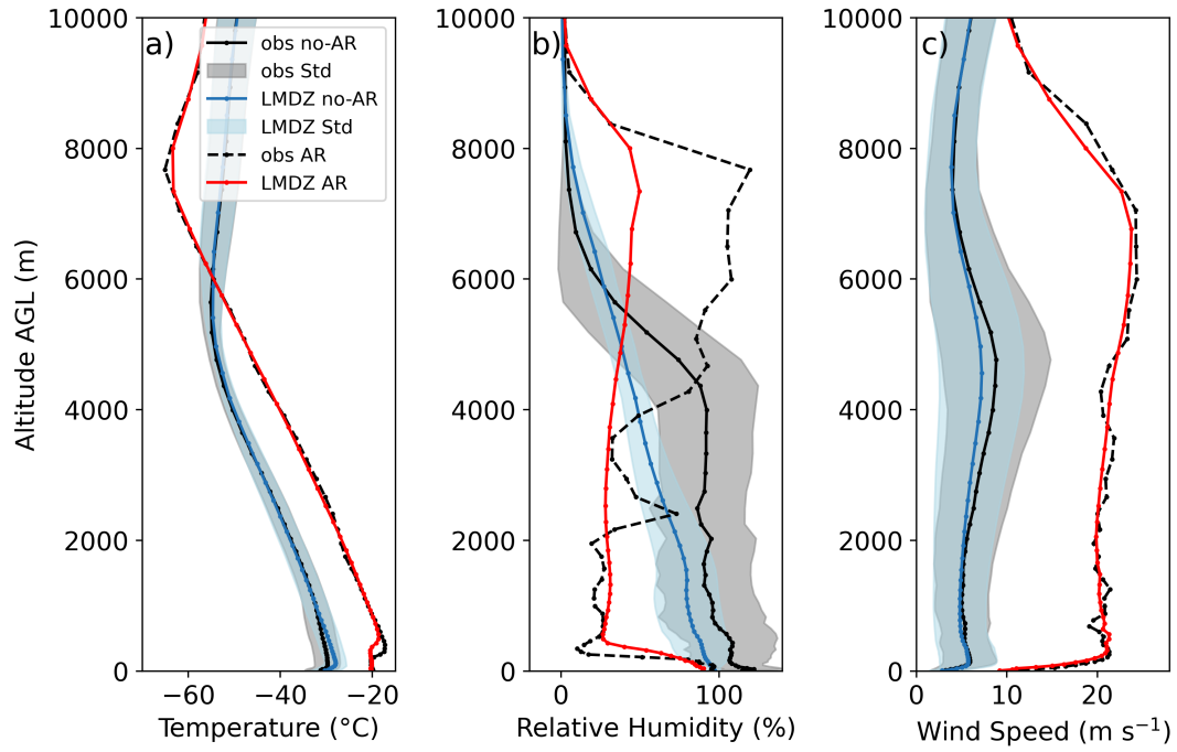
Figure S4. Vertical profiles of (a) temperature ( ^{\circ}\text{C} ), (b) relative humidity with respect to ice (%) and (c) wind speed ( \text{m s}^{-1} ) from the surface to 10000 m AGL, based on average radiosonde measurements at the Concordia station during December 2018 (twice per day, black solid lines) and during the AR event (22 December 2018 at 11:00 UTC, black dashed lines). Corresponding LMDZ model output at the nearest grid point for the same times are shown in blue lines (December averages) and red lines (AR event). The standard deviation is shown in gray for observations and in blue for LMDZ for 52 radiosondes during December 2018 outside the AR event.
