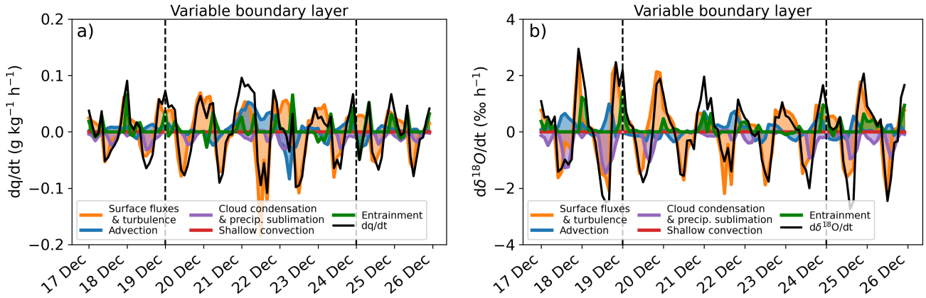
Figure S10. Rate of temporal change of the different processes contributing to the (a) specific humidity tendency (g kg -1 h -1 ) and (b) vapour \delta^{18}\text{O} tendency (‰ h -1 ) in the mixed layer at Concordia station. The black line represents the signal obtained from the model output, while the dashed line represents the sum of the different model processes. The individual contributions to the rate of change of humidity and \delta^{18}\text{O} are shown in colour: orange for vertical turbulent diffusion and surface sublimation, blue for advection, purple for cloud condensation and precipitation sublimation, red for shallow convection and green for mixing. It should be noted that the sign of changes is relative to water vapour so the surface sublimation is positive (increase in water vapour) and the cloud condensation is negative (decrease in water vapour).
