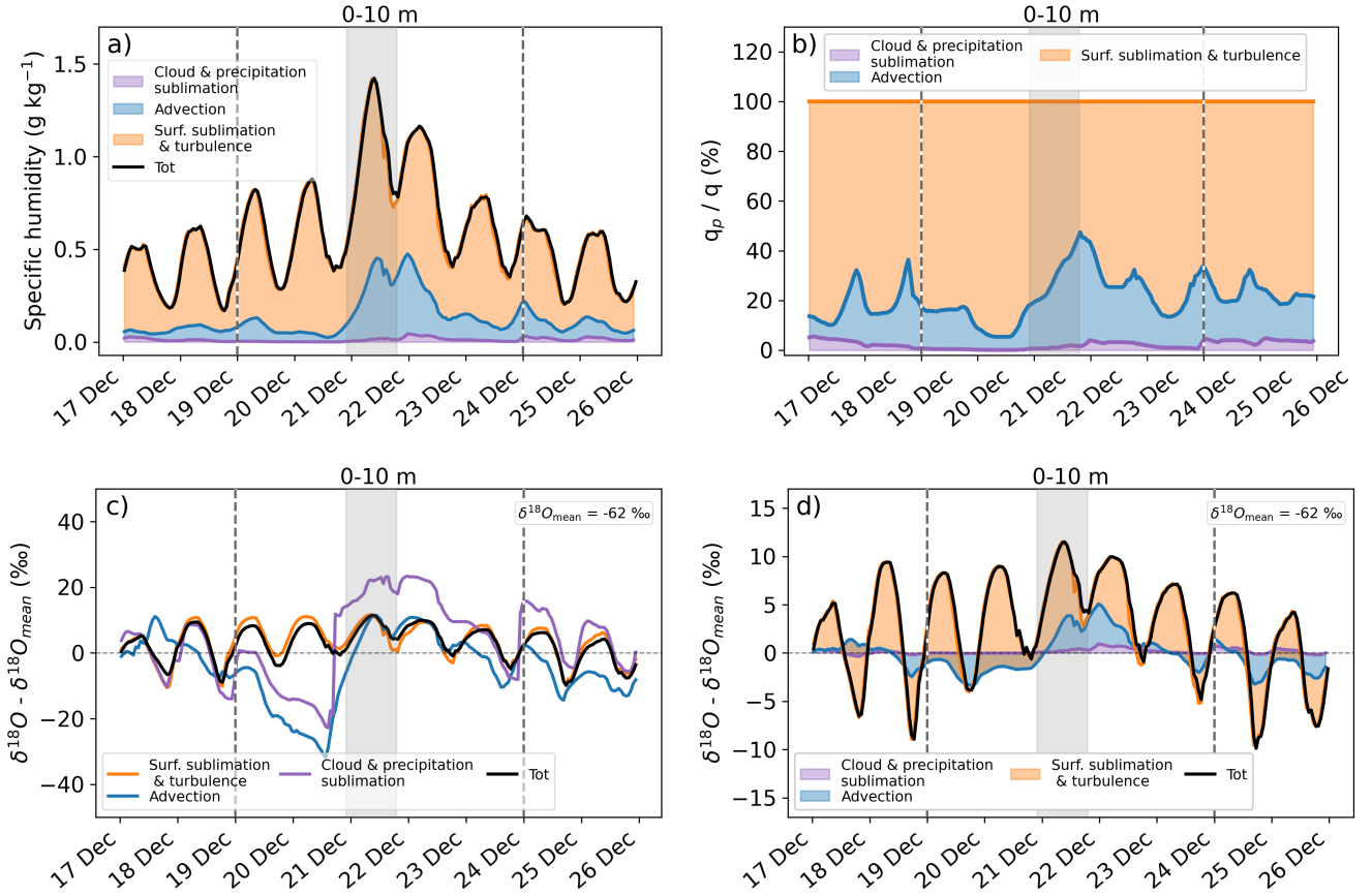
Figure 11. (a) Temporal evolution of the positive contributions of different processes to the surface specific humidity (6.7 m AGL) and (ab) and their respective percentages. (bc) Evolution of the \delta^{18}\text{O} anomaly relative to the mean clear-sky diurnal cycle value ( \delta^{18}\text{O}_{\text{mean}} = -62\text{‰} ), associated with different processes. (ed) Positive contributions of different processes to the surface \delta^{18}\text{O} anomaly relative to this mean diurnal value (d). The black line represents the signal obtained from total specific humidity and \delta^{18}\text{O} . Individual contributions to specific humidity and \delta^{18}\text{O} are shown in colour: orange for surface sublimation and vertical turbulent diffusion, blue for advection, and purple for cloud and precipitation sublimation. Vertical dashed lines mark the AR period (December 19-23), while the shaded area highlights the peak of the event, reached on December 21 at 09:30 UTC.
