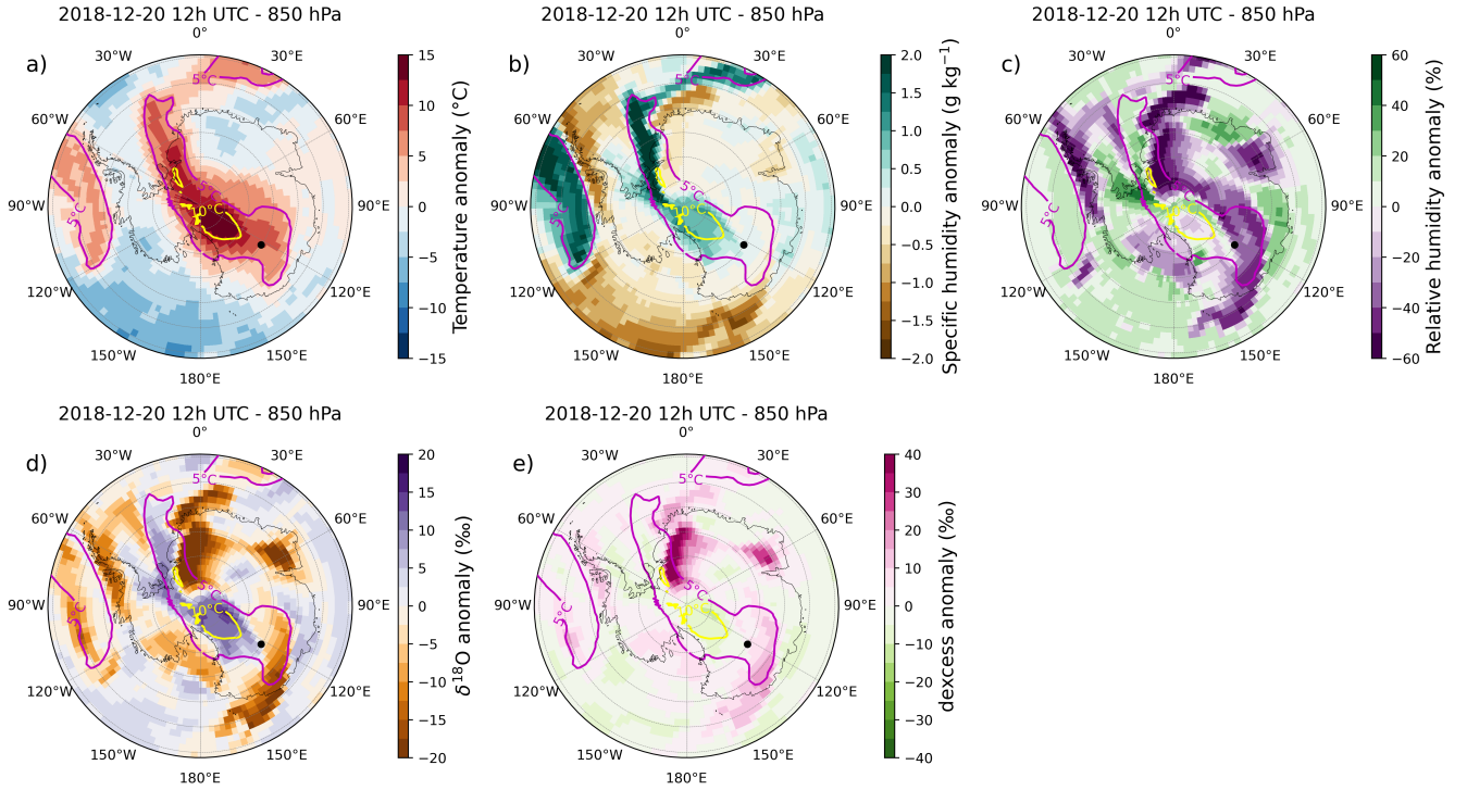
Figure 4. LMDZ6iso anomalies at the model level equivalent to 850 hPa above sea level of (a) temperature (°C), (b) specific humidity (g kg -1 ), (c) relative humidity (%), (d) \delta^{18}\text{O} (‰), and (e) d-excess (‰), calculated on December 20, 2018 at 12:00 UTC relative to the December average (1980–2021). The purple contour represents the 5 °C anomaly boundary, while the yellow contour indicates the 10 °C anomaly boundary. The black dot indicates Concordia station. The altitude above the surface corresponding to the LMDZ6iso model level equivalent to 850 hPa is shown in Fig. S5 (around 1000 m AGL over the ice sheet).
