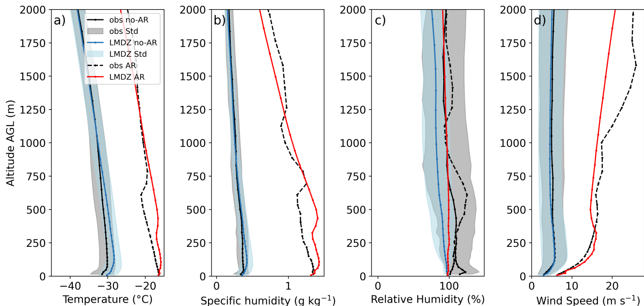
Figure 7. Vertical profiles of (a) temperature ( ^{\circ}\text{C} ), (b) specific humidity ( \text{g kg}^{-1} ) , (c) relative humidity with respect to ice (%) and (d) wind speed ( \text{m s}^{-1} ) from the surface to 2000 m AGL, based on average radiosonde measurements at the Concordia station during December 2018 excluding the event (December 19-23) (twice per day, black solid lines) and during the AR event ( 22-21 December 2018 at 11:00 UTC, black dashed lines). Corresponding LMDZ-LMDZ6iso model output at the nearest grid point for the same times are shown in blue lines (December averages) and red lines (AR event). The standard deviation is shown in gray for observations and in blue for LMDZ-LMDZ6iso for 52 radiosondes during December 2018 outside the AR event.
