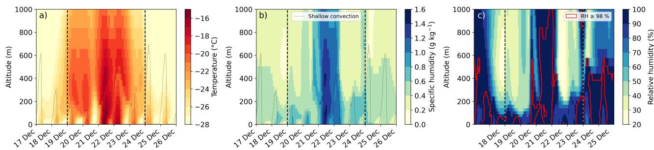
Figure 8. Modelled vertical profiles of (a) temperature ( ^{\circ}\text{C} ), (b) specific humidity ( \text{g kg}^{-1} ), and (c) relative humidity with respect to ice (%) at Concordia. The red outline indicates regions where the relative humidity is higher than 98 %. The dotted lines indicate the height of the mixed layer during shallow convection. The dashed vertical lines delineate the boundaries of the atmospheric river. All times are given in UTC; local time at Concordia is UTC+8, with maximum and minimum solar insolation occurring at 3 am and 3 pm local time, respectively.
