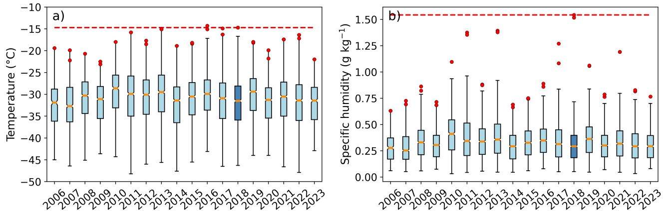
Figure 5. Hourly temperatures (a) and specific humidity (b) recorded at Dome C during summers (December-January) from December 2006 to January 2019-2024 from the AWS. The year of interest, 2018 (December 2018 - January 2019), is coloured in dark blue. Each box is delimited by the 0.25 and 0.75 percentiles and the orange bar represents the median. Black bars indicate the values outside inside 1.5 times the inter-quartile range. Red circles indicate values outside the 0.99-0.999 percentiles. The dotted red line indicate the value reached during the December 2018 AR.
