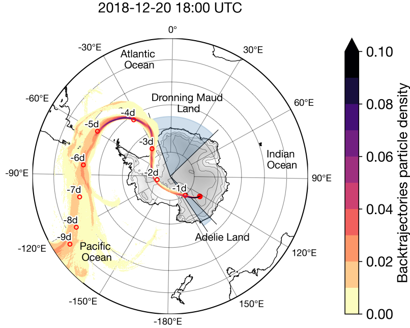
Figure 1. Total FLEXPART 10-days backtrajectory analysis showing particles total footprint, i.e. particles the density partition during FLEXPART 10-days back-trajectories (Pisso et al., 2019) starting the 20th of December 2018 and particles released at a 1500 m altitude. The red dot indicates the location of the French-Italian from Concordia station (red dot, 123.4 °E, 75.1 °S, 3 233 m above sea level) the 20th of December 2018 18:00 at a 1000 m above ground level. The French-Italian Concordia station is located at Dome C on the East Antarctic Plateau. The red circles and the “-xd” labels indicate the mean position of the particles during the x-th day preceding 20 December 2018. The light blue pie charts correspond to the Dronning Maud Land and Adelie Land regions. Units represent the density of particles in the atmospheric column launched from Concordia standardized by the total number of particles.
