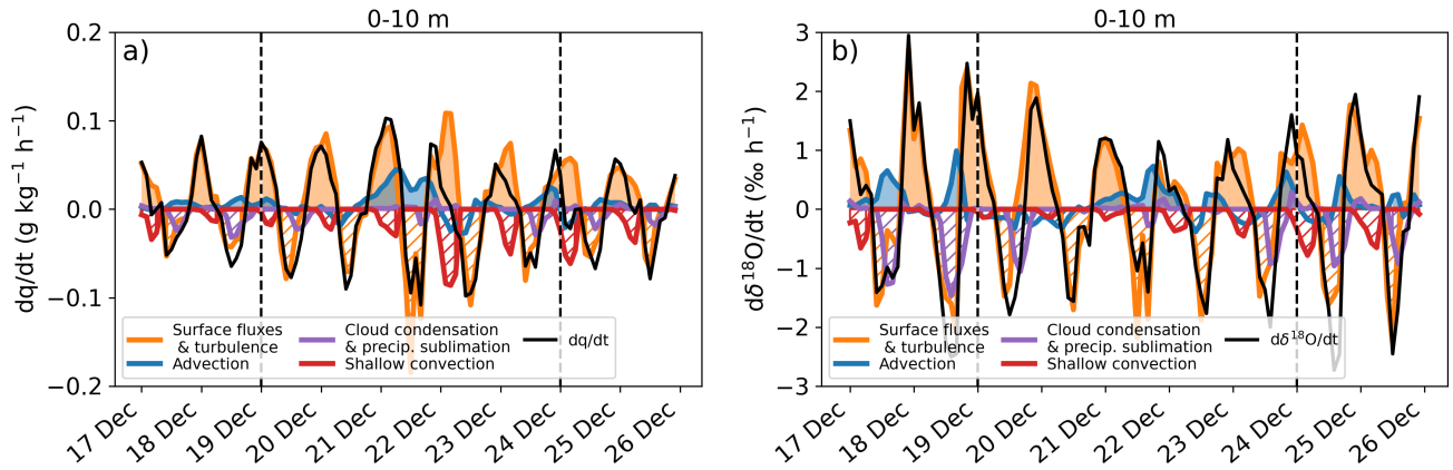
Figure 10. Rate of temporal change of in the different surface atmospheric layer due to the different processes contributing to the (a) specific humidity tendency ( \text{g kg}^{-1} \text{h}^{-1} ) and (b) vapour \delta^{18}\text{O} tendency ( \text{‰ h}^{-1} ) at Concordia station. The black line represents the signal obtained from the first level model output, while the dashed line represents the sum of the different model processes. The individual contributions to the rate of change of humidity and \delta^{18}\text{O} are shown in colour: orange for vertical turbulent diffusion and surface sublimation fluxes, blue for advection, purple for cloud condensation and precipitation sublimation and red for shallow convection. Processes with positive contributions are shown in solid colours, whereas processes with negative contributions are shown using hatched shading. It should be noted that the sign of changes is relative to water vapour so the surface sublimation is positive (increase in water vapour) and the cloud condensation is negative (decrease in water vapour). The dashed vertical lines delineate the boundaries of the atmospheric river.
