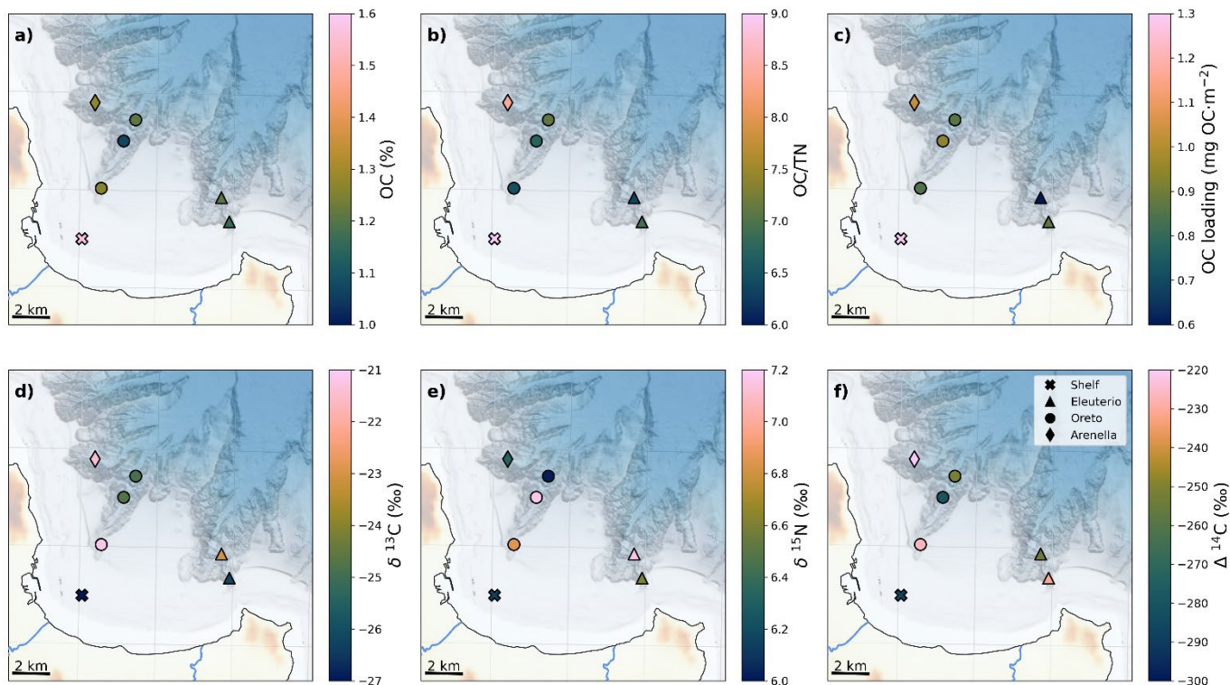
Figure 2. Spatial distribution of bulk parameters: a) OC, b) OC/TN, c) OC loading, d) δ 13 C, e) δ 15 N, f) Δ 14 C. Colour bars are adjusted to highlight the minimum, mean, and maximum values for each variable.
