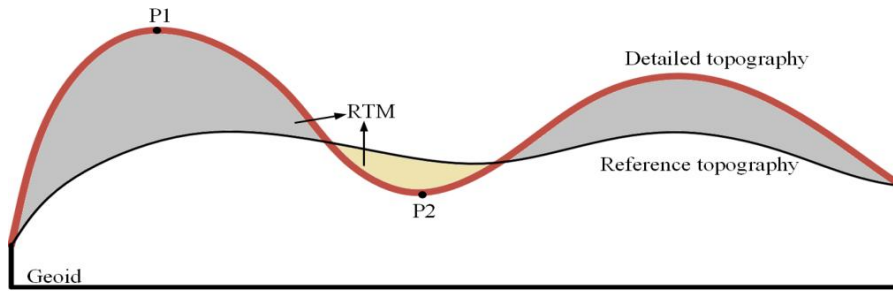
160 Figure 3: Schematic diagram of the RTM.
