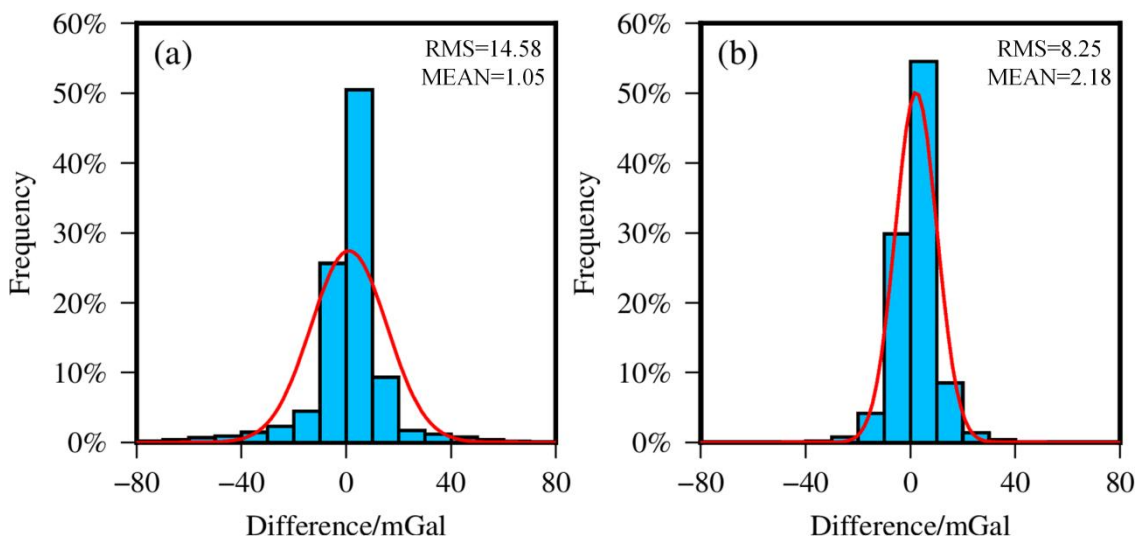
Figure 11: Histogram of the differences between the measured GA and XGM-GA (a), and the differences between the measured GA and XGM/RTM-GA (b).
