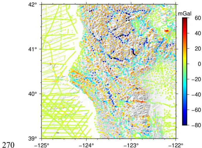
Figure 9: RTM-GA values at the measured points.
