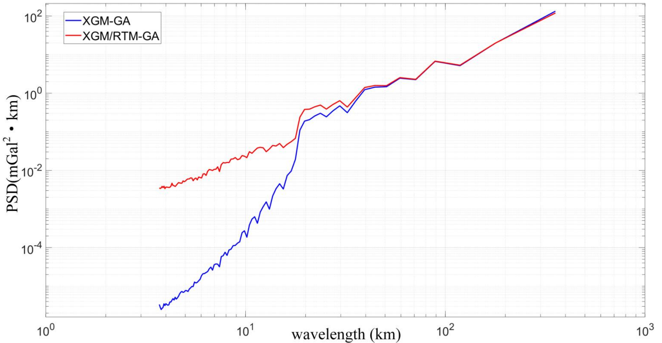
Figure 12: PSD of the XGM-GA and XGM/RTM-GA models.
