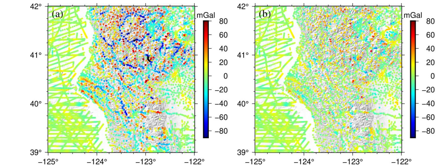
Figure 10: The difference between the measured GA and XGM-GA (a), and the difference between the measured GA and XGM/RTM-GA (b).
