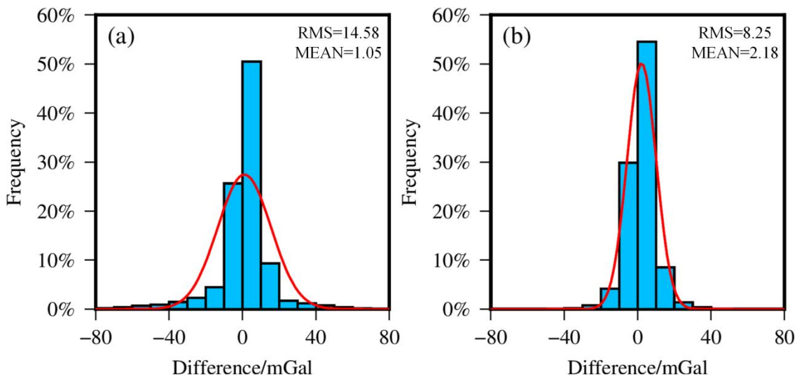
315 Figure 11: Histogram of the differences between the measured GA and XGM-GA (a), and the differences between the measured GA and XGM/RTM-GA (b).
