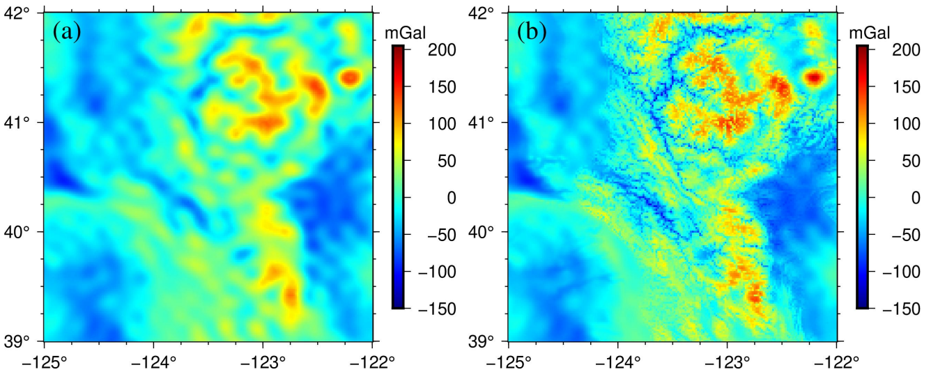
Figure 8: XGM-GA model (a) and XGM/RTM-GA model (b).
