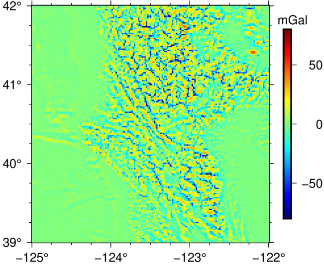
260 Figure 7: RTM-GA model.
