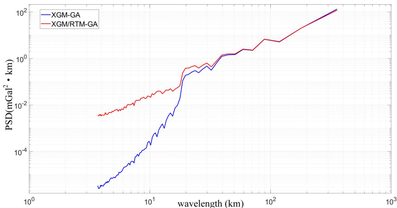
355 Figure 12: PSD of the XGM-GA and XGM/RTM-GA models.
