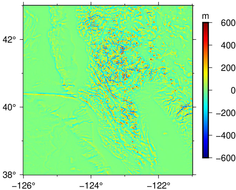
Figure 4 RTM of the study area.
