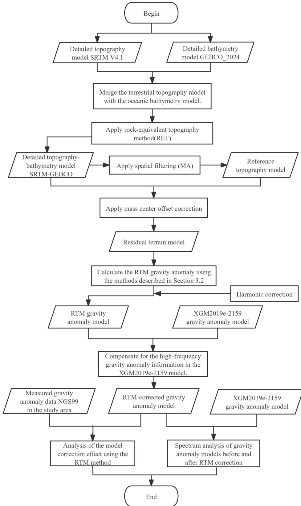
Figure 6: Workflow of XGM-GA model refinement based on RTM.
