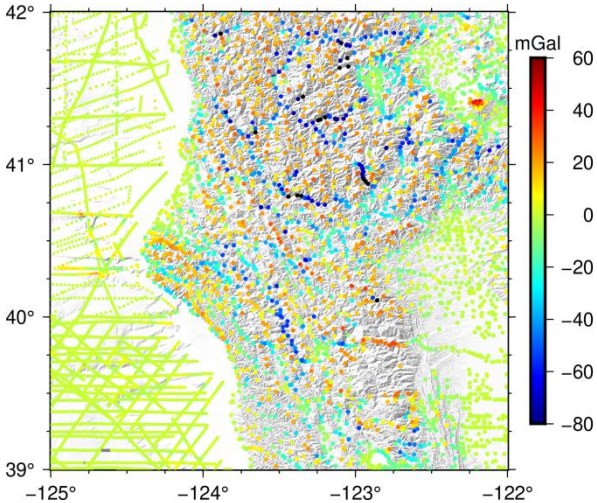
Figure 9: RTM-GA values at the measured points.
