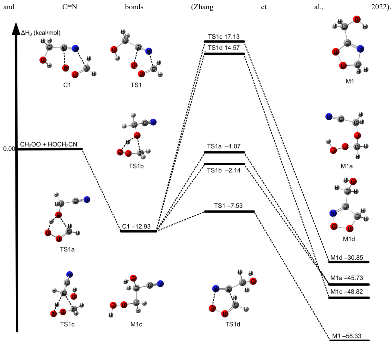
Figure 1: The relative enthalpies at 0 K for the reaction of \text{CH}_2\text{OO} + \text{HOCH}_2\text{CN} . Values are given for all species as calculated by M11-L/MG3S.
