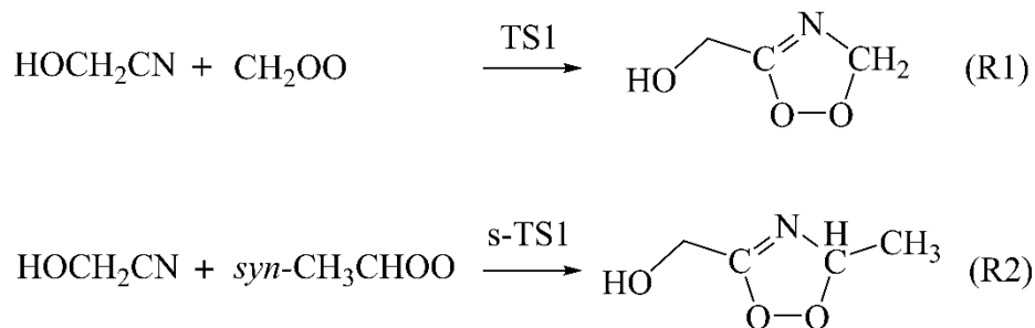
Scheme 1. The reaction route for \text{CH}_2\text{OO}/\textit{syn}\text{-CH}_3\text{CHOO} + \text{HOCH}_2\text{CN}
