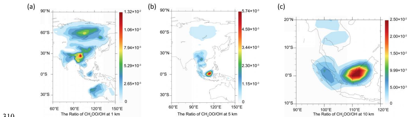
Figure 4: The ratio of \text{CH}_2\text{OO} to OH at night from literature.(Long et al., 2024) (a) at 1 km, (b) at 5 km, (c) at 10 km, (d)at 15 km.
