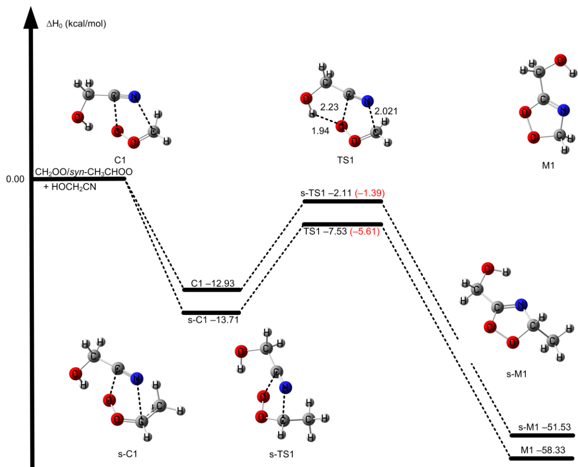
195 Figure 2: The relative enthalpies at 0 K for the reaction of \text{CH}_2\text{OO}/\text{syn-CH}_3\text{CHOO} + \text{HOCH}_2\text{CN} for R1 and R2. Values are given for all species as calculated by M11-L/MG3S, and in small parentheses and brackets, values are given for the transition state TS path as calculated by W3X-L//DF-CCSD(T)-F12b/jun-cc-pVDZ. The bond length in TS1 is in units of Å.
