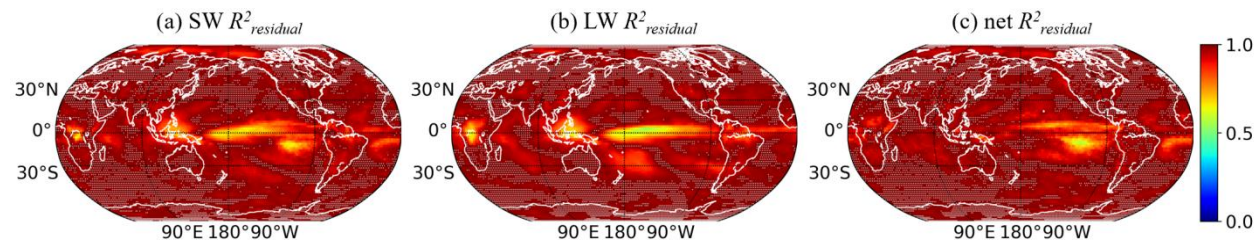
Figure S4: Maps of residual R^2 for results in Fig. 3 in the main text. (a) CRE_{SW} , (b) CRE_{LW} , and (c) CRE_{net} . White dots denote grids with statistically insignificant partial regression coefficients of both time and ONI (i.e., a and b in Eq. 1) at the 95% confidence level.
