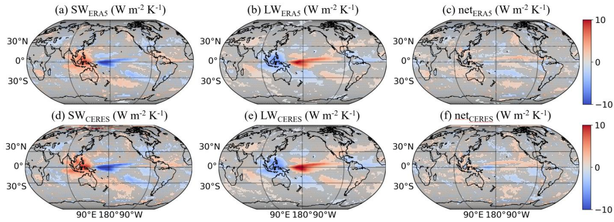
Figure S5: ENSO contribution to cloud feedback estimates for CRE_{SW} (left column), CRE_{LW} (middle column), and CRE_{net} (right column), derived from ERA5 data and CERES measurements (January 2002–December 2021). (a–c) Maps based on ERA5 data. (d–f) Maps based on CERES measurements. Black dots denote grids with statistically insignificant partial regression coefficient of ONI (i.e., b in Eq. 1) in either the GMST or CRE model at the 95% confidence level.
