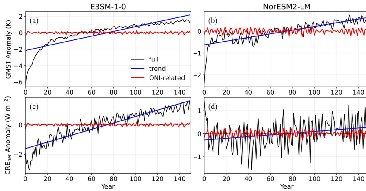
Figure S9: Decomposition of GMST and global-mean CRE net , derived from two GCM simulations of the abrupt-4×CO 2 experiment (first 150 years). (a–b) GMST for (a) E3SM-1-0 and (b) NorESM2-LM. (c–d) Global-mean CRE net for (c) E3SM-1-0 and (d) NorESM2-LM. The blue and red lines represent the trend- and ONI-related components, respectively.
