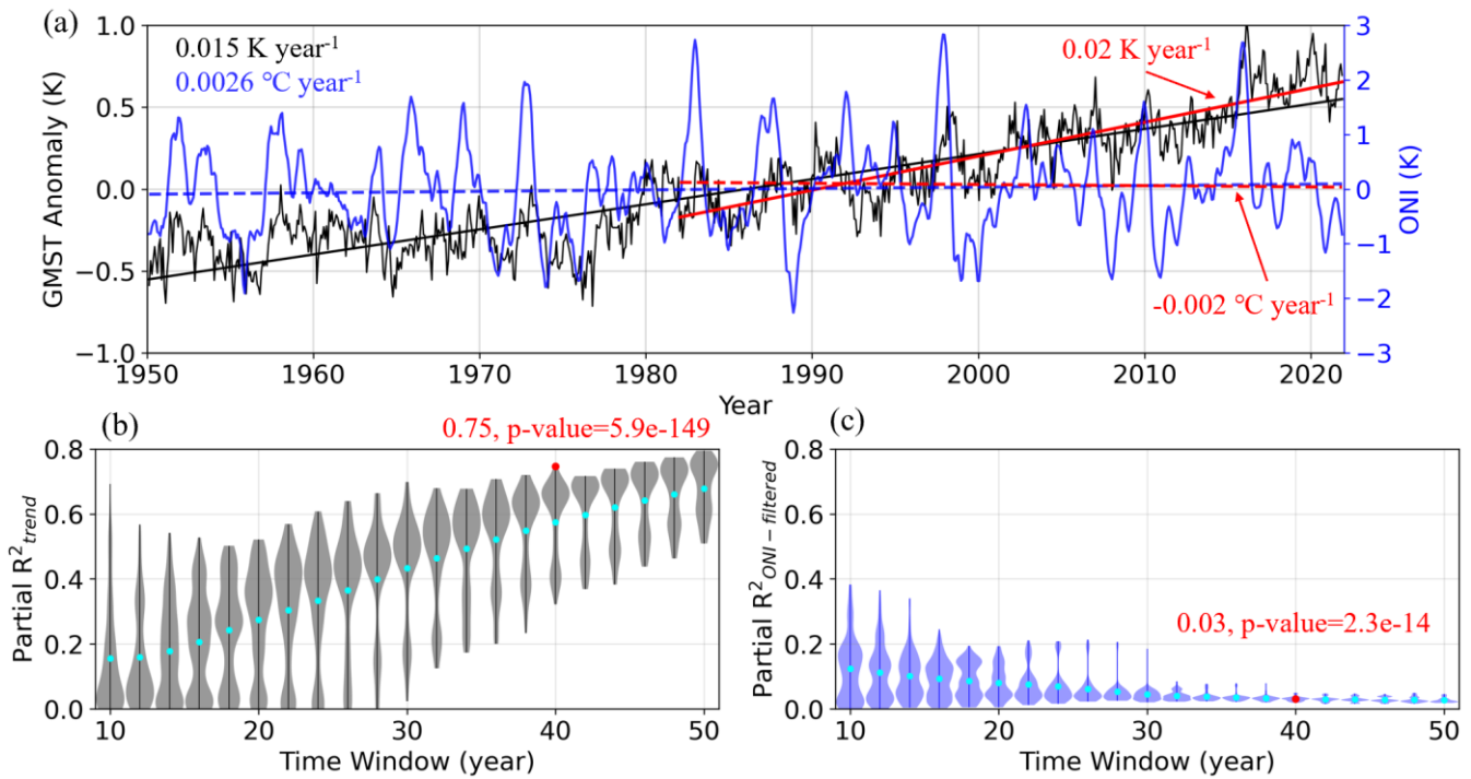
Figure 2: Analysis of the GMST variations driven by the temporal trend and ENSO, derived from ERA5 data (during January 1950–December 2021). (a) Time series of GMST anomaly (black curve; left y-axis) and ONI (blue curve; right y-axis). The black and blue lines and number represent the corresponding OLS regression fits, with the values indicating their slope and slope, respectively. (b–c) Violin plots of (b) partial R^2_{trend} and (c) partial R^2_{ONI-filtered} for GMST, shown as a function of the time window (2-year intervals in intervals of 2 years). Per-For each time window, the vertical line indicates the range (minimum to maximum), the shaded area represents the probability density, and the cyan dot denotes the mean value. The red lines, dots and numbers highlight the results for the selected representative 40-year subset (January 1982–December 2021) that is analyzed in Figs. 3–4. In panel (a), solid and dashed lines represent the statistically significant and insignificant trends at the 95% confidence level, respectively.
