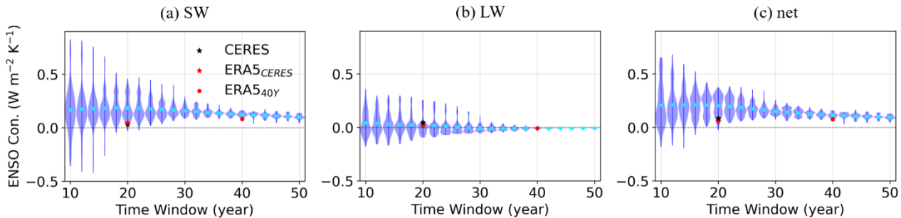
280 Figure 6: Violin plots of the ENSO contribution to global-mean CREs, derived from ERA5 data (during January 1950–December 2021). (a) CRE SW , (b) CRE LW , and (c) CRE net . The black star, red star, and red dot denote the results from CERES measurements, ERA5 data during the CERES period, and ERA5 data during the representative example 40-year period, respectively.
