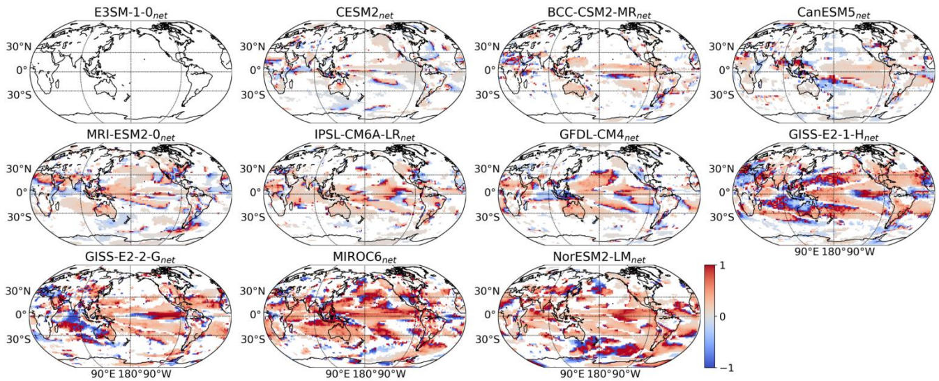
310 Figure 8: Maps of the relative ENSO contribution to CRE_{net} derived from GCM simulations from of the abrupt- 4\times CO_2 experiment during the (first 150 years) . The name of the corresponding model name is indicated in each panel. Grids with statistically insignificant partial regression coefficient of ONI (i.e., b in Eq. 1) for either GMST or CRE at the 95% confidence level are masked in white.
