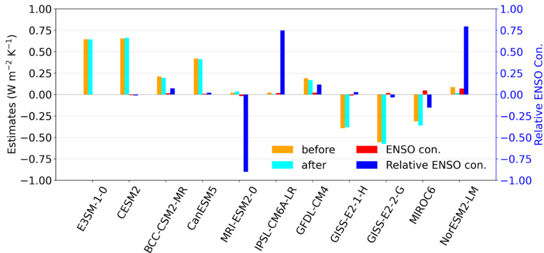
Figure 9: Bar charts of the ENSO contribution to global-mean CRE_{net} derived from GCM simulations from-of the abrupt- 4\times CO_2 experiment during the (first 150 years). The orange and cyan bars indicate global-mean cloud feedback estimates before and after the ENSO correction, respectively. The red and blue bars indicate the ENSO contribution (orange minus cyan bars). The blue bars indicate and relative ENSO contribution (red divided by orange bars; right y-axis), respectively . Note that a large relative value (blue bar) can arise when the original feedback estimate (orange bar) is small.
