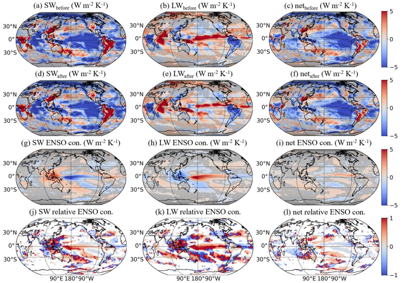
230 Figure 4: A sample analysis of the ENSO contribution to cloud feedback estimates for CRE_{SW} (left column), CRE_{LW} (middle column), and CRE_{net} (right column), derived from ERA5 data (during January 1982–December 2021). (a–c) Cloud feedback estimates before ENSO correction. (d–f) Cloud feedback estimates after ENSO correction. (g–i) ENSO contribution (a–c minus d–f). (j–l) Relative ENSO contribution (g–i divided by a–c). In panels (a–i), black dots denote grids with statistically insignificant partial regression coefficient of ONI (i.e., b in Eq. 1) for either GMST or respective CRE at the 95% confidence level. In panels (j–l), these insignificant grids are masked in white.
