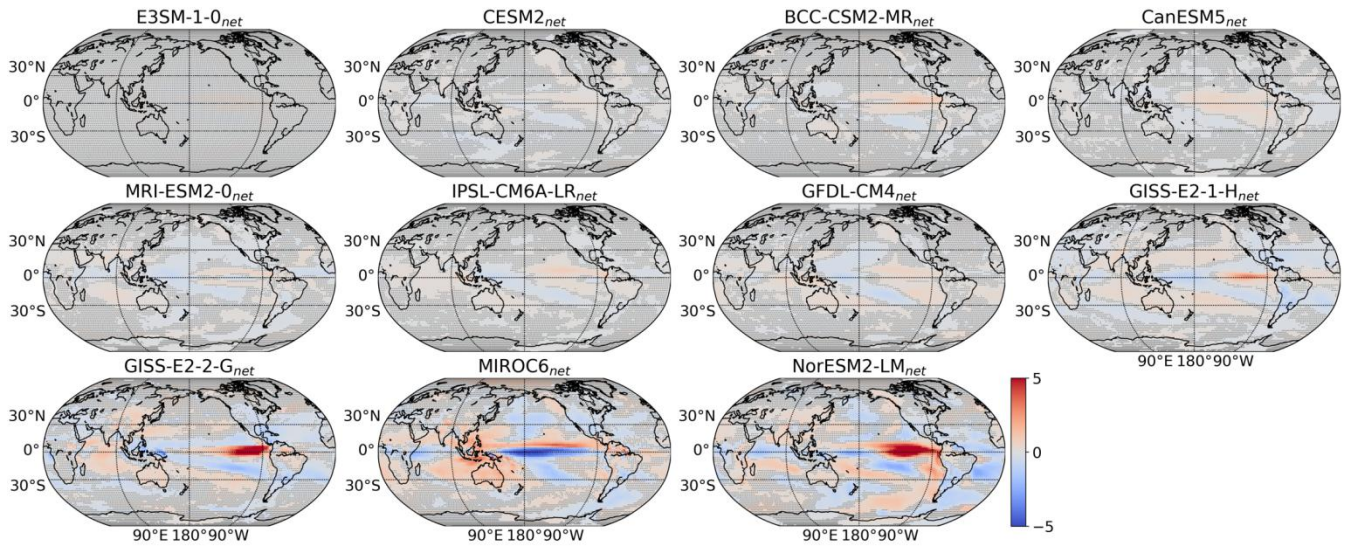
Figure 7: Maps of ENSO contribution to CRE_{net} , derived from GCM simulations from of the abrupt- 4\times CO_2 experiment during the (first 150 years) . The name of the corresponding model name is indicated in each panel. Black dots denote grids with statistically insignificant partial regression coefficient of ONI (i.e., b in Eq. 1) for either GMST or CRE at the 95% confidence level.
