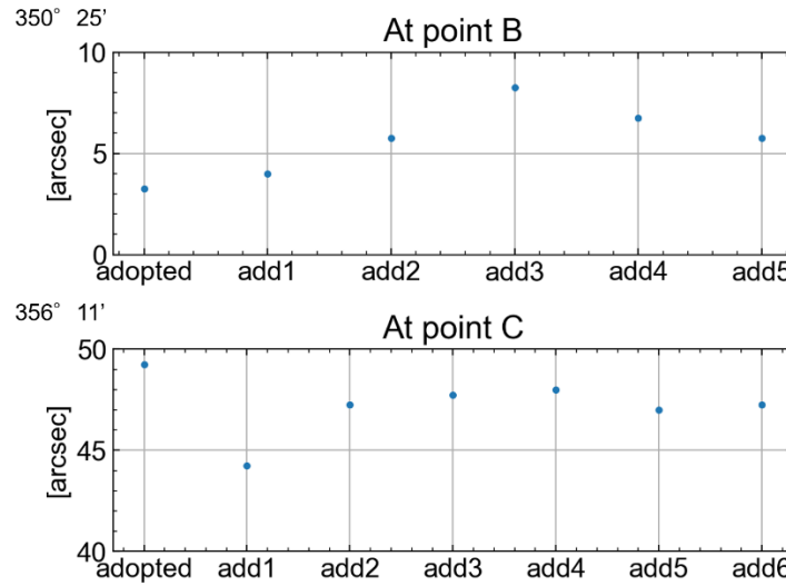
Figure 6: The adopted results of the horizontal angles, \beta_1 at point B and \beta_2 at point C, and \beta_z , and the results of additional observations.
