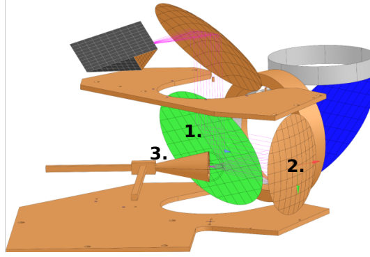
Figure 4. A GRASP model of the TEMPERA-C optics, showing the rotatable planar mirror (1), the focusing parabolic mirror (2), and the feed-horn (3).
