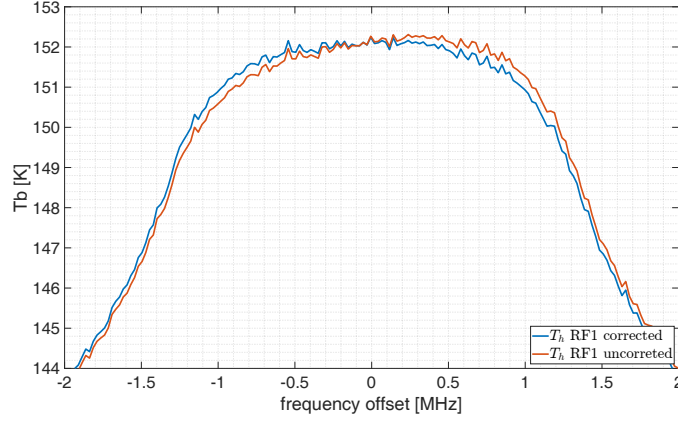
Figure 13. T_{sky,h} before and after the correction according (54) illustrated for the emission line with centered at 53.067 GHz. The uncorrected line spectrum shows an asymmetry around the line center, which is eliminated after applying the correction.
