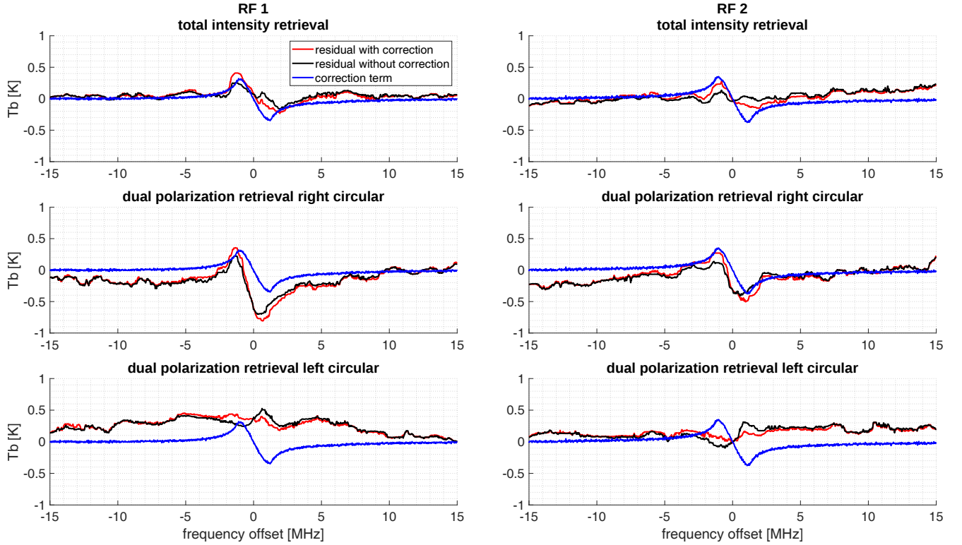
Figure B2. Forward model residuals from different retrieval algorithms calculated by \Delta y = y - y_f and smoothed with a moving window median, alongside the calibrated correction terms (Eq. (54)). The total intensity and dual-circular-polarization retrievals were executed once with cross-talk correction and once without the cross-talk correction. The dual-circular-polarization retrieval produces two residuals, one for the left-hand-circularly polarized spectrum and another for the right-hand-circularly polarized spectrum. RF 1 and RF 2 line centers are at 53.067 GHz and 53.596 GHz, respectively.
