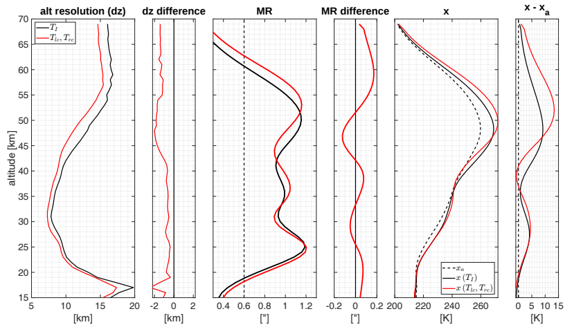
Figure 16. Same as Fig. 14 with measurements which were taken on March 25, 2024, at the Sphinx observatory.
