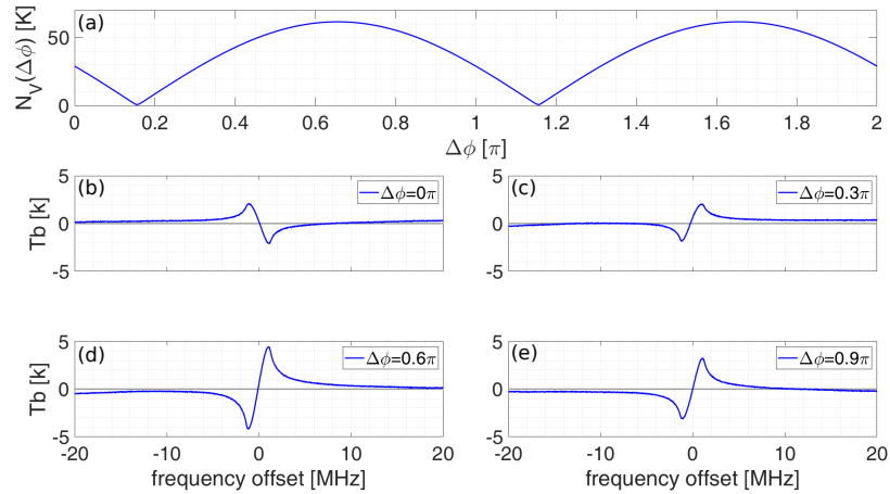
Figure 11. Panel (a) illustrates N_V as a function of \Delta\phi (Eq. (49)), while panels (b-e) show calibrated T_4^{\text{sky}} spectra (Eq. (52)) for various values of \Delta\phi . The mixing of U- and V-Stokes components varies with dependence on \Delta\phi .
