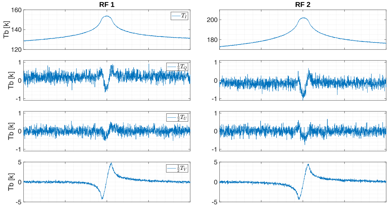
Figure B1. TEMPERA-C calibrated and corrected spectra in the representation [T_I, T_Q, T_U, T_V] measured at the Sphinx observatory. The measurement was taken on March 25, 2024, at night. The integration time is 30 min. RF 1 and RF 2 line centers are at 53.067 GHz and 53.596 GHz, respectively.
