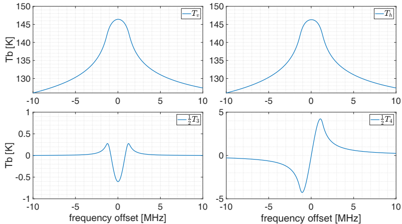
Figure 1. The four components of the modified Stokes vector, simulated for the Zeeman split emission line at 53.067 GHz. The viewing geometry used in the simulation matches that during the measurement campaign at the Sphinx observatory, which has a sensor altitude of 3571 m.a.s.l, a zenith angle of 30^\circ , and an azimuth angle 75^\circ . The fourth Stokes component is represented in a right-handed geometry and is sign-inverted compared to the simulation (Sec. 5.1), which uses left-hand geometry. Detailed descriptions of the remaining forward model parameters can be found in Sec. 5.2.
