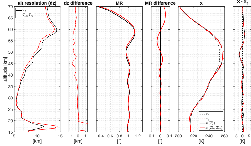
Figure 14. Results of the comparison with idealized conditions where the retrieval algorithm was tested with simulated spectra of total intensity T_I and dual-circularly-polarized states ( T_{lc}, T_{rc} ). The plot illustrates the vertical resolution (dz), measurement response (MR), forward model ( x_f ), a priori ( x_a ), and retrieved temperature profiles ( x ), along with the corresponding differences between the results for T_I and T_{lc}, T_{rc} .
