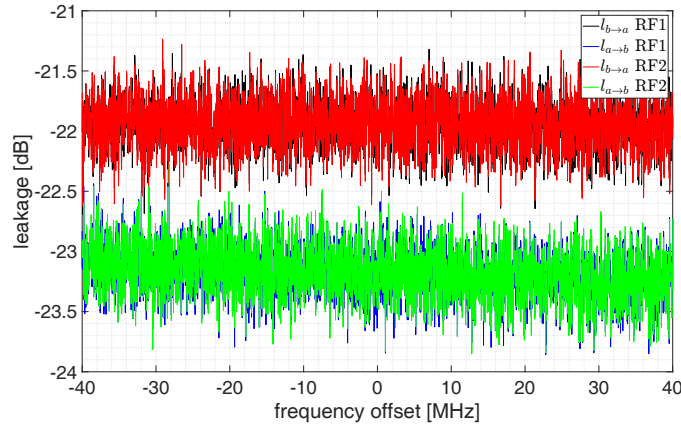
Figure 8. Upper limits of the leakage parameters (Eq. (26)). The RF 1 and RF 2 center frequencies are tuned to 53.07 GHz and 53.6 GHz, respectively. The subscripts a and b denote the two orthogonal polarized receiver chains.
