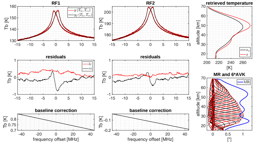
Figure 15. Overview of the retrieval result from spectra observed on March 25, 2024, at the Sphinx observatory. Line centers of the RF1 and RF2 spectra are at 53.067 GHz and 53.596 GHz, respectively. The residuals were calculated by \Delta y = y - y_f and smoothed with a moving window median. For illustrative purposes, every second row of the Averaging Kernel Matrix (AVK) was omitted in the figure, and the remaining rows were multiplied by a factor of 6 to match the Measurement Response (MR).
