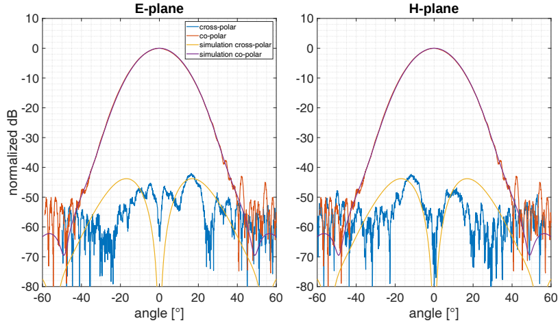
Figure 3. Measured and simulated co- and cross-polar antenna patterns for the feed-horn at 53 GHz were measured without the parabolic mirror. The E and the H plane are orthogonally polarized antenna planes. The cross-polar field introduces cross-talk between the polarization components. These measurements were performed using a linearly polarized receiver in the laboratory at the University of Bern.
