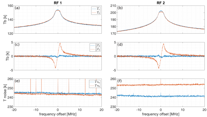
Figure 12. TEMPERA-C calibrated and corrected spectra in representation of the modified Stokes vector and instrument noise temperatures measured at the Sphinx observatory. These measurements were taken during nighttime on March 25, 2024, with an integration time of 30 minutes. Panels (a, c, e) display the spectra for the emission line centered at 53.067 GHz, with RF 1 frequency tuned to 53.07 GHz. Panels (b, d, f) show the spectra for the emission line centered at 53.596 GHz, with RF 2 frequency tuned to 53.6 GHz.
