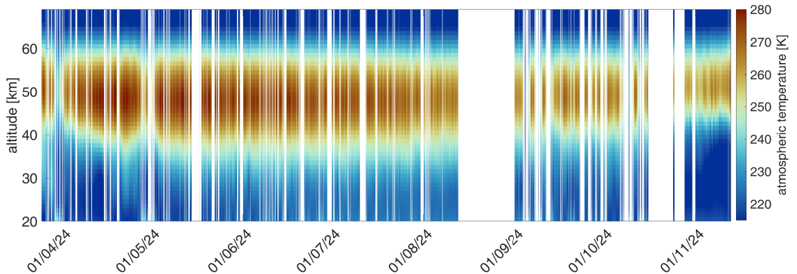
Figure 17. Series of the profiles of retrieved atmospheric temperature during the Jungfraujoch campaign. The dataset of retrieved temperature profiles shows dynamical features, such as thermal tides.
