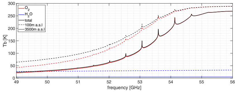
Figure 5. Left wing of the 60 GHz oxygen band, simulated for a ground-based sensor at a zenith angle of 30^\circ . Simulations were performed for two sensor altitudes: 100 m.a.s.l. and 3500 m.a.s.l. The influence of air humidity is illustrated by including the \text{H}_2\text{O} emission in the figure.
