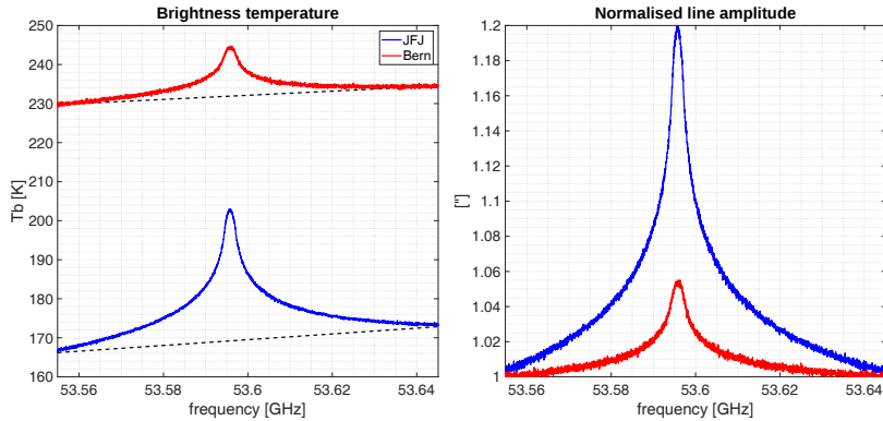
Figure 6. Comparison of calibrated TEMPERA-C measurements between Bern and the Jungfrauoch high altitude station. The comparison illustrates two measurements of the fine structure emission line at 53.596 GHz in single polarization taken at the Sphinx observatory and at the University of Bern, both during clear sky conditions. The left figure shows the direct comparison after calibration as a solid line, while the contribution from the troposphere (tropospheric background) is depicted as a dashed line. The right figure illustrates the same data normalized by dividing the spectra by the corresponding tropospheric background.
