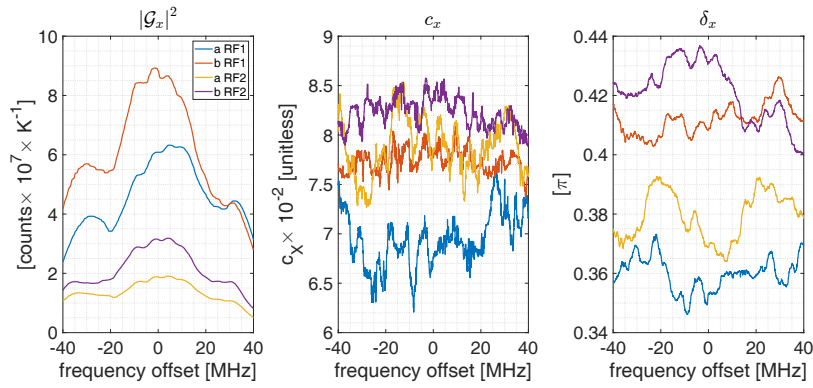
Figure 9. Cross-talk parameters calculated according Eq. (34)-(37). The RF 1 and RF 2 center frequencies are tuned to 53.07 GHz and 53.6 GHz, respectively. The subscripts a and b denote the two orthogonally polarized receivers, while x serves as a placeholder for either a or b .
