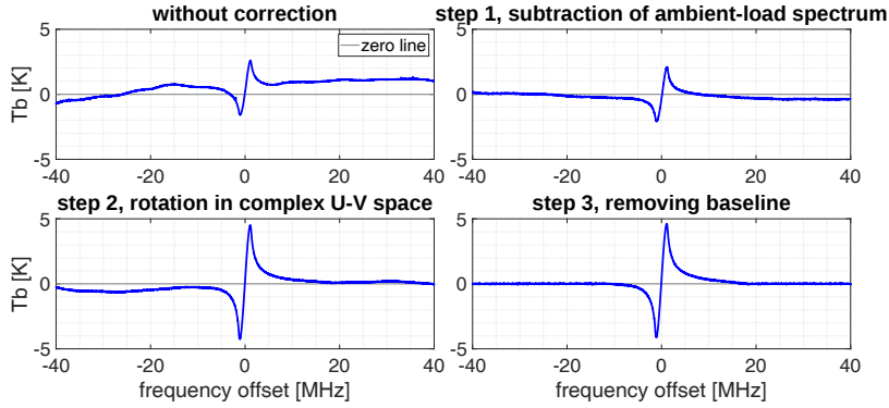
Figure 10. Step-by-step correction of the V-Stokes component (Eq. (52)). Step 1 is after subtracting r_{3,4}^{\text{hot}} , step 2 is after rotating by \Delta\phi , and step 3 is after removing R_X by interpolation. The illustration is provided for the emission line centered at 53.067 GHz. The correction for the other line centered at 53.596 GHz follows analogously.
