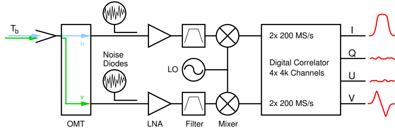
Figure 2. Simplified schematic of the TEMPERA-C front- and back-end (Krochin et al. (2022b)). The subscripts h and v denote the two pathways for horizontal and vertical polarization. The Stokes vector representation I, Q, U, V is of illustrative purpose. The direct output of the digital correlator has the representation of the modified Stokes vector (Sec. 2).
