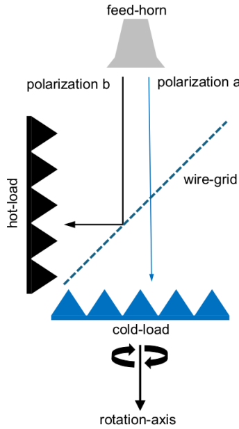
Figure 7. Measurement setup according to Gasiewski and Kunkee (1993). The wire grid is positioned at a 45^\circ angle between the hot-load and cold-load. The rotation of the grid by the angle \alpha occurs around the axis indicated by the black straight arrow. The optical paths for the two orthogonally polarized receiver chains, labeled as a and b , are depicted for the case when \alpha = 0 .
