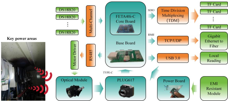
95 Figure 4: Hardware circuit structure
