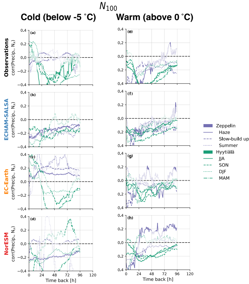
Figure 8. Spearman correlations between precipitation rate and N_{100} for cold (defined as below -5^{\circ}\text{C} at the station) versus warm (defined as above 0^{\circ}\text{C} at the station) conditions at the station separately. Otherwise the same as Fig. 7.
