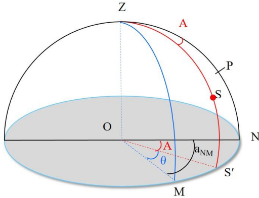
100 Figure 1: Spherical Diagram of Astronomical Azimuth
