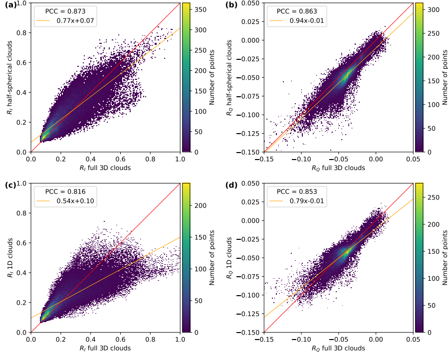
Figure 7. Scatter plots of the simulations with half-spherical clouds in the IDEFAX and one-dimensional clouds in the ICA against the real full three-dimensional simulation for R_I (a,c) and R_Q (b,d). Panels (a) and (b) show the comparison for half-spherical clouds, (c) and (d) for one-dimensional clouds. The red curve shows the identity, the orange curve a linear fit to the data. The fit parameters and the Pearson correlation coefficients (corresponding to the R value) are given in the legends.
