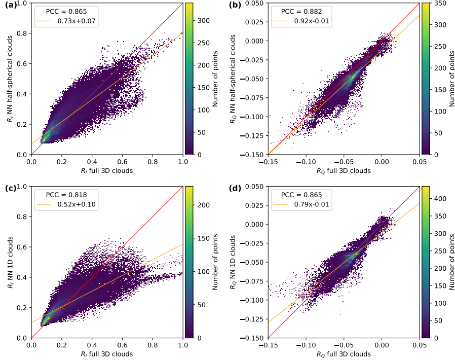
Figure 9. Scatter plots of the simulations with the neural networks for half-spherical clouds with the IDEFAX and one-dimensional clouds against the real - full three-dimensional simulation for R_I (a,c) and R_Q (b,d). Panels (a) and (b) show the comparison for half-spherical clouds, (c) and (d) for one-dimensional clouds. The red curve shows the identity, the orange curve a linear fit to the data. The fit parameters and the Pearson correlation coefficients (corresponding to the R value) are given in the legends.
