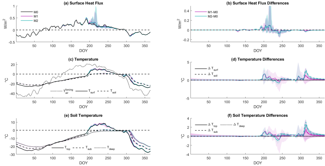
Figure 2. Simulation- Single-year simulation results (left; M0: black, M1: purple, M2: green) and deviations from reference model M0 (right; M1: purple, M2: green; eq. 5) for surface heat fluxes (top row), surface temperatures (middle rows), and soil temperatures (bottom row). Lines represent spatial mean, whereas shaded areas show the intra-model ranges, i.e. the ranges among columns for M1 and M2. The full simulated timeseries can be found in the appendix (fig.: B1). (a) Simulated surface heat flux ( F_{surf} ), which is defined as sum of sensible heat flux ( H ) and latent heat flux ( \lambda E ) at the surface, which directly interacts with the atmosphere, i.e. soil surface or snow. (b) Differences of surface heat fluxes ( \Delta F_{surf} ). (c) Simulated surface temperature ( T_{surf} , solid lines), whereby surface refers to the surface that is interacting with the atmosphere directly, as well as soil temperature ( T_{soil} , all depths up to 1m depth, dashed lines), and atmospheric forcing temperature ( T_{atm}^{forcing} , dotted line) for comparison. (d) Differences in surface temperature ( \Delta T_{surf} , solid lines) and soil temperature ( \Delta T_{soil} , all depths up to 1m depth, dashed lines). (e) Simulated soil temperatures in topsoil (0-20cm depth; T_{top} , solid lines), subsoil (20-80cm depth; T_{sub} , dashed lines), and deep soil (80-100cm depth; T_{deep} , dotted lines). (f) Differences in topsoil ( \Delta T_{top} , solid lines), subsoil ( \Delta T_{sub} , dashed lines), and deep soil temperatures ( \Delta T_{deep} , dotted lines).
