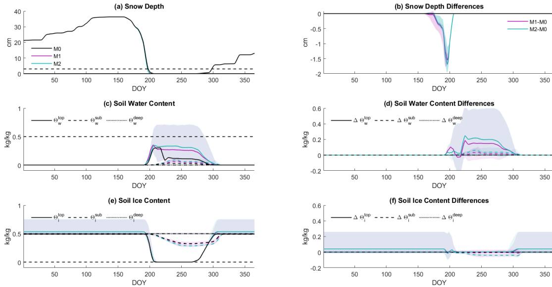
Figure B2. Simulation results (left; M0: black, M1: purple, M2: green) and deviations from reference model M0 (right; M1: purple, M2: green; eq. 5) for snow height-depth (top row), soil water content (kg water per kg dry soil; middle rows), and soil ice content (kg ice per kg dry soil; bottom row). Lines represent spatial mean, whereas shaded areas show the intra-model ranges, i.e. the ranges among columns for M1 and M2. (a) Simulated snow height-depth. Dashed line indicates 3cm-threshold for snow effects on surface albedo and soil insulation. (b) Differences in simulated snow height-depth. (c) Simulated soil water content in topsoil (0-20cm depth; \Theta_w^{top} , solid lines), subsoil (20-80cm depth; \Theta_w^{sub} , dashed lines), and deep soil (80-100cm depth; \Theta_w^{deep} , dotted lines). (d) Differences in topsoil ( \Delta\Theta_w^{top} , solid lines), subsoil ( \Delta\Theta_w^{sub} , dashed lines), and deep soil water contents ( \Delta\Theta_w^{deep} , dotted lines). Black dashed line represents mean porosity ( \Theta_{pore}^{soil} , tab. 3) as indicator for an upper limit for \Theta_w . (e) Simulated soil ice content in topsoil (0-20cm depth; \Theta_i^{top} , solid lines), subsoil (20-80cm depth; \Theta_i^{sub} , dashed lines), and deep soil (80-100cm depth; \Theta_i^{deep} , dotted lines). Black dashed line represents mean porosity ( \Theta_{pore}^{soil} , tab. 3) as indicator for an upper limit for \Theta_i . (f) Differences in topsoil ( \Delta\Theta_i^{top} , solid lines), subsoil ( \Delta\Theta_i^{sub} , dashed lines), and deep soil ice contents ( \Delta\Theta_i^{deep} , dotted lines).
