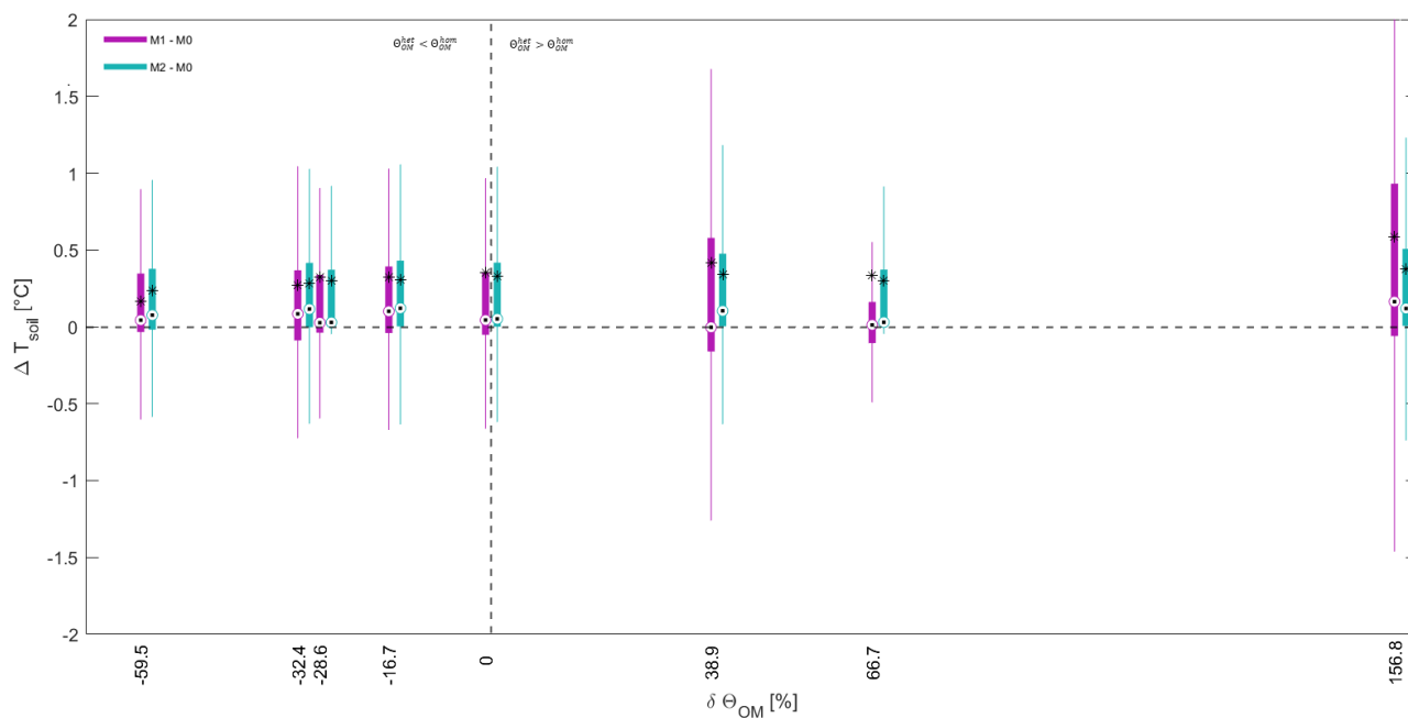
Figure B4. Differences in simulated daily soil temperature per grid cell between M1 and M0 (purple), as well as M2 and M0 (green) calculated by equation 5. Grid cells are aggregated by changes in OM content ( \delta\Theta_{OM} , eq. ??) between the heterogeneous and the homogeneous soil inputs. Boxes represent quartile range of data and whiskers show the 0.1-0.9-quantile range. Circles show data median, whereas stars indicate data mean.
