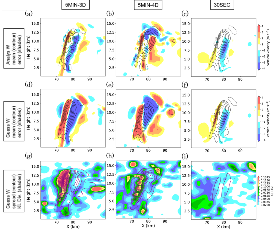
Figure 10. Same with figure 4 but for the experiments with background wind perturbation. Purple contours in (g-i) indicate first guess ensemble spread of vertical velocity with contour interval of 1 m s -1 .
