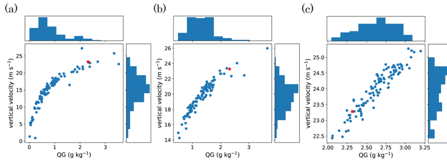
Figure 7. The examples of scatter plots of 100 ensemble members between graupel mixing ratio (QG) and vertical velocity (W) for each of (a) 5MIN-3D, (b) 5MIN-4D, and (c) 30SEC cases, at 00:50:00 as in Fig. 5 . The blue dots indicate values of each ensemble member. The red star marker indicates the value of nature run. Histograms of QG and W are shown on the top and on the right of each panel, respectively.
