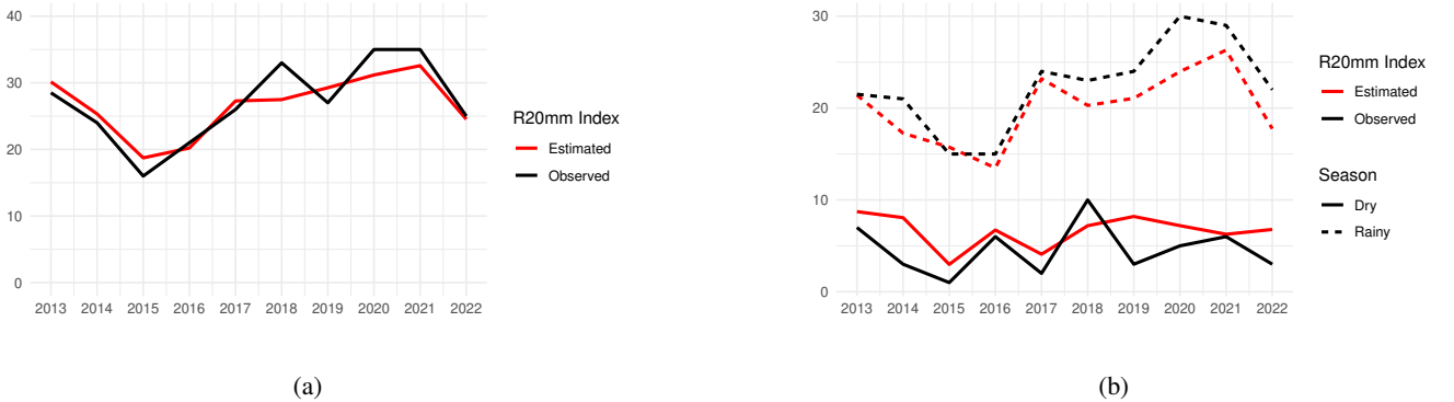
Figure 3. The estimated and the observed R20mm index by year (a) and season (b) at station s_3 .
