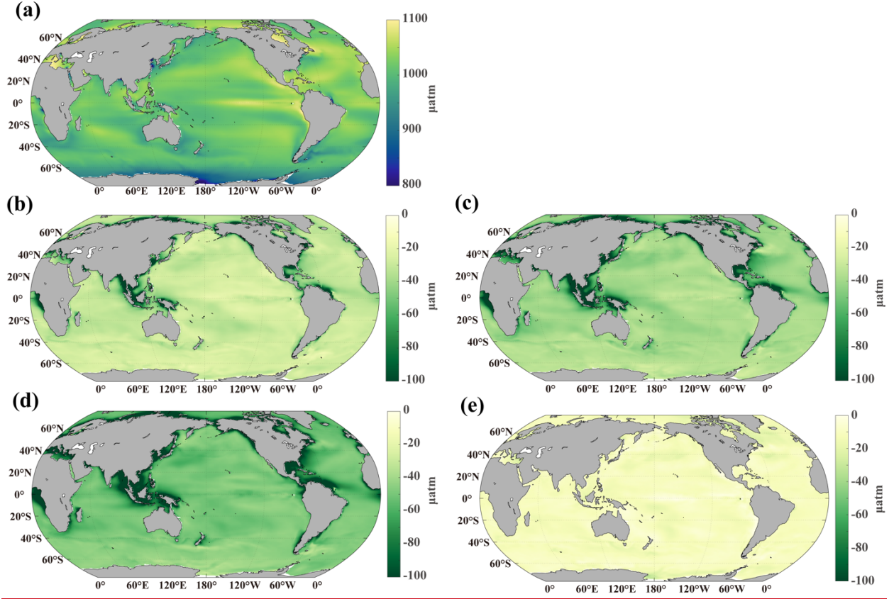
305 Figure 65: Distribution of surface p\text{CO}_2 . (a) control simulation, (b) difference between OWE5 and CTL, (c) difference between OWE75 and CTL, (d) difference between OWE10 and CTL, (e) difference between OWE0 and CTL. All the comparisons are based on the average of the last 10 years of simulation.
