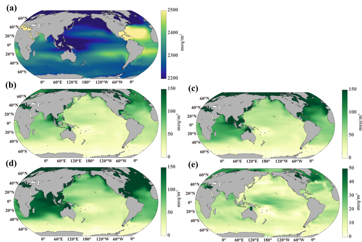
Figure 43: Distribution of alkalinity (unit: \text{meq/m}^3 ) in upper 100 m. (a) upper 100 m mean alkalinity in the upper 100 m in control simulation at the end of this century, (b) differences between OWE5 and CTL, (c) differences between OWE75 and CTL, (d) differences between OWE10 and CTL, (e) differences between OWE0 and CTL. Note the different colour scale of (e). All the comparisons are based on the average of the last 10 years of simulation.
