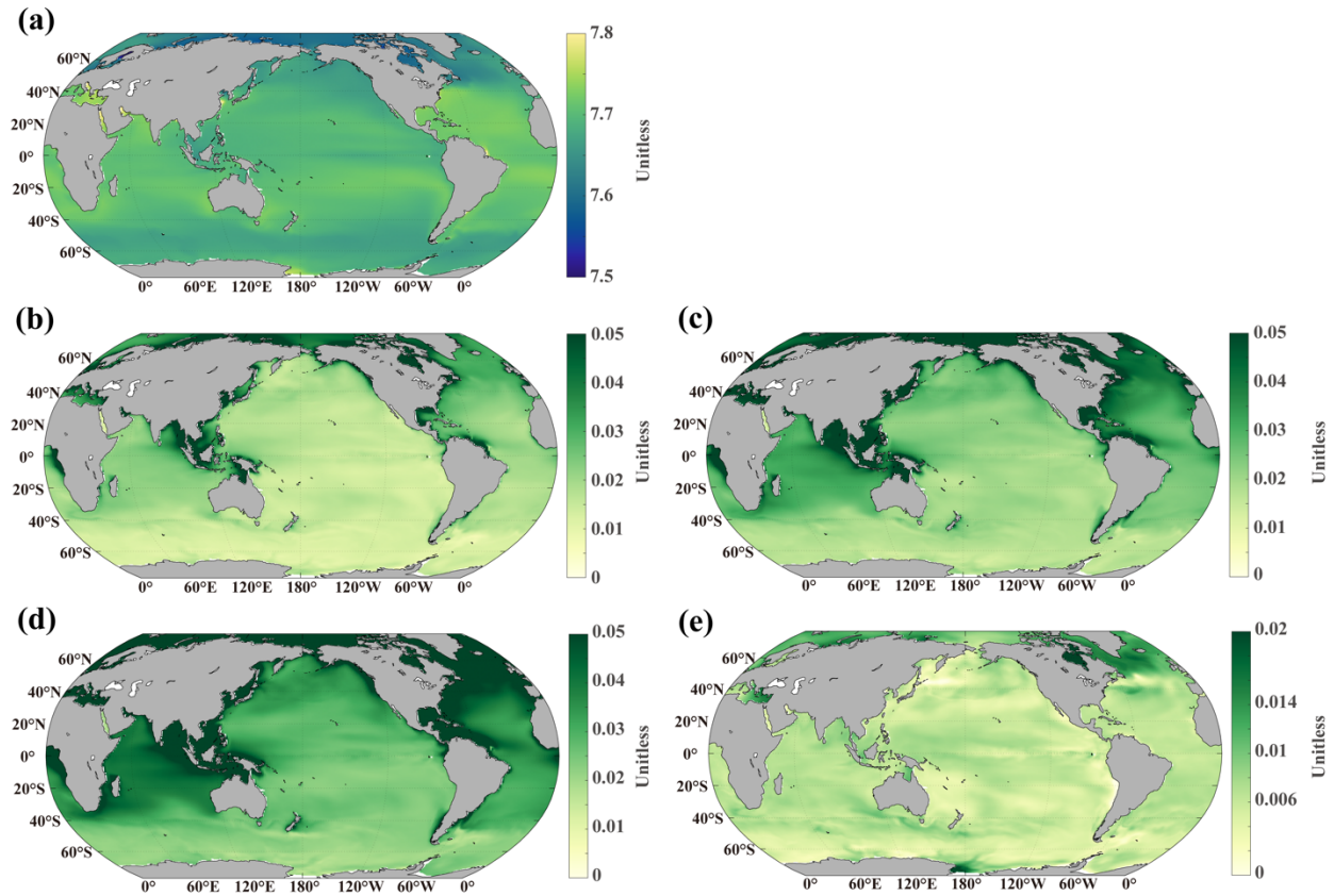
Figure 98: Distribution of surface pH. (a) control simulation at the end of the century, (b) difference between OWE5 and CTL, (c) difference between OWE75 and CTL, (d) difference between OWE10 and CTL, (e) difference between OWE0 and CTL. Note the different colour scale in (e). All the comparisons are based on the average of the last 10 years of simulation.
