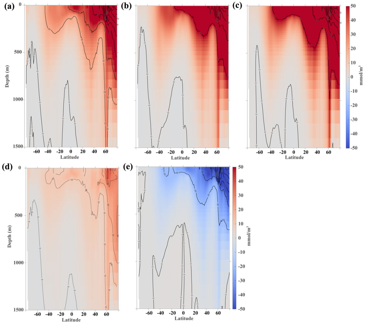
Figure 8. Vertical7. Zonal mean vertical distribution of DIC inventoryconcentration anomalies (upper 1500 m). (a) differences between OWE5 and CTL, (b) difference between OWE75 and CTL, (c) difference between OWE10 and CTL, (d) differences between OWE0 and CTL, and (e) differences between OWE0 and OWE5. All the comparisons are based on the average of the last 10 years of simulation.
