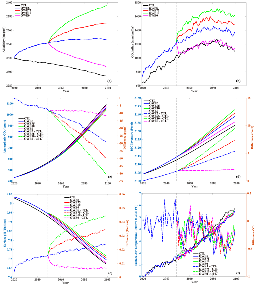
Figure 3: Global2: Temporal changes of (a) upper 100-m-mean alkalinity in the upper 100 m (unit: meq/m 3 ), (b) CO 2 influx (unit: mmol/m 2 /yr), (c) atmospheric CO 2 (unit: ppmv), (d) integrated DIC inventory (unit: Pmol), (e) surface pH, (f) surface air temperature (unit: °C). DashPerpendicular grey dash lines starting from in the year of 2050 denote the onset of the 7.5××, 10×× alkalinity enhancement scenarios, (OWE 75 and OWE10, respectively) , as well as the termination of alkalinity addition via rivers . (OWE0) . The coloured dash lines in (c), (d), (e), (f) are the anomaly between OAE simulations and the control run.
