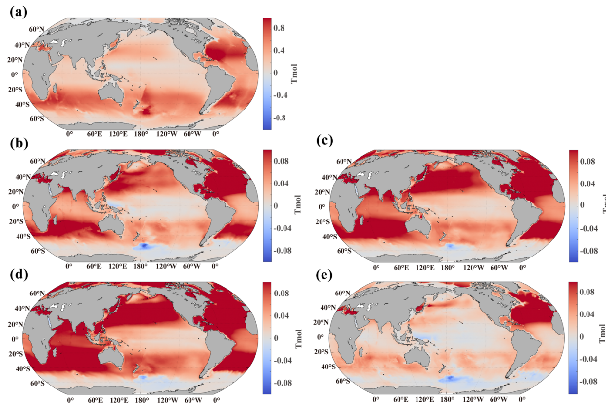
Figure 76: Anomaly of DIC inventory. (a) Change in DIC inventory at the end of the century relative to the initial year, (b) difference between OWE5 and CTL, (c) difference between OWE75 and CTL, (d) difference between OWE10 and CTL, and (e) difference between OWE0 and CTL. All the comparisons are based on the average of the last 10 years of simulation.
