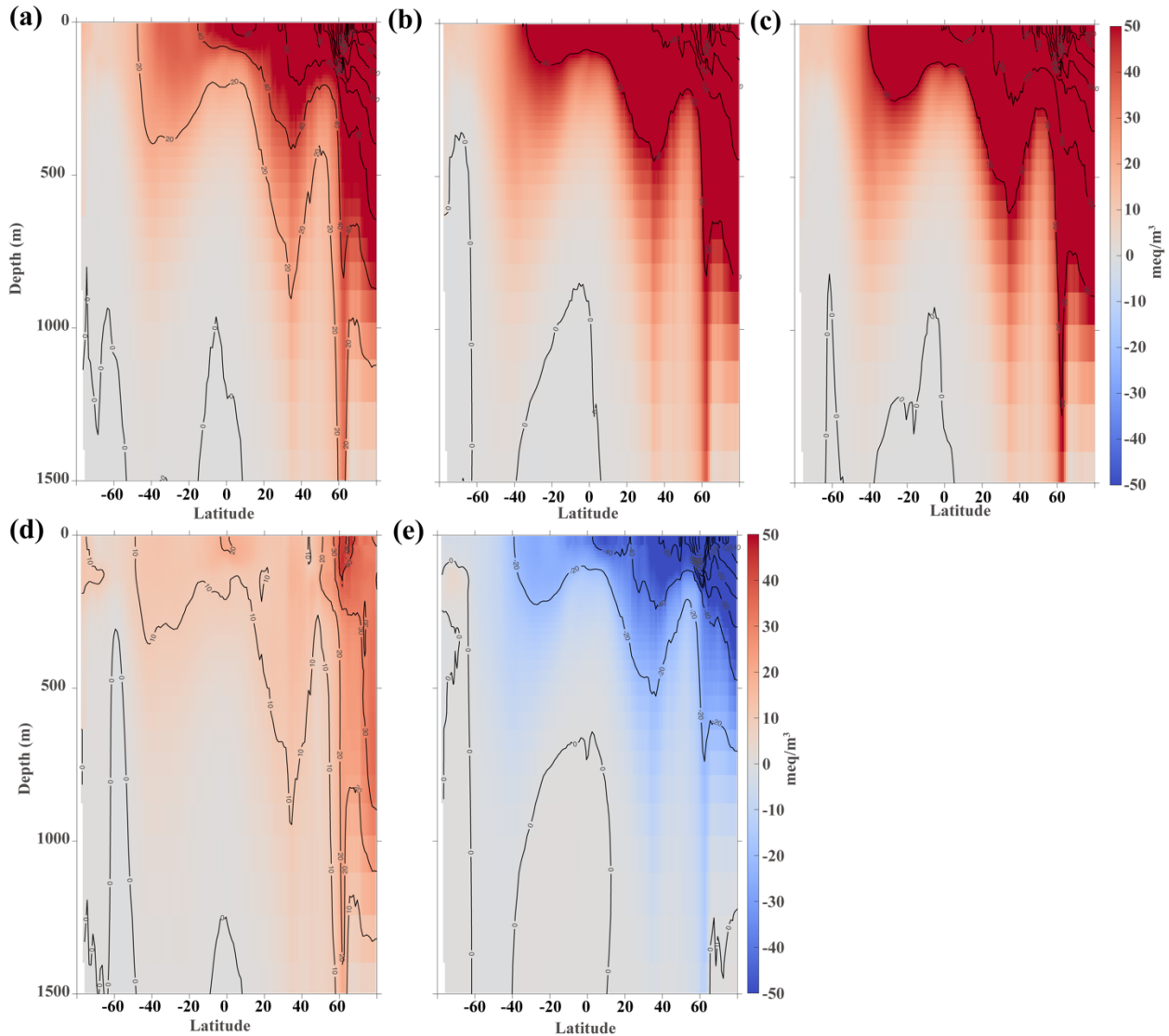
Figure 54: Vertical distribution of zonal mean alkalinity anomaly (upper 1500 m). (a) differences between OWE5 and CTL, (b) differences between OWE75 and CTL, (c) differences between OWE10 and CTL, (d) differences between OWE0 and CTL, (e) differences between OWE0 and OWE5. All the comparisons are based on the average of the last 10 years of simulation.
