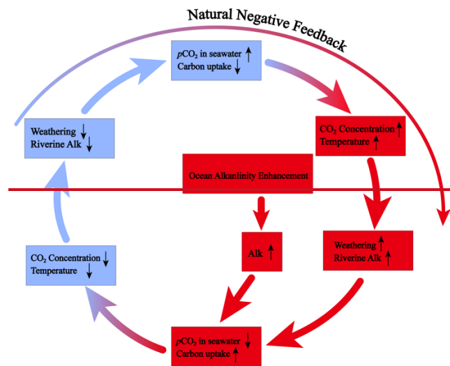
Figure1: Schematic diagram of natural negative feedback and OAE mechanism. This study provides the transient responses of ocean system to OAE and insights into persistence and reversibility of OAE-induced changes, as well as the suggestion to future study and deployment of OAE.
