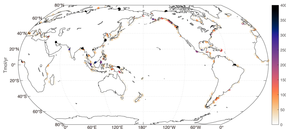
Figure 21: Location and fluxes of enhanced alkalinity input.
