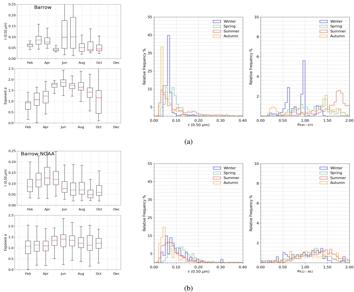
Figure 2. Left-hand side: Time-patterns of the monthly mean values and the first and third quartiles of aerosol optical thickness \tau(0.500\mu m) and the Ångström exponent \alpha . The whiskers extend from the box to the farthest data point within 1.5 times the interquartile range (IQR) from the box. Right-hand side: relative frequency histograms for \tau(0.500\mu m) and \alpha separately for winter (arctic haze, DJF), spring (MAM), summer (background, JJA), and autumn (SON). These statistics were obtained from multi-year sun-photometer measurements conducted at Barrow by (a) Atmospheric Radiation Measurements, and by (b) National Oceanic and Atmospheric Administration.
