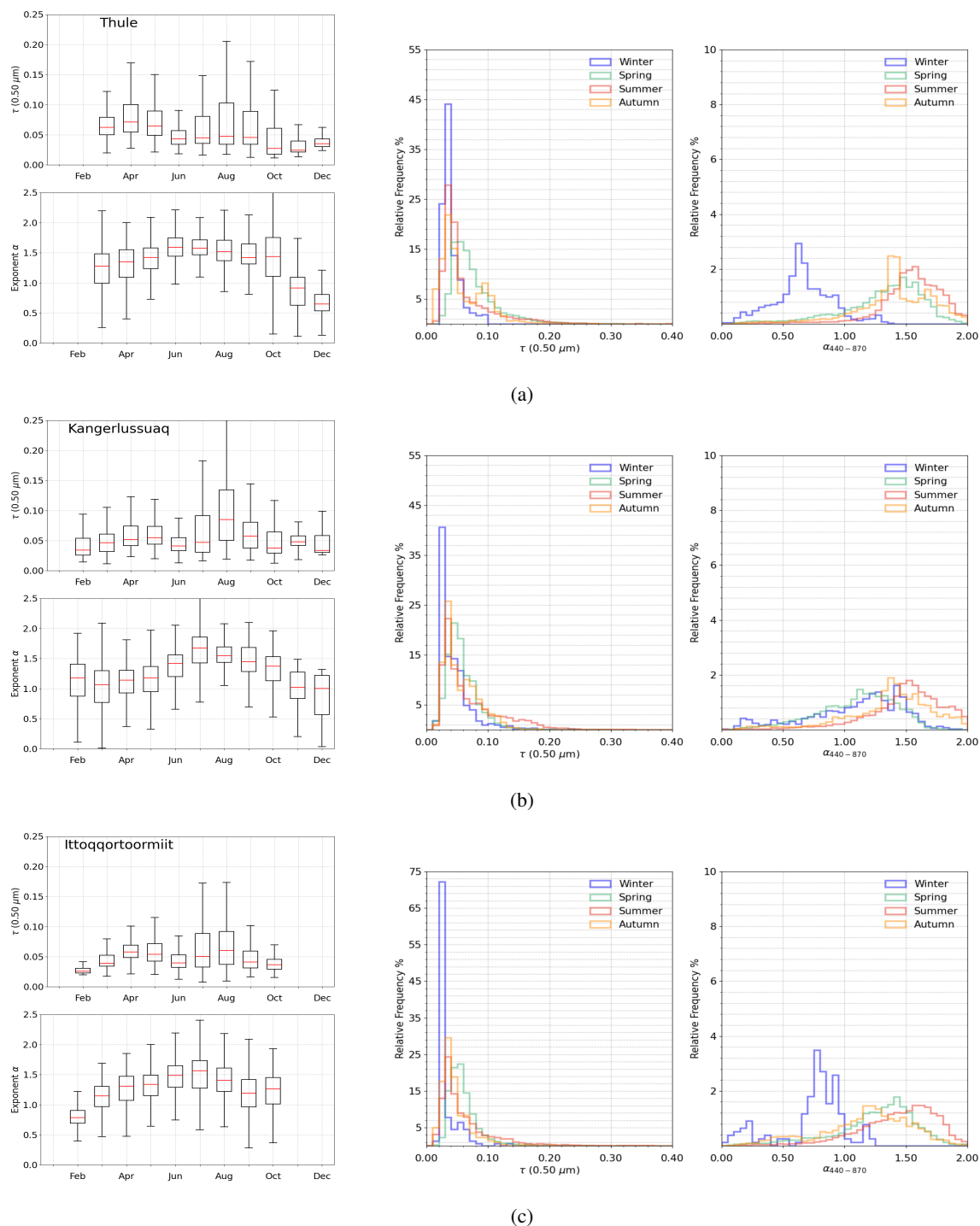
Figure 5. As in Fig.2, for the multi-year sun-photometer measurements of aerosol optical depth \tau(0.500\mu\text{m}) and exponent \alpha conducted at: (a) Thule, (b) Kangerlussuaq and (c) Ittoqqortoormiit by NASA Goddard Space Flight Center. To show clearly the RFH of \tau(0.500\mu\text{m}) , the y-axis scale for the Ittoqqortoormiit station has been adjusted to range from 0 to 75.
