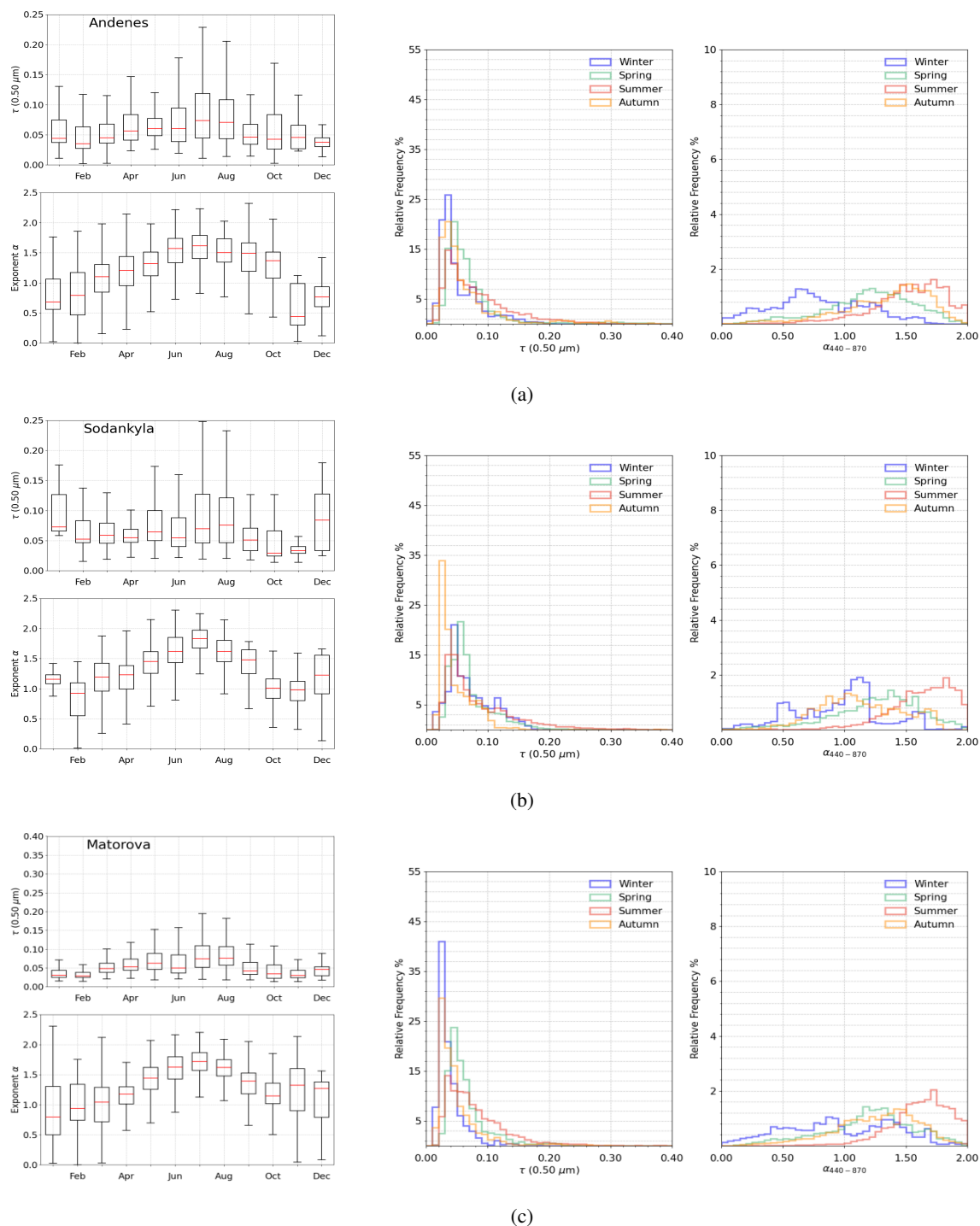
Figure 8. As in Fig.2, for the multi-year sun-photometer measurements of aerosol optical depth \tau(0.500\mu\text{m}) and exponent \alpha conducted at: (a) Andenes by Andøya and University of Valladolid, (b) Sodankylä and (c) Matorova by the Finnish Meteorological Institute.
