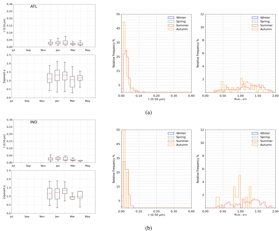
Figure 16. Multi-year sun-photometer measurements of aerosol optical depth \tau(0.500\mu\text{m}) and exponent \alpha conducted by several research institution during scientific cruises in the Antarctic ocean between 2004 and 2024.
