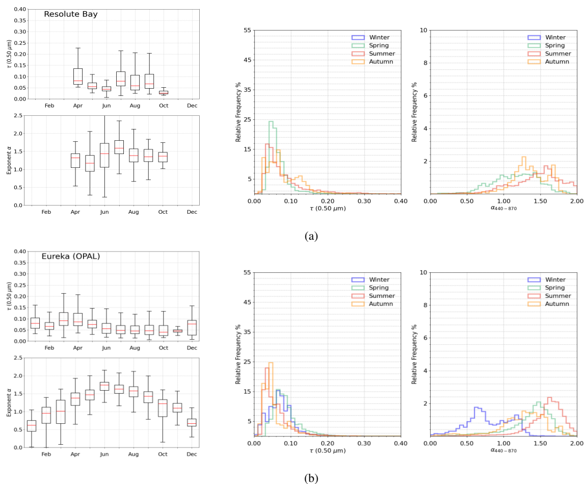
Figure 4. As in Fig.2, for the multi-year sun-photometer measurements of aerosol optical depth \tau(0.500\mu m) and exponent \alpha conducted at: (a) Resolute Bay by AEROCAN; (b) Eureka (OPAL).
