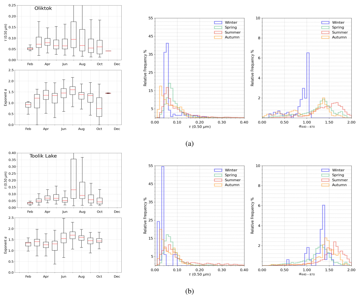
Figure 3. As in Fig.2, for the multi-year sun-photometer measurements of aerosol optical depth \tau(0.500\mu m) and exponent \alpha conducted at: (a) Oliktok by Atmospheric Radiation Measurements, and (b) Toolik Lake by National Ecological Observatory Network. To show the monthly boxplot of \tau(0.50\mu m) , the y-axis scale for the Toolik Lake station has been adjusted to range from 0 to 0.40.
