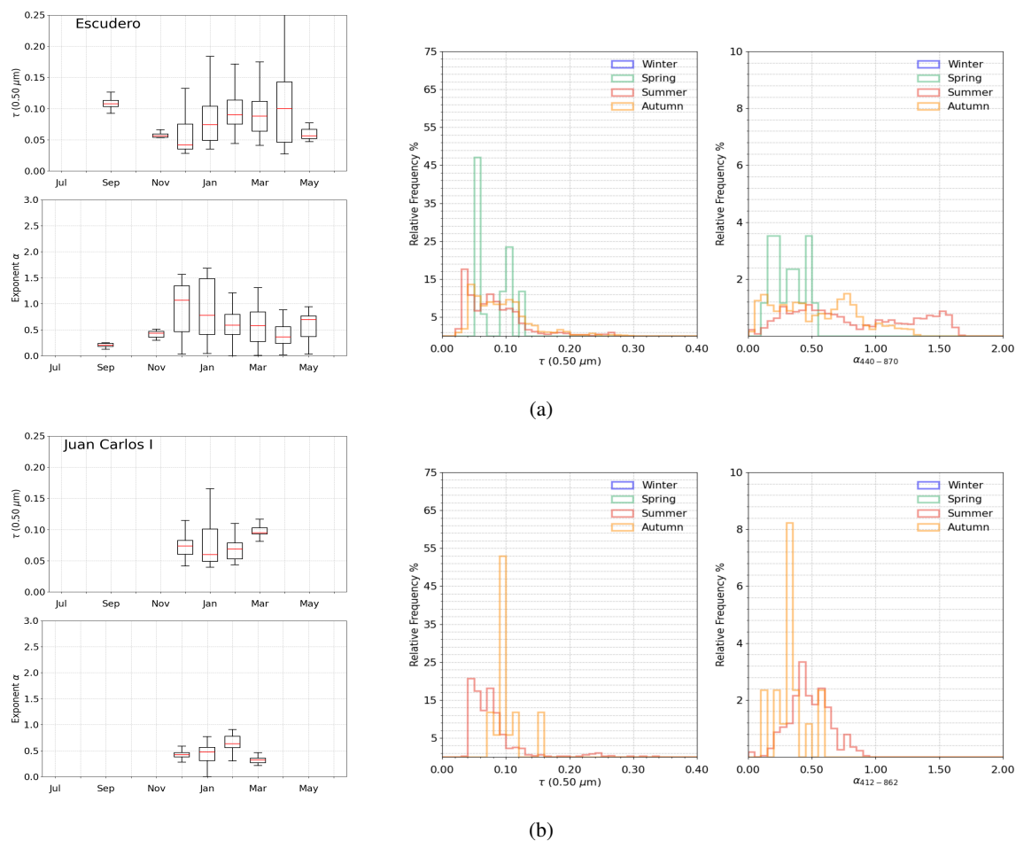
Figure 9. As in Fig.2, for the multi-year sun-photometer measurements of aerosol optical depth \tau(0.500\mu m) and exponent \alpha conducted at: (a) Escudero by University of Santiago and Chilean Antarctic Institute, and (b) Juan Carlos I by University of Valladolid.
