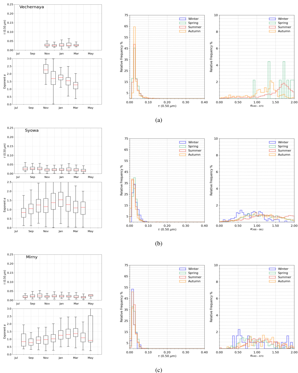
Figure 12. As in Fig.2, for the multi-year sun-photometer measurements of aerosol optical depth \tau(0.500\mu\text{m}) and exponent \alpha conducted at: (a) Vechernaya Hill by National Academy of Sciences of Belarus and University of Lille (b) Syowa by the Japan Meteorological Agency, and (c) Mirny by the Arctic and Antarctic Research Institute.
