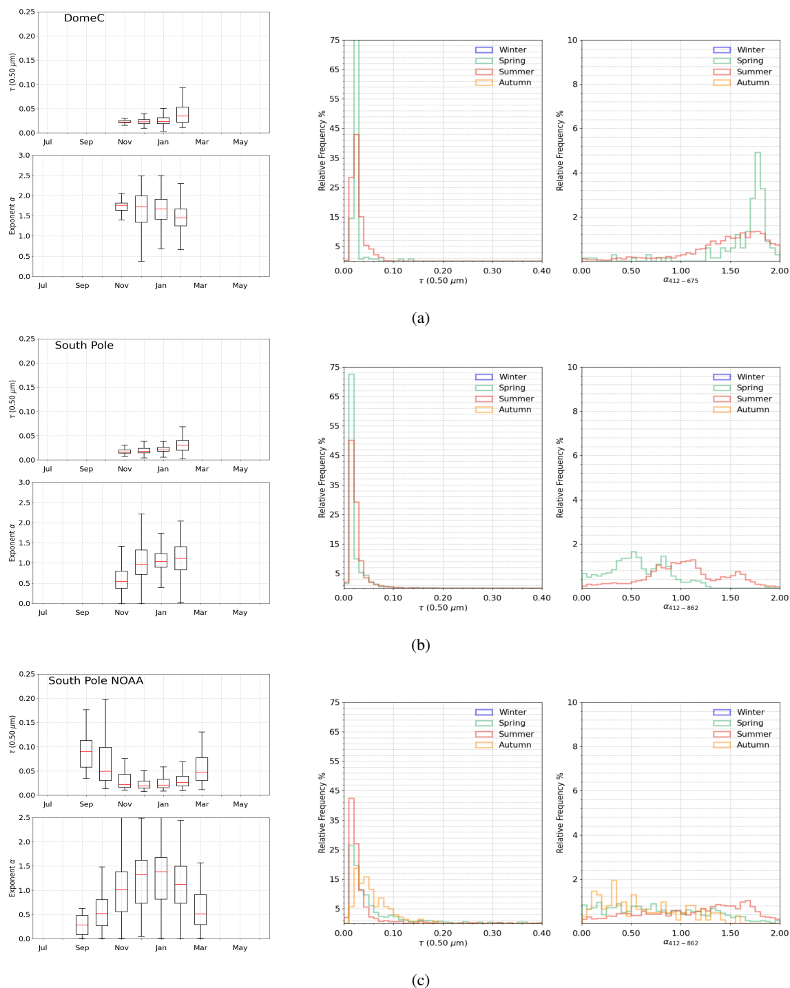
Figure 13. As in Fig.2, for the multi-year sun-photometer measurements of aerosol optical depth \tau(0.500\mu\text{m}) and exponent \alpha conducted at: (a) Dome C by National Research Council of Italy and National Oceanic and Atmospheric Administration (NOAA), (b) South Pole by NASA/GSFC, and (c) South Pole by NOAA.
