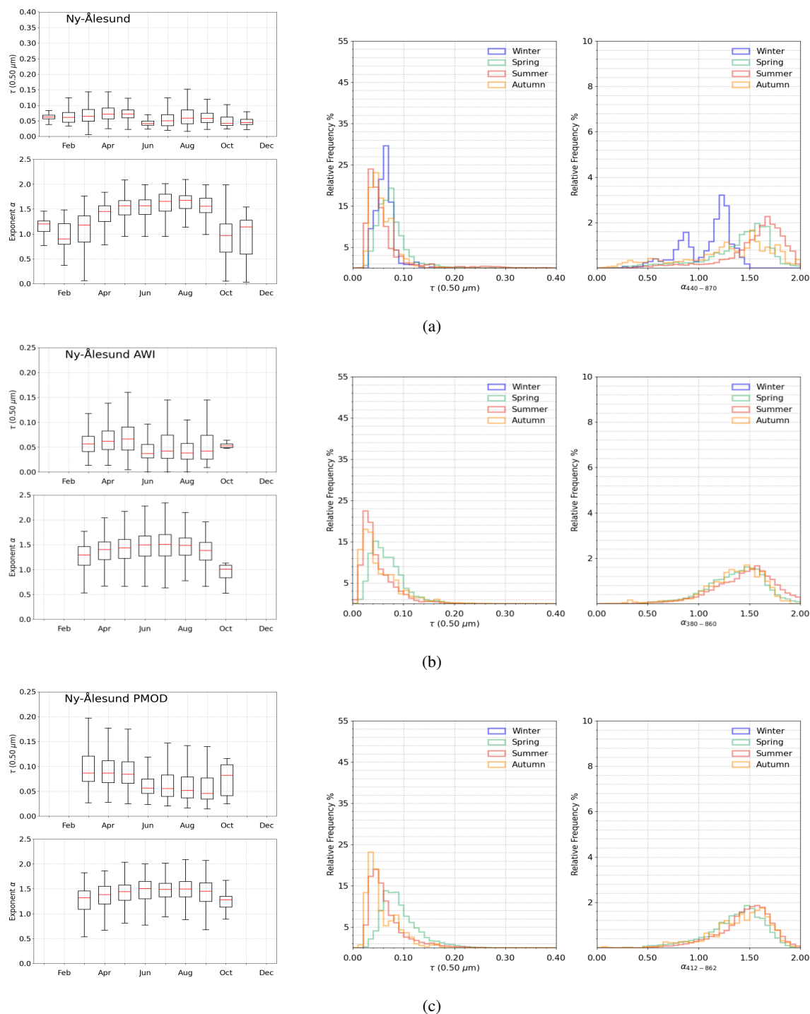
Figure 6. As in Fig.2, for the multi-year sun-photometer measurements of aerosol optical depth \tau(0.500\mu m) and exponent \alpha conducted at Ny-Ålesund: (a) by AWI and University of Valladolid using a CIMEL CE318-T, (b) by AWI using a SP1A, and (c) by PMOD and Norwegian Polar Institute using a PFR.
