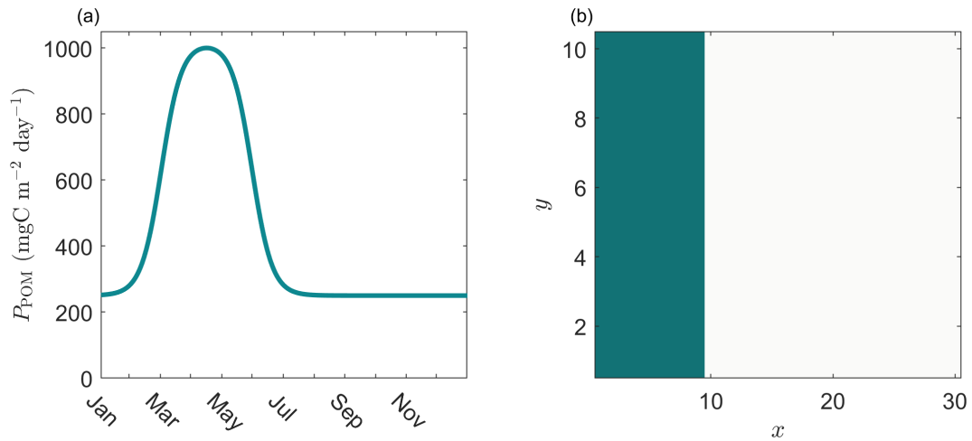
Figure 2. Reconstruction of (a) a simple annual production cycle of primary particles peaking in middle April, (b) which are assigned to a size range between 1\text{--}50\ \mu\text{m} and are equally distributed throughout the excess density space. x is the logarithmic scaling factor of aggregate size, y is the stretched logarithmic scaling factor of excess density (see Eq. 2). This scenario is the base for the results in section 3.2, section 3.3 and section 3.1 with the exception that in the latter analysis only primary particles of size 1\ \mu\text{m} are produced in this case study.
