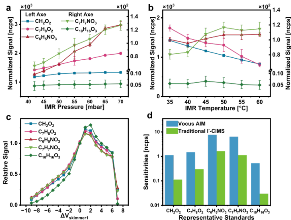
240 Figure 3. The optimization results: the dependence of instrument sensitivities of representative standards on the instrumental conditions, (a) IMR pressure, (b) IMR temperature, (c) voltage of skimmer in the BSQ and (d) the comparison of sensitivities in optimized Vocus AIM and traditional I-CIMS.
