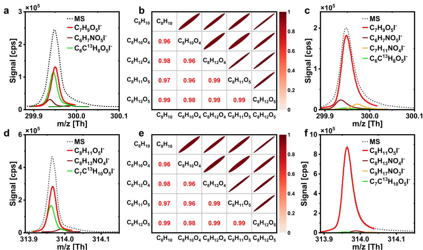
Figure 4. Peak fitting result for BPRs in the oxidation of (a) toluene, (d) m-xylene with H_2O photolysis the sole source of OH, correlation analysis of BPRs, precursors and products (b, e) and improvement in the peak fitting after adding H_2O_2 (c, f).
