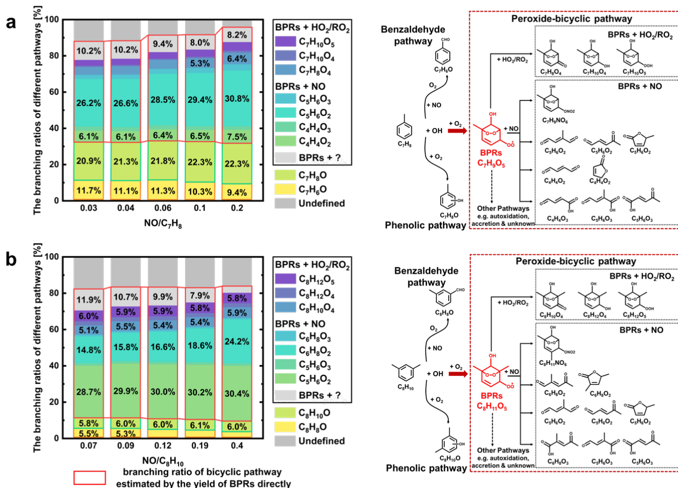
Figure 6. Experimental branching ratios for different pathways in the case of toluene and m-xylene, calculated by direct-measured method and product-yield method.
