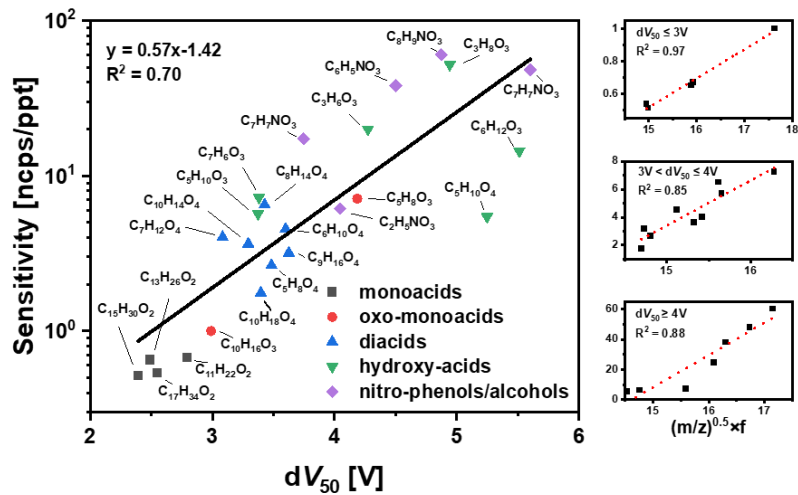
Figure S2 Relationship between the sensitivities and the corresponding dV_{50} values of standards in the AIM-CIMS (left). dV_{50} -based segmented linear fitting of the sensitivity and the product of the square root of m/z and fragmentation ratio (right).
