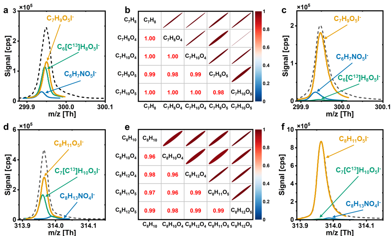
280 Figure 4. Peak fitting result for BPRs in the oxidation of (a) toluene, (d) m-xylene with H_2O photolysis the sole source of OH, correlation analysis of BPRs, precursors and products (b, e) and improvement in the peak fitting after adding H_2O_2 (c, f).
