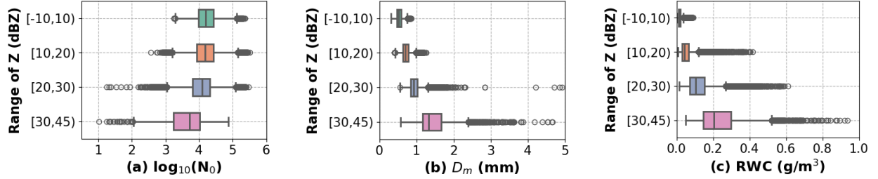
Figure 1. Box plots of the parameters of MP size distribution in different Z intervals. (a) \log_{10}(N_0) . (b) D_m . (c) RWC.
