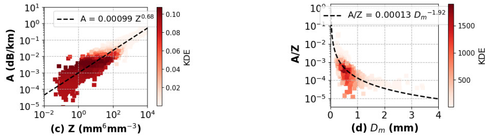
295 Figure 10. Empirical relations for QPE and attenuation correction using Ka-band radar in the eastern Tibetan Plateau. (a) Z-R relation. (b) D m -R relation, (c) Z-A relation. (d) D m -A/Z relation, where A refers to the specific attenuation in dB/km, Z in mm 6 m -3 .
