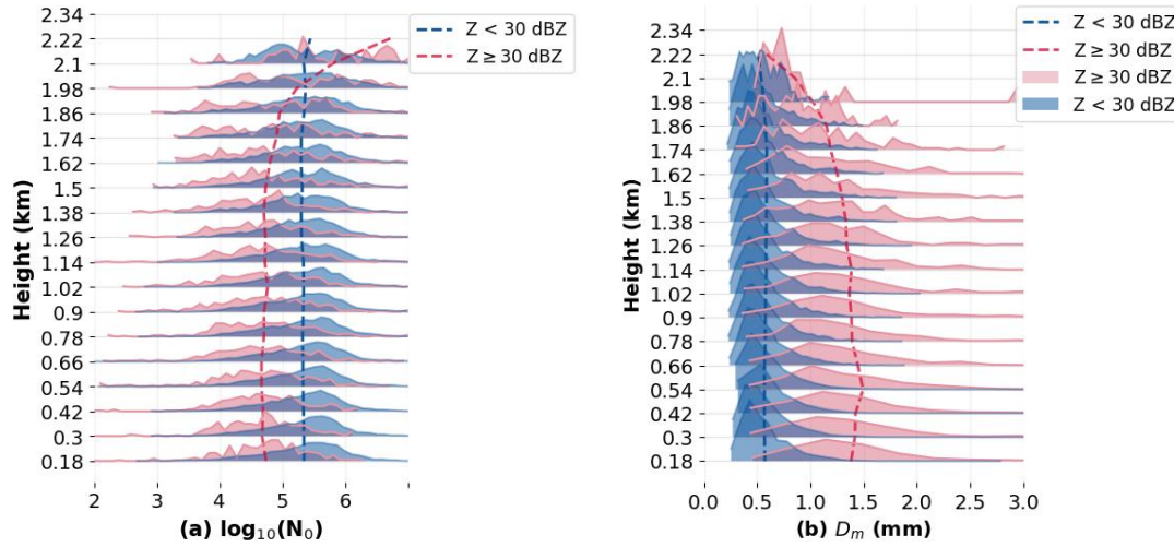
Figure 8. The distribution and the mean values of DSD parameters with height during July to August 2024 at Hongyuan. (a) \log_{10}(N_0) . (b) D_m .
