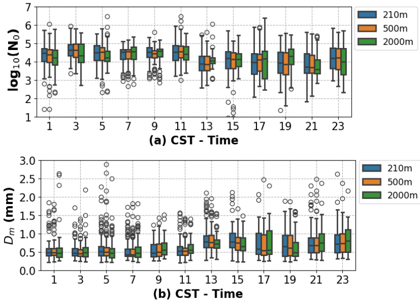
Figure 9. Box plots of the DSD parameters at 210, 500, and 2000 m. (a) N_0 . (b) D_m .
