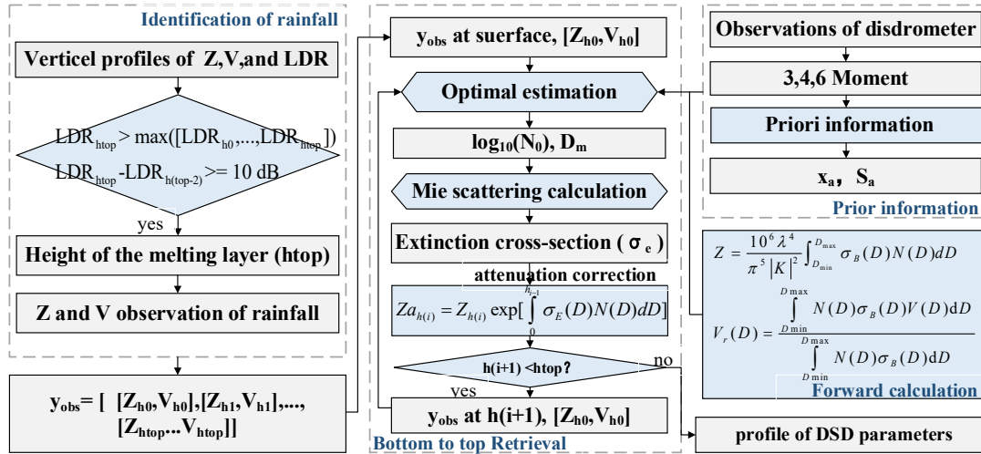
Figure 3. Flowchart for the retrieval method of vertical profiles of DSD parameters.
