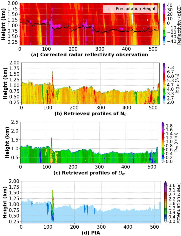
Figure 7. Profiles of the attenuation-corrected Z , the retrieved profiles of DSD parameters, and PLA of the precipitation on August 15, 2024. (a) Z . (b) \log_{10}(N_0) . (c) D_m and (d) PIA.
