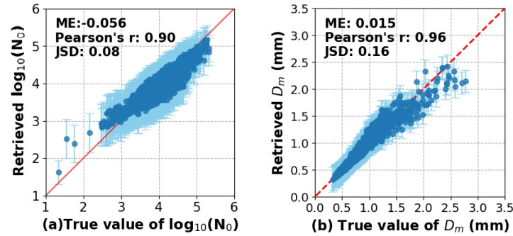
Figure 5. The retrieved values and the true values of \log_{10}(N_0) and D_m . (a) \log_{10}(N_0) . (b) D_m .
