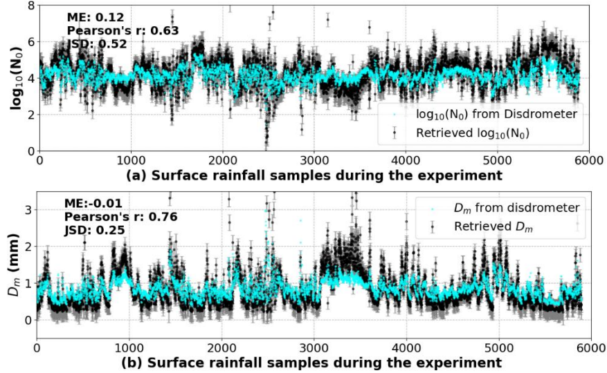
Figure 6. The retrieved and observed \log_{10}(N_0) and D_m during the field campaign in July and August 2024. (a) \log_{10}(N_0) . (b) D_m .
