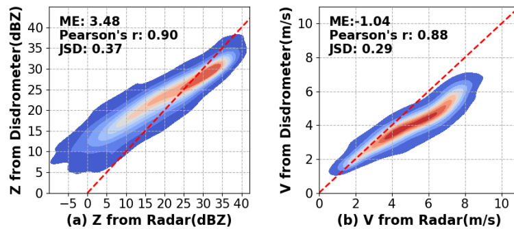
Figure 4. The true values of Z and V_r observed from the Ka-band zenith-pointing radar and simulated values during the field campaign in July and August 2024. (a) Z . (b) V_r .
