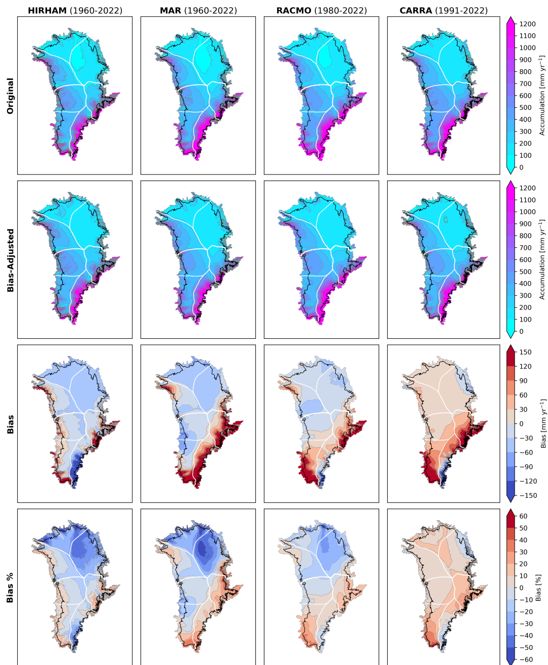
Figure A4. Mean maps of model accumulation and bias for the full model periods, HIRHAM (1960-2022), MAR (1960-2022), RACMO (1980-2022) and CARRA (1991-2022). The black line indicates the boundary of the accumulation zone. First row: original mean accumulation before adjustment. Second row: mean bias-corrected accumulation. Third row: mean bias in \text{mm yr}^{-1} . Fourth row: mean relative bias. PROMICE drainage basin boundaries are indicated in white.
