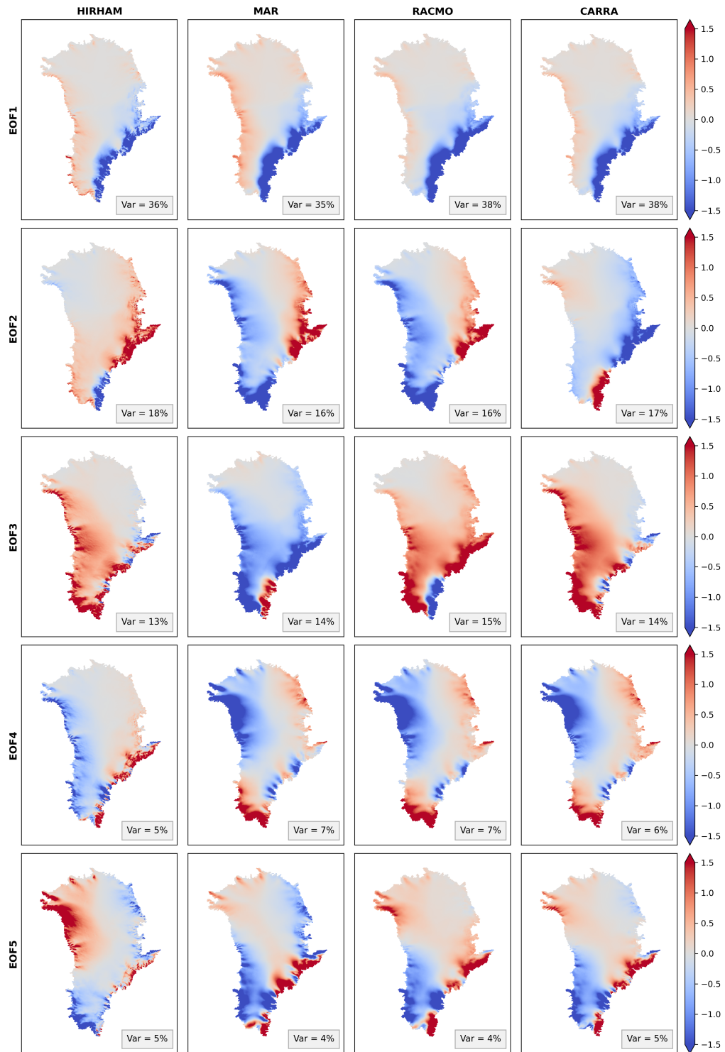
Figure A5. First five EOF patterns for HIRHAM, MAR, RACMO and CARRA over 1991-2022.
