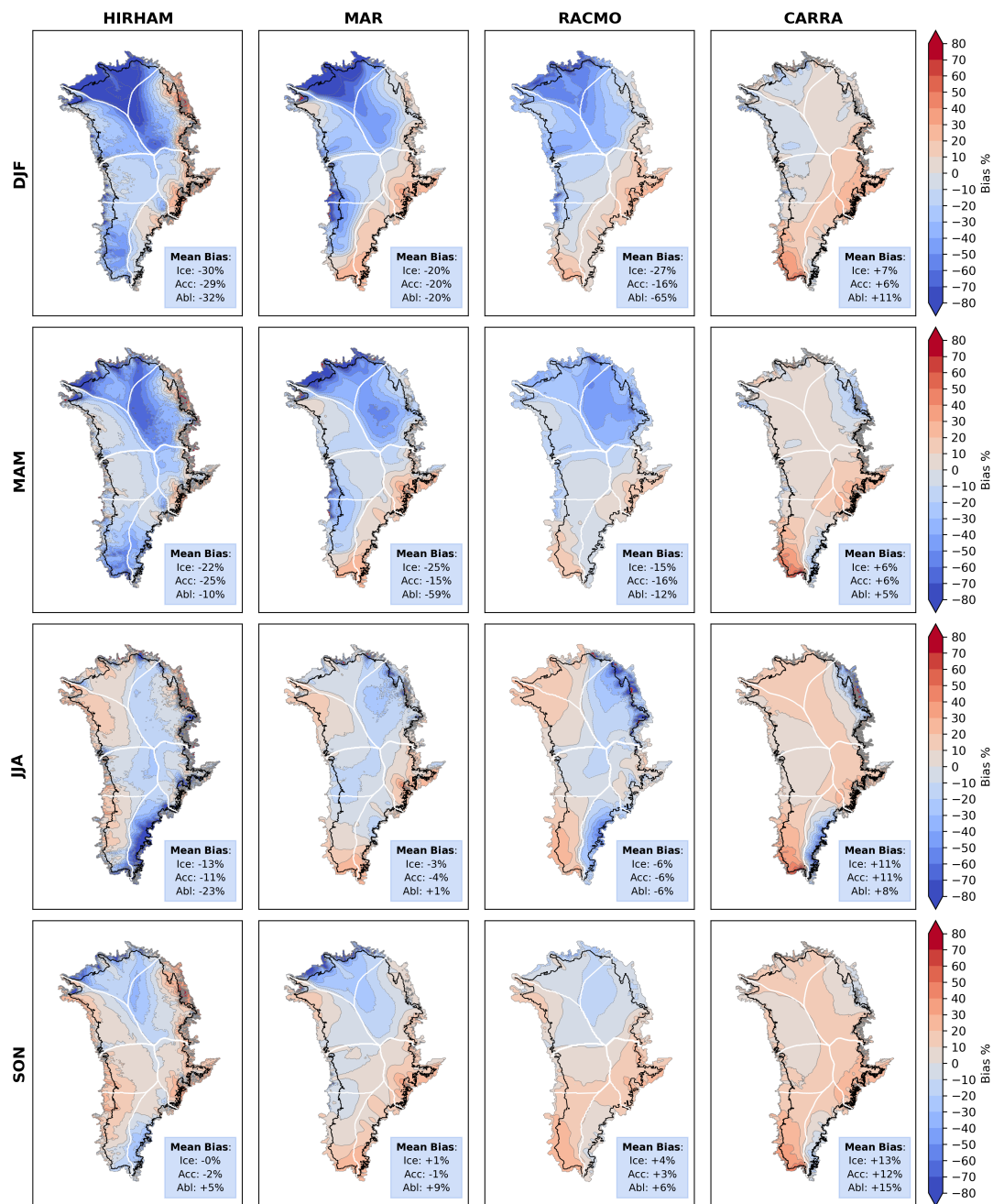
Figure 4. Model mean seasonal relative bias over the 1991-2022 common period: \text{mean}(\text{original} - \text{bias-adjusted})/\text{mean}(\text{original}) . Values stated in the lower right corners represent the mean bias for each season over the ice-sheet (Ice), accumulation zone (Acc) and ablation zone (Abl).
