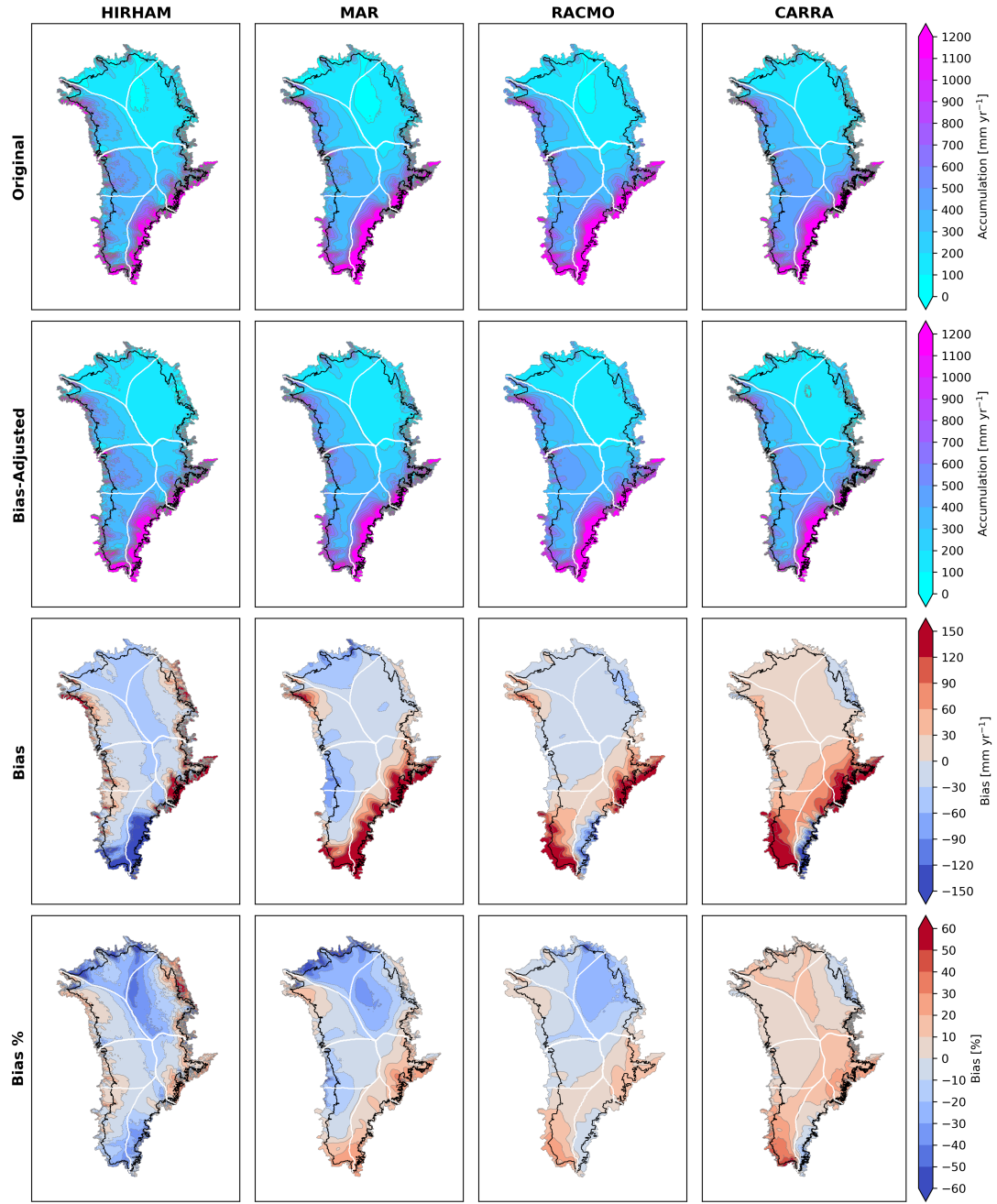
Figure 3. Mean maps of model accumulation and bias over over the 1991-2022 common period. The black line indicates the boundary of the accumulation zone. First row: original mean model accumulation before bias-adjustment. Second row: bias-corrected mean accumulation. Third row: mean bias in mm yr -1 , mean(original - bias-adjusted). Fourth row: mean relative bias, calculated by (eq. 11). PROMICE drainage basins boundaries are shown in white. Maps for the full model periods are provided in the appendix, Fig. A4.
