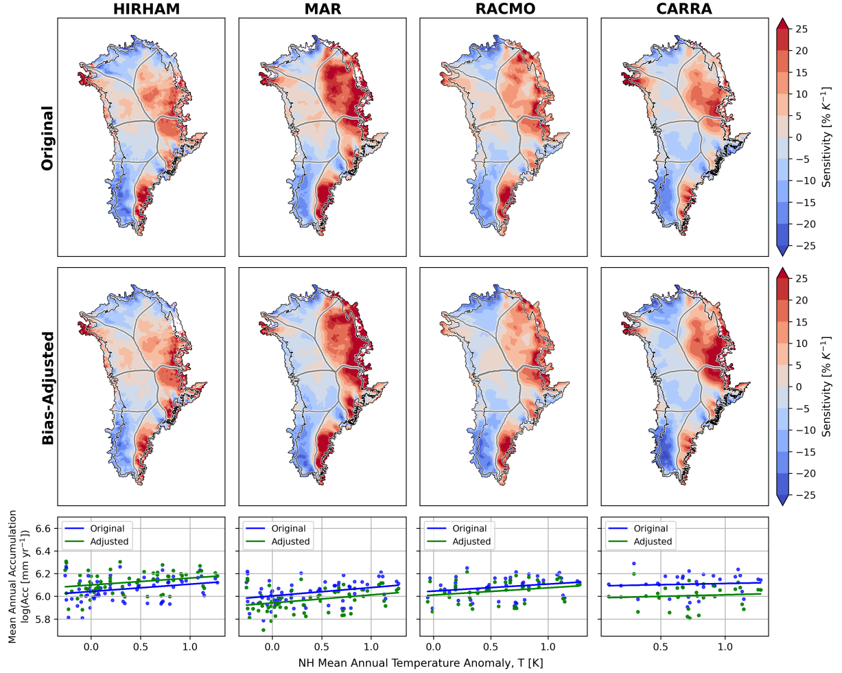
Figure 6. Temperature sensitivity analysis following eq. 12. Upper panels show spatial patterns of sensitivity over 1991-2022, derived from grid-point wise linear regressions of log-transformed annual model accumulation against NHT anomalies from HadCRUT5. Empty grid points resulting from negative accumulation values are excluded from calculation of mean ice-sheet sensitivities. Lower panels show ice-sheet wide mean annual accumulation (log-transformed) as a function of NHT anomalies with linear fits for HIRHAM (1960-2022), MAR (1960-2022), RACMO (1980-2022) and CARRA (1991-2022).
