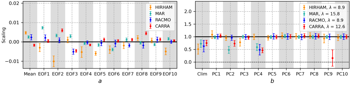
Figure 2. Bias-adjustment coefficients derived from fitting the 1991-2022 overlap period using the arctan loss function. Error bars represent the uncertainty in the parameter estimates, reflecting the confidence in the fitted coefficients rather than spatial variability. The initial guess (no adjustment) is denoted by the solid black line. Left: a parameters adjusting the time-independent mean bias and 10 EOF modes. Right: b parameters adjusting the time-dependent climatology and 10 PC modes, with \lambda values derived independently for each model via cross-validation.
