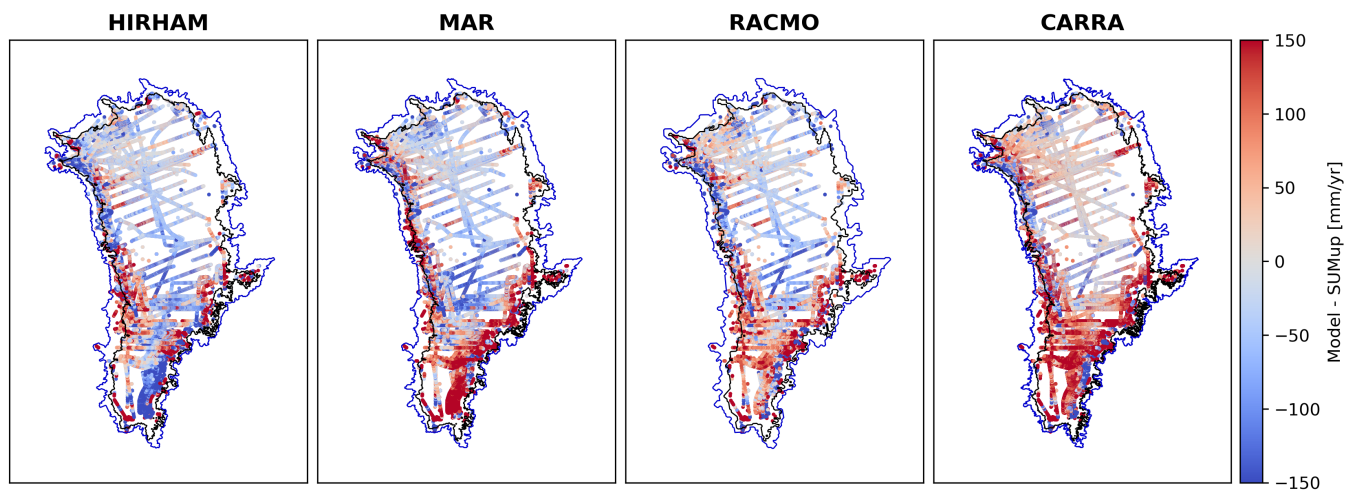
Figure A3. SUMup point-wise bias (1991-2022). The blue contour indicates the boundary of the PROMICE ice-sheet mask and the black contour shows the boundary of the accumulation zone.
