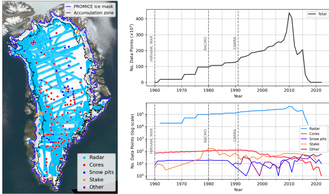
Figure 1. Left: geographical distribution of SUMup data points used in this study between 1960 and 2022, illustrated by measurement type. The method type ‘other’ includes mass balance profiles and SnowFox sensors. Right upper: time dependence of total number of data points with markers for the start year of model data. Right lower: time dependence of data points by measurement type, with counts in log scale.
