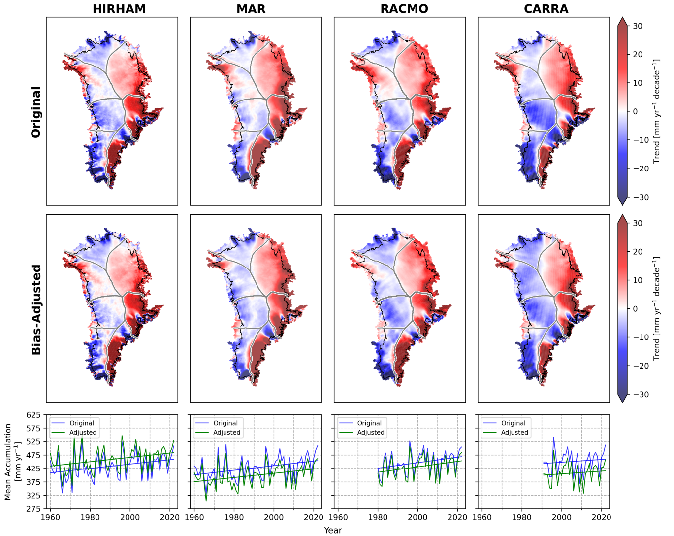
Figure 5. Temporal regressions before and after bias-adjustment. Upper: grid-point-wise regression for the 1991-2022 fitting period, representing spatial variation in linear trends. Lower: mean annual accumulation over the ice sheet with linear fits for HIRHAM (1960-2022), MAR (1960-2022), RACMO (1980-2022) and CARRA (1991-2022).
