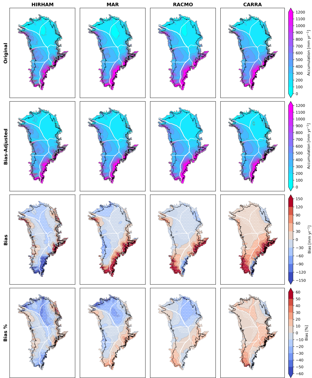
Figure 3. Mean maps Spatial patterns of of model mean accumulation and bias over over the 1991-2022 common period . The black line indicates the boundary of the accumulation zone. First row: original mean model accumulation before bias adjustment. Second row: bias-corrected mean accumulation. Third row: mean net bias in ( \text{mm yr}^{-1} , \text{mean}(\text{original} - \text{bias-adjusted}) , (\text{original} - \text{adjusted}) . Fourth row: mean relative bias, calculated by (eq. 11). Hatched regions indicate statistically significant biases ( p < 0.05 ) . The black line indicates the accumulation zone boundary, and white lines show PROMICE drainage basin boundaries are shown in white . Maps for the full model periods are provided in the appendix, Fig. A4.
