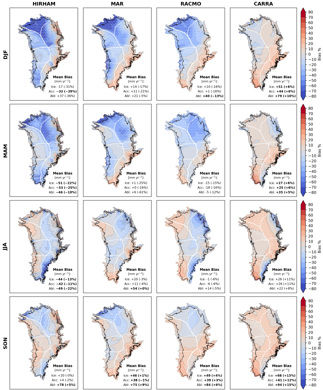
Figure 4. Model mean seasonal relative bias over the 1991-2022 common period: \text{mean}_{\text{season}} = \frac{\text{original} - \text{bias-adjusted}}{\text{original}} (eq. 11) for each season. Hatched regions indicate statistically significant biases ( p < 0.05 ). Values stated in the lower-right corners represent the in-panel labels show seasonal mean bias for each season values over the ice-sheet (Ice), accumulation zone (Acc) and ablation zone (Abl), with statistically significant biases indicated in bold.
