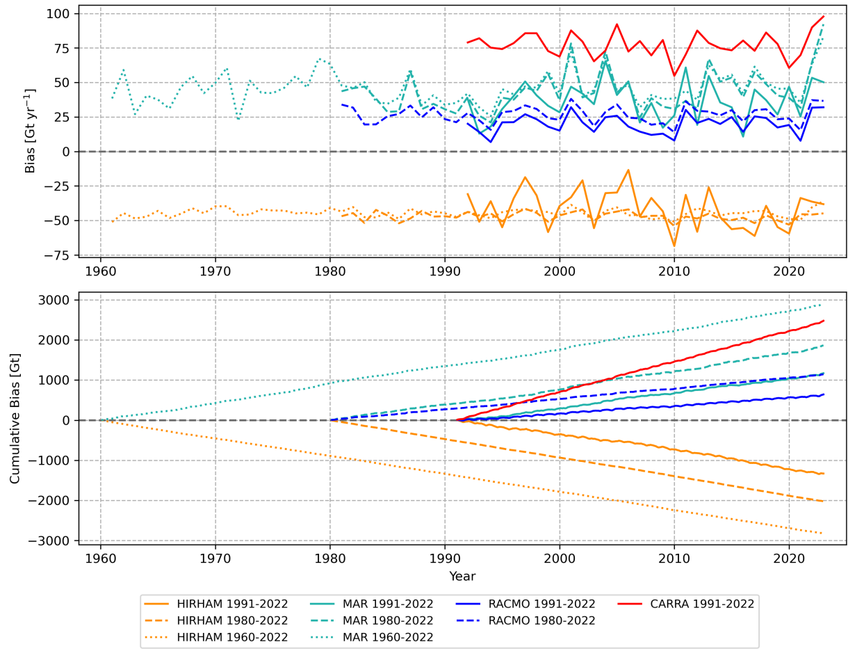
Figure A6. Spatially integrated annual bias \text{Gt yr}^{-1} for each model over the 1960-2022, 1980-2022 and 1991-2022 fitting periods, shown by year (upper) and as the cumulative sum (lower), indicating the net effect of the adjustment through time.
