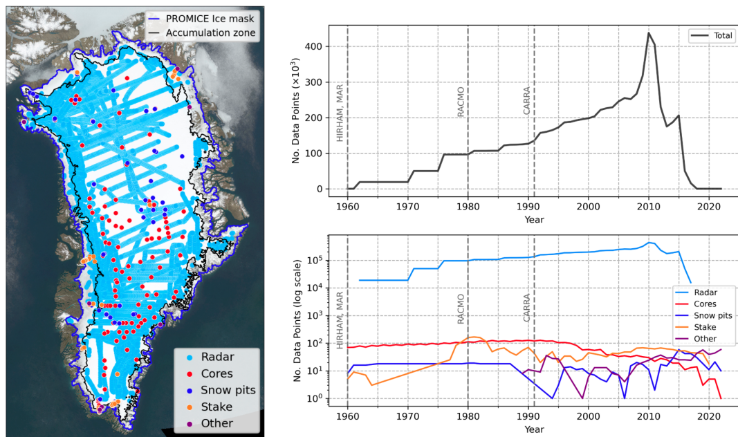
Figure 1. Left: geographical distribution of SUMup data points used in this study between 1960 and 2022, illustrated by measurement type. The method type ‘other’ includes mass balance profiles and SnowFox sensors. Right upper: time dependence of total number of data points with markers for the start year of model data. Right lower: time dependence of data points by measurement type, with counts in log scale.
