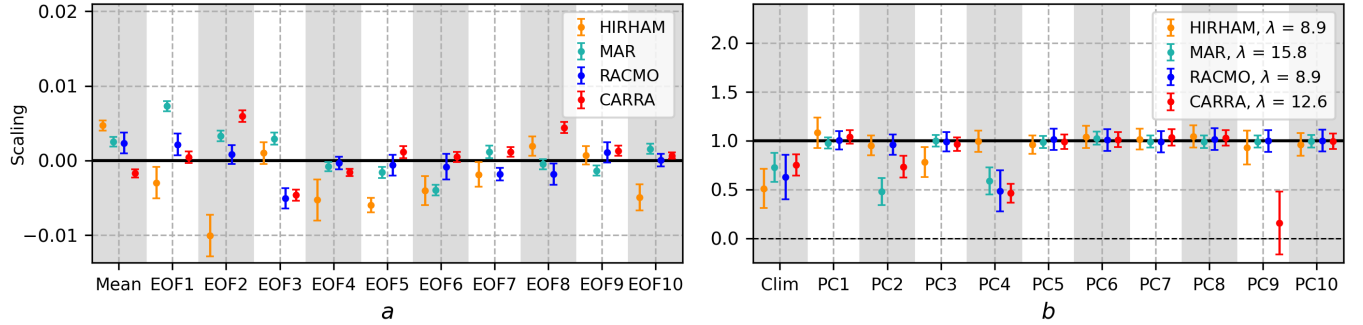
Figure 2. Bias-adjustment coefficients derived from fitting the 1991-2022 overlap period using the arctan loss function. Error bars represent the uncertainty in the parameter estimates, reflecting the confidence in the fitted coefficients rather than spatial variability. The initial guess (no adjustment) is denoted by the solid black line. Left: a parameters adjusting the time-independent mean bias and 10 EOF modes. Right: b parameters adjusting the time-dependent climatology and 10 PC modes, with \lambda values derived independently for each model via cross-validation.
