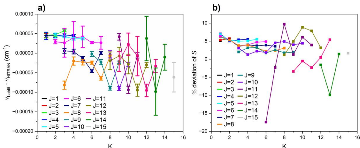
Figure 4. (a) Differences between the measured line positions and those from HITRAN 2020 (Gordon et al., 2021) for the NH 3 \nu_2(a) \leftarrow 0(s) Q branch lines, and (b) percentage deviations in intensity between the measured line intensities and those from HITRAN 2020 for the NH 3 \nu_2(a) \leftarrow 0(s) Q branch lines. For both cases, only lines with line intensity > 1 \times 10^{-21} \text{ cm}^{-1} / (\text{molecule cm}^{-2}) are plotted, and the error bars are 3\sigma .
