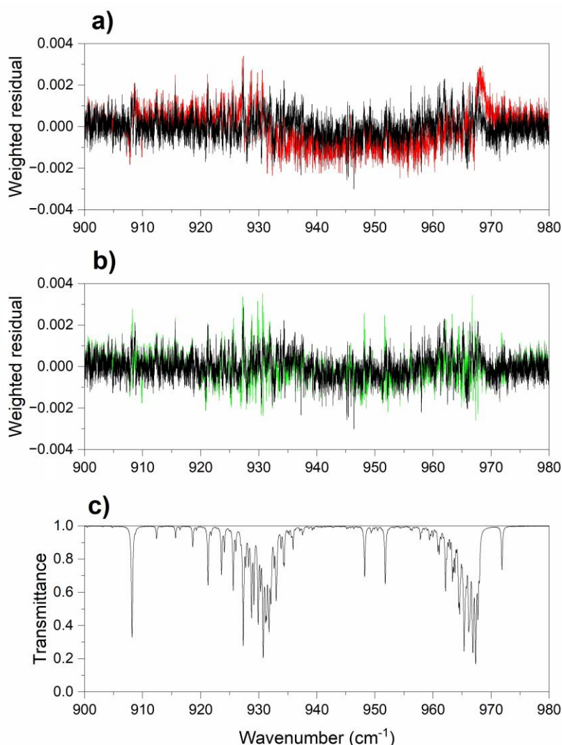
Figure 11. Comparison plots over the spectral region containing the \nu_2 Q branches (900-980 \text{cm}^{-1} ) of the weighted fit residuals for the measured highest-pressure spectrum (total pressure 978.3 hPa): (a) with (black) and without (red) the inclusion of Rosenkranz line mixing; (b) with (black) and without (green) the inclusion of speed dependence; (c) shows the measured laboratory transmittance spectrum.
