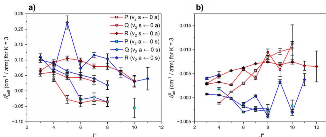
Figure 8. Plots of (a) self-pressure-induced shifts, \delta_{self}^0 , and (b) air-pressure-induced shifts, \delta_{air}^0 , against J'' for K = 3 , for the P, Q and R branches of the \nu_2(s) \leftarrow 0(a) and \nu_2(a) \leftarrow 0(s) transitions. The present measured values are given with uncertainties of 3\sigma . The HITRAN 2020 database does not include values for these parameters in this band.
