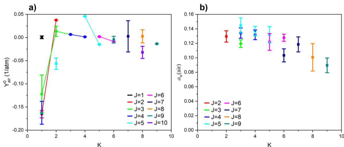
445 Figure 10. Plots of (a) Rosenkranz line mixing parameter, Y^0_{air} , and (b) speed dependence of the halfwidth parameter, a_w(air) , against K for each J value of the \nu_2(a) \leftarrow 0(s) Q branch. The present measured values are shown with uncertainties of 3\sigma . The HITRAN 2020 database does not include values for these line parameters of \text{NH}_3 .
