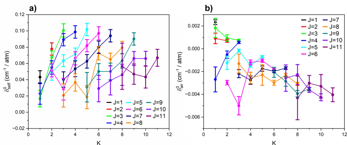
Figure 7. Plots of (a) self-pressure-induced shifts, \delta_{self}^0 , and (b) air-pressure-induced shifts, \delta_{air}^0 , against K for each J value of the \nu_2(a) \leftarrow 0(s) Q branch. Measured values are plotted with uncertainties of 3\sigma . The HITRAN 2020 database does not include values for these parameters.
