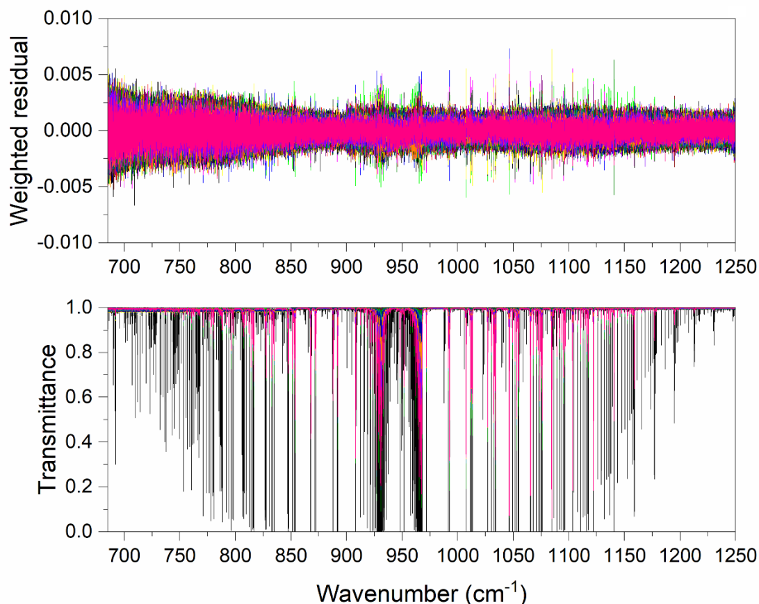
220 Figure 2: Overlay of all the transmittance spectra across the entire measured spectral region, 685-1250 \text{cm}^{-1} , alongside their weighted fit residuals, defined as the difference between the observed and calculated spectra.
