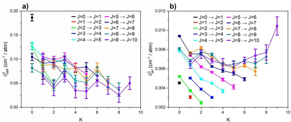
Figure S27. Plots of (a) self-pressure-induced shifts, \delta_{self}^0 , and (b) air-pressure-induced shifts, \delta_{air}^0 , against K for each J value of the \nu_2(s) \leftarrow 0(a) R branch. Measured values are plotted with uncertainties of 3\sigma . The HITRAN 2020 database does not include values for these parameters.
