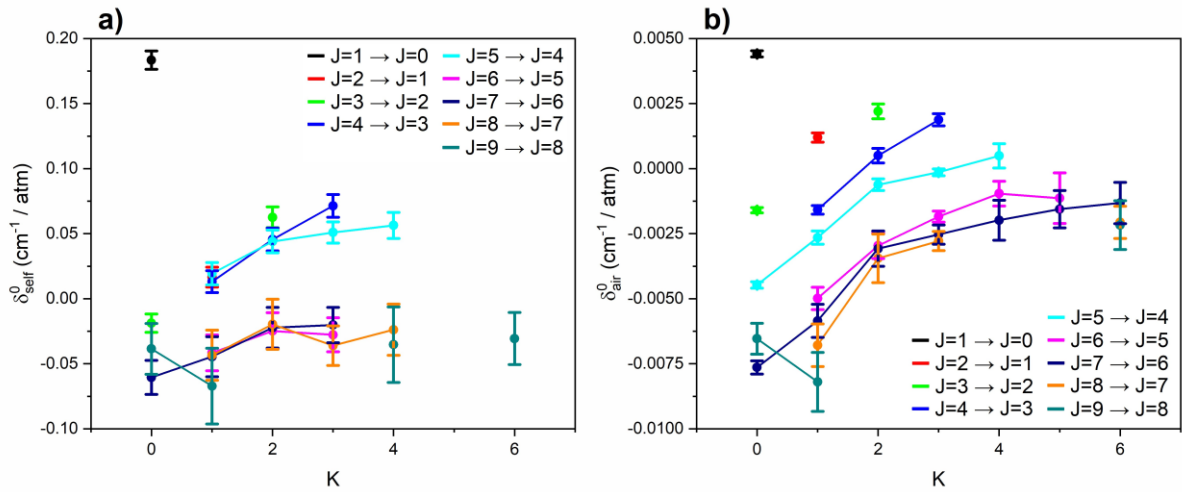
Figure S12. Plots of (a) self-pressure-induced shifts, \delta_{self}^0 , and (b) air-pressure-induced shifts, \delta_{air}^0 , against K for each J value of the \nu_2(a) \leftarrow 0(s) P branch. Measured values are plotted with uncertainties of 3\sigma . The HITRAN 2020 database does not include values for these parameters.
