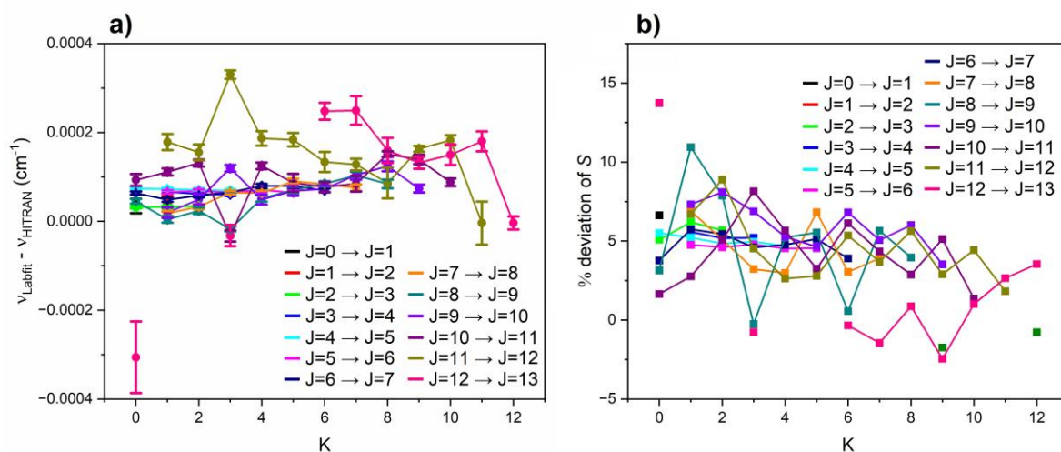
Figure S24. (a) Differences between the measured line positions and those from HITRAN 2020 for the \text{NH}_3 \nu_2(s) \leftarrow 0(a) R branch lines, and (b) percentage deviations in intensity between the measured line intensities and those from HITRAN 2020 for the \text{NH}_3 \nu_2(s) \leftarrow 0(a) R branch lines. For both cases, only lines with line intensity > 1 \times 10^{-21} \text{ cm}^{-1} / (\text{molecule cm}^{-2}) are plotted, and the error bars are 3\sigma .
