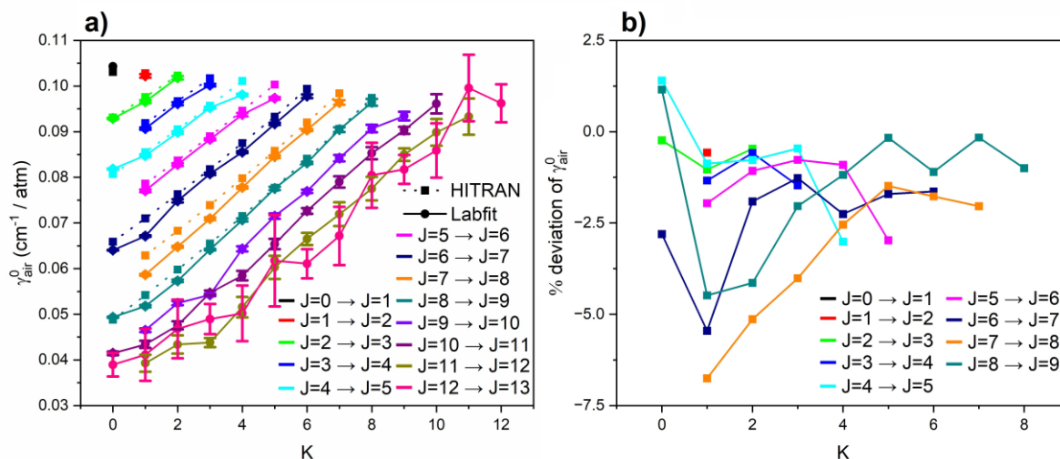
Figure S26. Plots of (a) air-broadened halfwidth, \gamma_{air}^0 , and (b) percentage deviations from HITRAN of \gamma_{air}^0 plotted against K for each J value of the \nu_2(s) \leftarrow 0(a) R branch. The Labfit values are included with uncertainties of 3\sigma . For J'' > 8 , HITRAN values for the air-broadened halfwidth were set to the same value as their corresponding K value at J'' = 8 (with values of K > 8 set to the value for K = 8 ), so percentage deviations have not been calculated for these cases.
