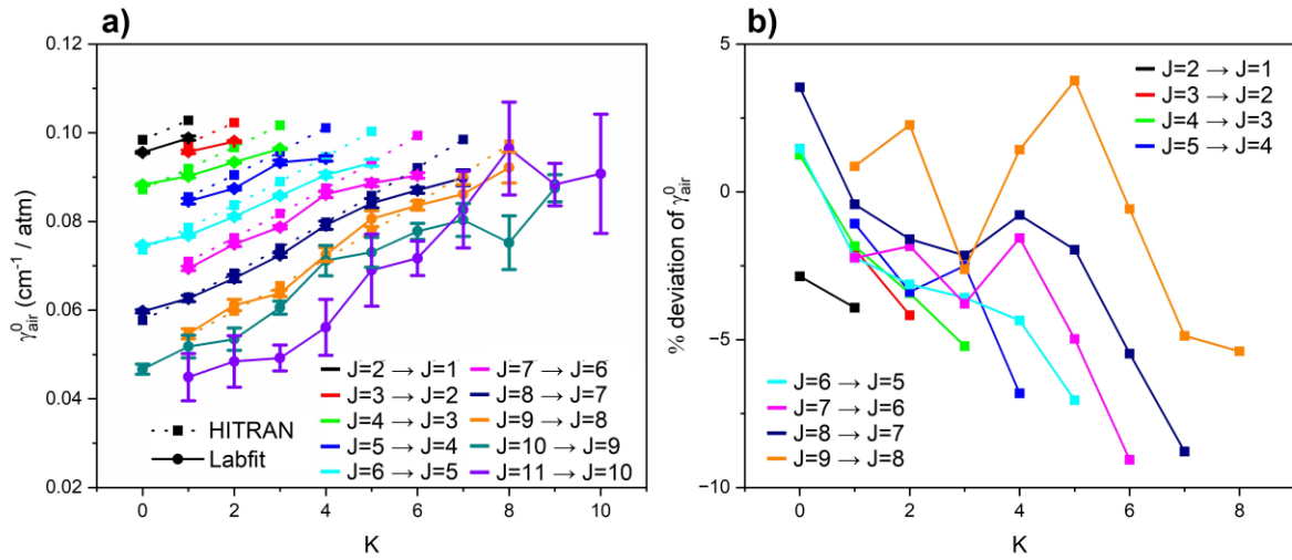
Figure S16. Plots of (a) air-broadened halfwidth, \gamma_{air}^0 , and (b) percentage deviations from HITRAN of \gamma_{air}^0 plotted against K for each J value of the \nu_2(s) \leftarrow 0(a) P branch. The Labfit values are included with uncertainties of 3\sigma . For J'' > 9 , HITRAN values for the air-broadened halfwidth were set to the same value as their corresponding K value at J'' = 9 (with values of K > 9 set to the value for K = 9), so percentage deviations have not been calculated for these cases.
