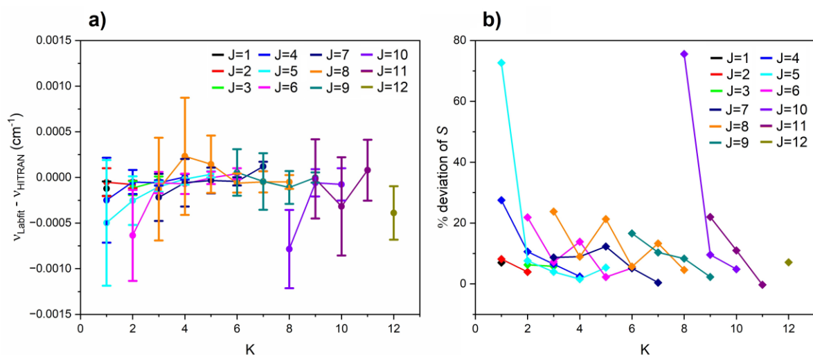
Figure S29. (a) Differences between the measured line positions and those from HITRAN 2020 for the ^{15}\text{NH}_3 \nu_2(a) \leftarrow 0(s) Q branch lines, and (b) percentage deviations in intensity between the measured line intensities and those from HITRAN 2020 for the ^{15}\text{NH}_3 \nu_2(a) \leftarrow 0(s) Q branch lines. For both cases, the error bars are 3\sigma .
