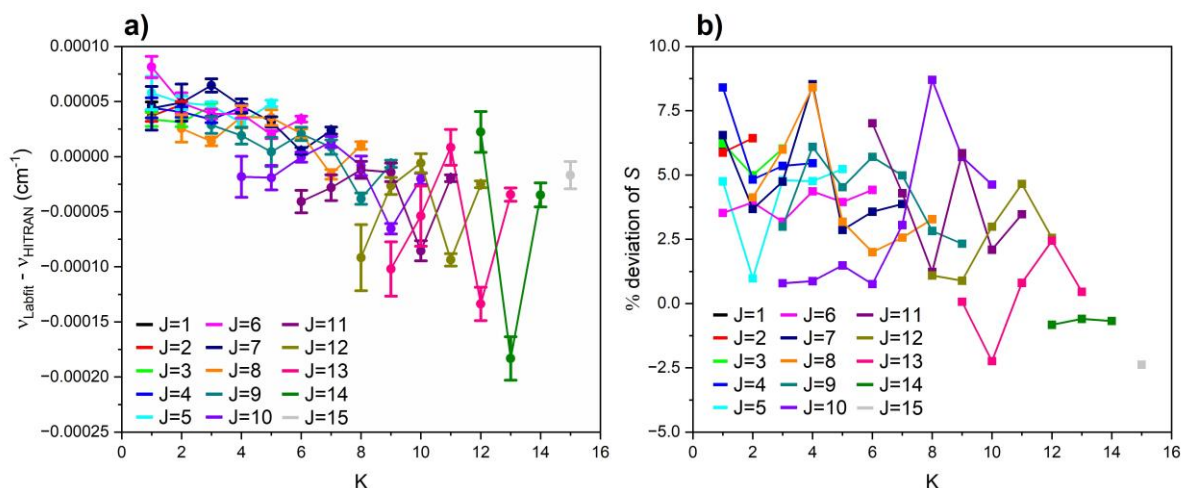
Figure S3. (a) Differences between the measured line positions and those from HITRAN 2020 for the \text{NH}_3 \nu_2(s) \leftarrow 0(a) Q branch lines, and (b) percentage deviations in intensity between the measured line intensities and those from HITRAN 2020 for the \text{NH}_3 \nu_2(s) \leftarrow 0(a) Q branch lines. For both cases, only lines with line intensity > 1 \times 10^{-21} \text{ cm}^{-1} / (\text{molecule cm}^{-2}) are plotted, and the error bars are 3\sigma .
