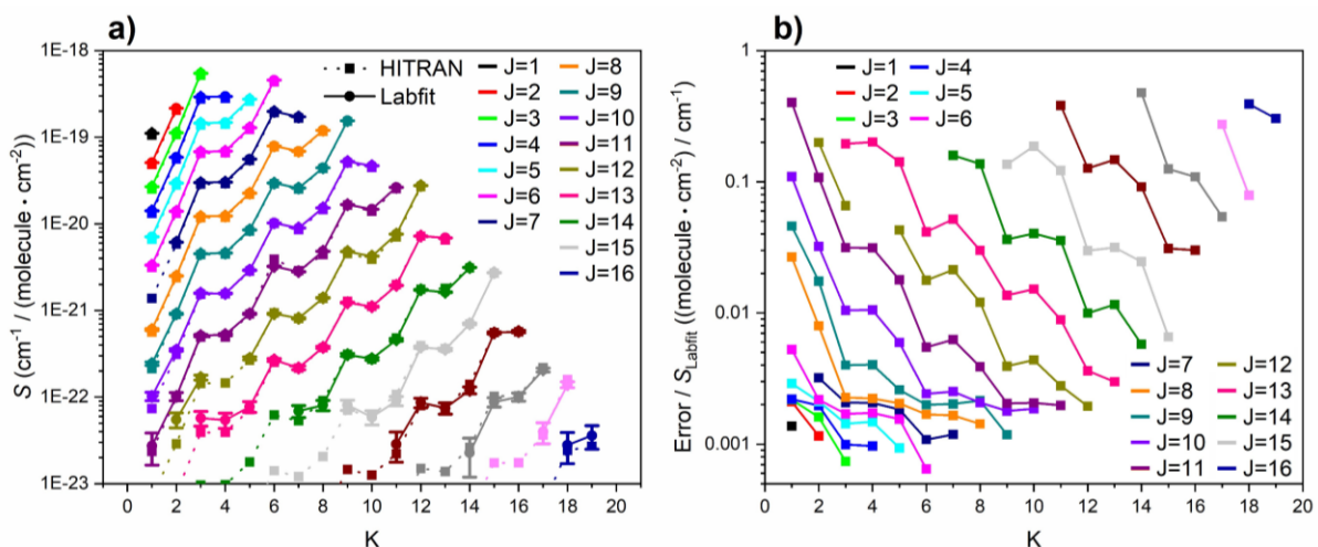
Figure S1. Plots of (a) spectral line intensity S , with Labfit value uncertainties of 3\sigma , and (b) 3\sigma uncertainty divided by Labfit line intensity S_{\text{Labfit}} plotted against K for each J value of the \text{NH}_3 \nu_2(a) \leftarrow 0(s) Q branch.
