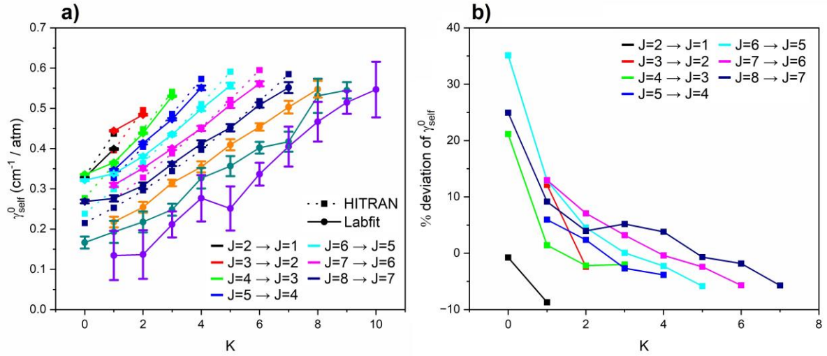
Figure S15. Plots of (a) self-broadened halfwidth, \gamma_{self}^0 , and (b) percentage deviations from HITRAN of \gamma_{self}^0 plotted against K for each J value of the \nu_2(s) \leftarrow 0(a) P branch. The Labfit values are included with uncertainties of 3\sigma . For J'' > 8 , HITRAN values for the self-broadened halfwidth were all set to 0.5, so percentage deviations have not been calculated for these cases.
