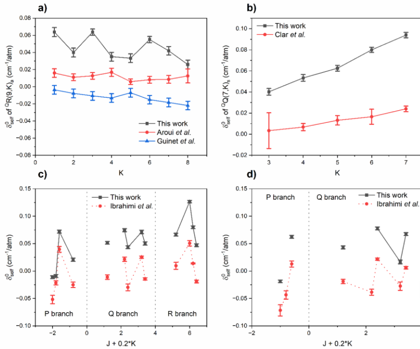
Figure 9. Comparison plots of self-pressure-induced shifts, \delta_{self}^0 , from our work and other papers, against K, for (a) the R branch of the \nu_2(s) \leftarrow 0(a) transition, where J=9 ; (b) the Q branch of the \nu_2(a) \leftarrow 0(s) transition, where J=7 ; (c) the P, Q and R branches of the \nu_2(s) \leftarrow 0(a) transition; (d) the P and Q branches of the \nu_2(a) \leftarrow 0(s) transition. Unlike other plots, uncertainties are plotted here as 1\sigma to better compare with the previous studies. The HITRAN 2020 database does not include values for these parameters in this band.
