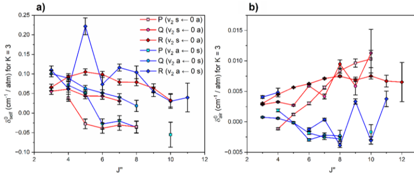
Figure 8. Plots of (a) self-pressure-induced shifts, \delta_{self}^0 , and (b) air-pressure-induced shifts, \delta_{air}^0 , against J'' for K=3 , for the P, Q and R branches of the v_2(s) \leftarrow 0(a) and v_2(a) \leftarrow 0(s) transitions. The present measured values are given with uncertainties of 3\sigma . The HITRAN 2020 database does not include values for these parameters in this band.
