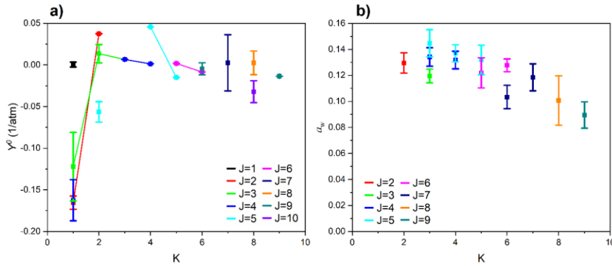
455 Figure 10. Plots of (a) Rosenkranz line mixing parameter, Y^0_{air} , and (b) speed dependence of the halfwidth parameter, a_w(air) , against K for each J value of the v_2(a) \leftarrow 0(s) Q branch. The present measured values are shown with uncertainties of 3\sigma . The HITRAN 2020 database does not include values for these line parameters of NH_3 .
