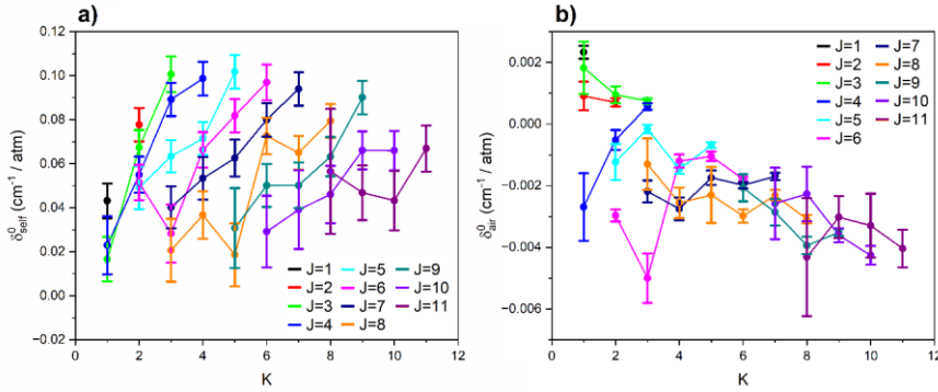
Figure 7. Plots of (a) self-pressure-induced shifts, \delta_{self}^0 , and (b) air-pressure-induced shifts, \delta_{air}^0 , against K for each J value of the \nu_2(a) \leftarrow 0(s) Q branch. Measured values are plotted with uncertainties of 3\sigma . The HITRAN 2020 database does not include values for these parameters.
