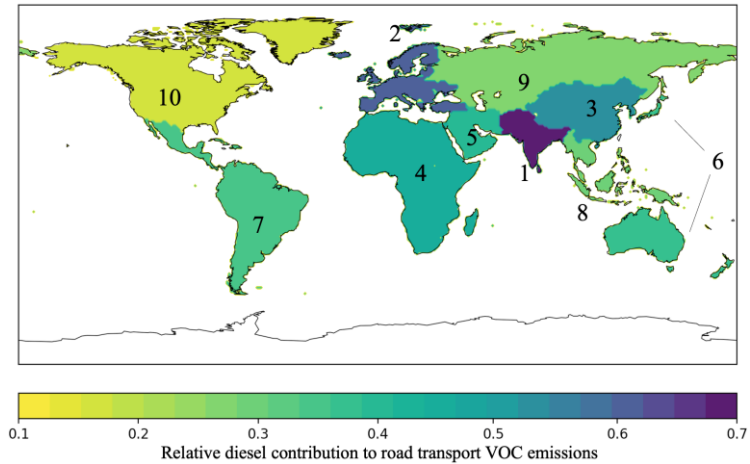
840 Figure 3: Global diesel share of VOC emissions in 10 subcontinents. The numbers correspond to the subcontinent names in Table 2.
