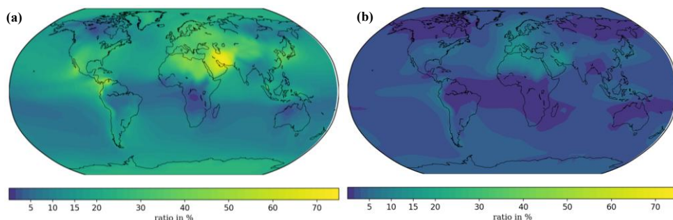
Figure 1110: Ratio of modelled SOA-iv from the road transport sector to SOA-iv from all sectors as simulated by the (a) ORACLE-IVOC and (b) ORACLE-base, averaged over the years 2011–2020.
