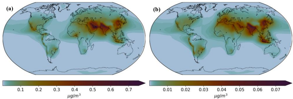
Figure 76: Modelled surface concentration of SOA-iv from the road transport sector for the years 2011 – 2020 by using (a) the ORACLE-IVOC model and (b) the ORACLE-base model.
