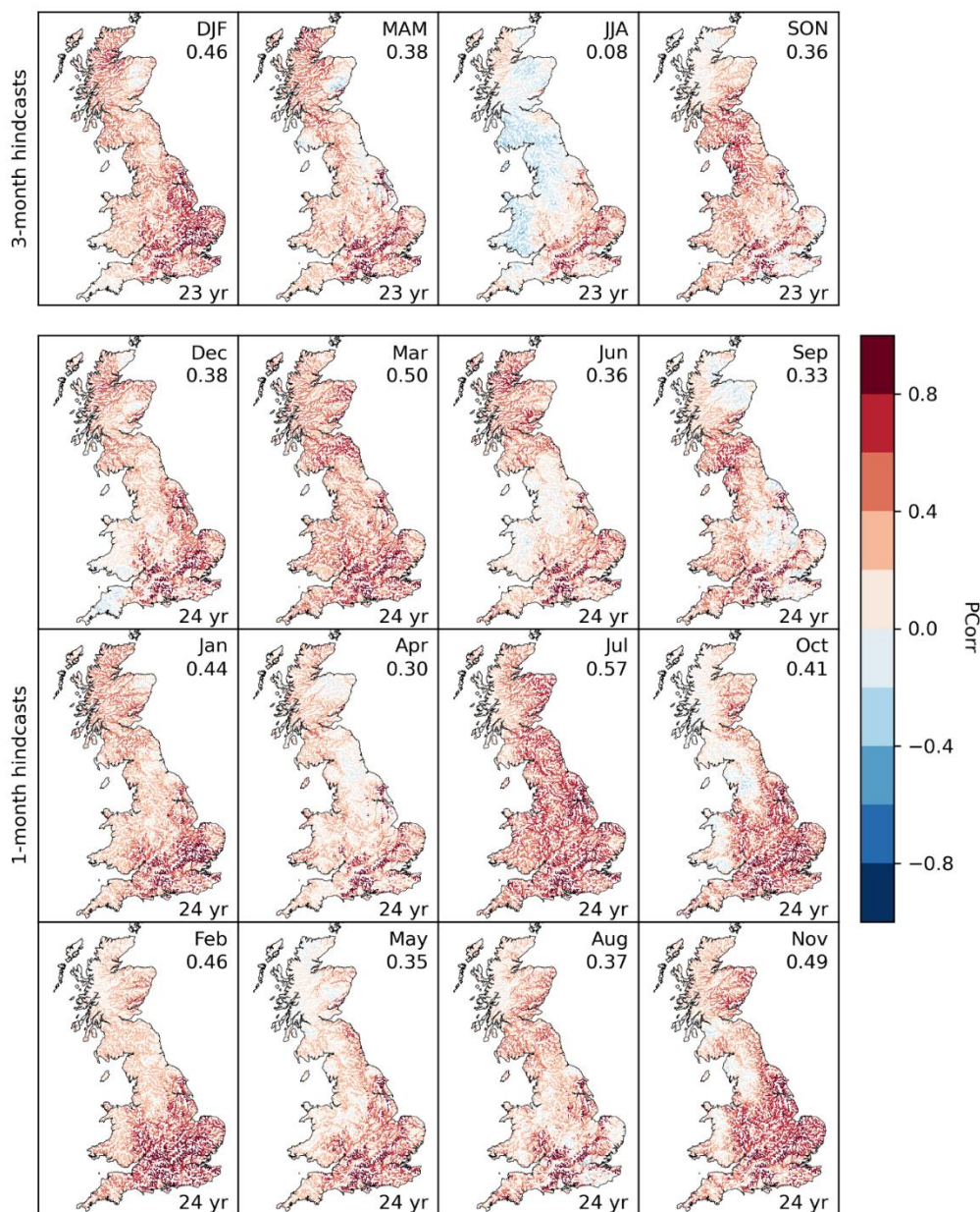
425 Figure 4: Pearson correlation between G2G/WBM forecast ensemble mean and 'ground truth' river flows for 3-month (top row) and 1-month (bottom three rows) hindcasts. A positive correlation is indicated in red while a negative correlation is in blue. In each panel the number in the top-right corner is the spatial mean while the number of hindcasts used to calculate the correlation is in the bottom-right corner.
