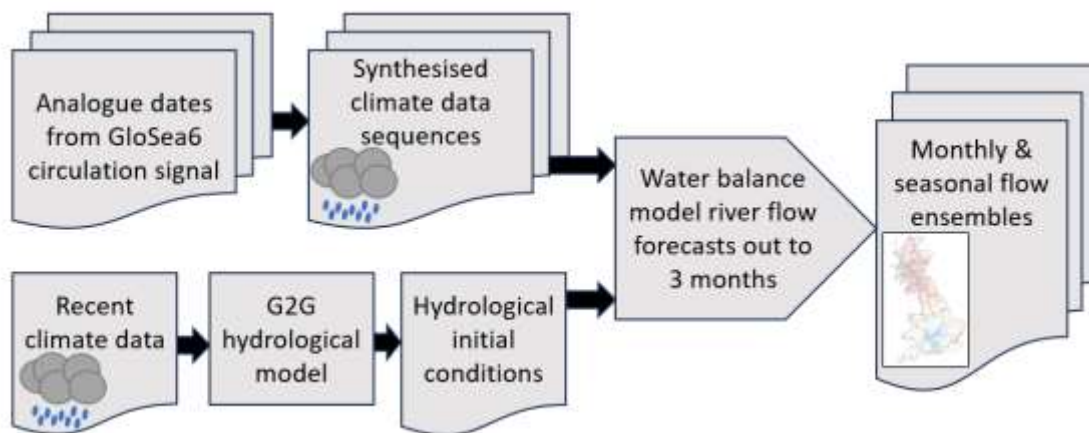
110 Figure 1: Schematic of the G2G/WBM hydrological forecasting scheme, here driven by rainfall forecasts derived from Historic Weather Analogues.
