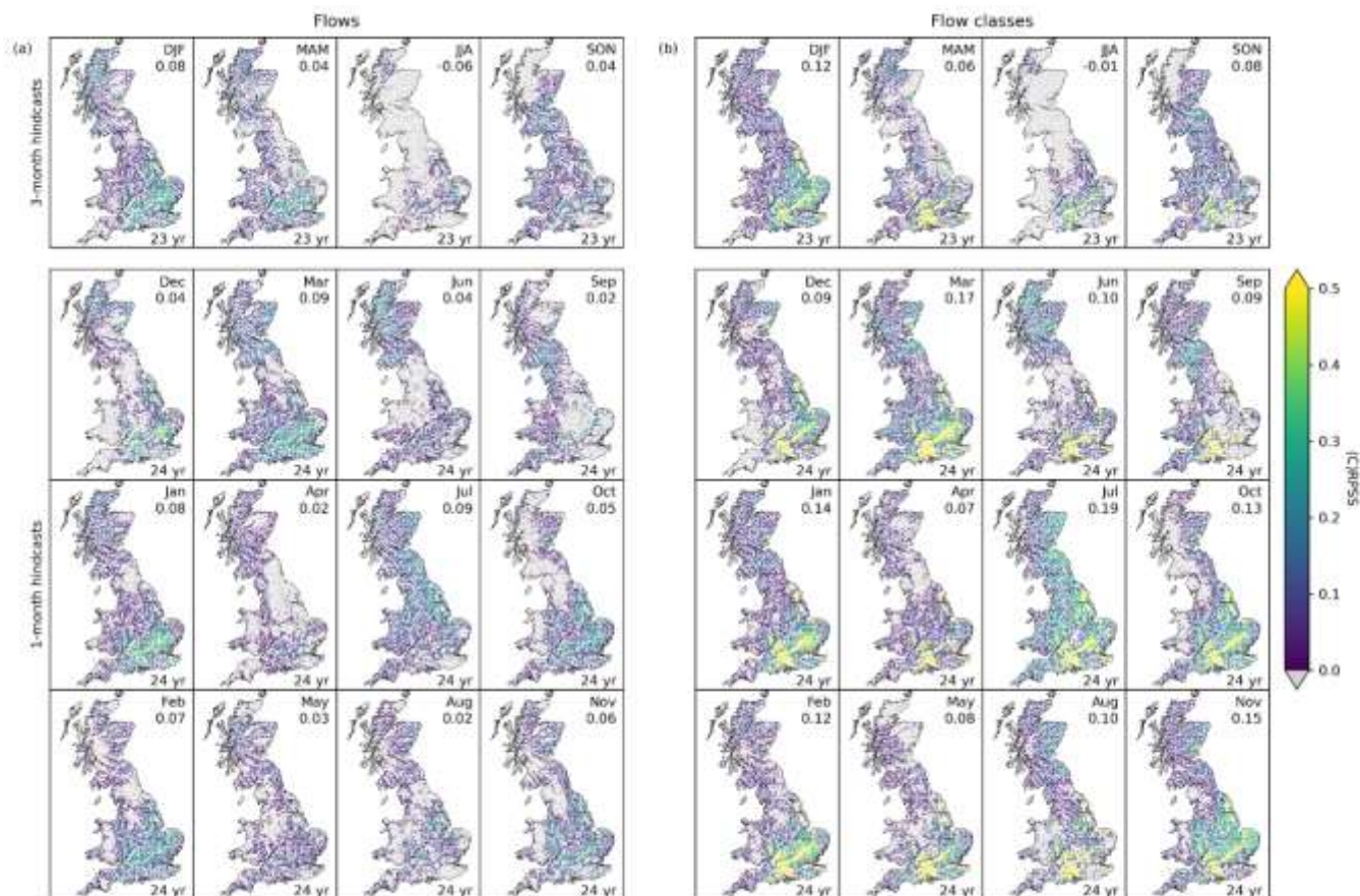
410 Figure 4: The skill of the G2G/WBM river flow forecasting scheme over assuming the climatological distribution. Left: CRPSS for predicting volumetric river flows (m3/s). Right: RPSS for predicting classified flows (Table 1). Scores greater than 0 (coloured) indicate the G2G/WBM scheme outperforms the climatological distribution, while those less than zero (grey) indicate the converse. The spatial mean is shown in the top-right of each panel, with the number of hindcasts in the bottom-right.
