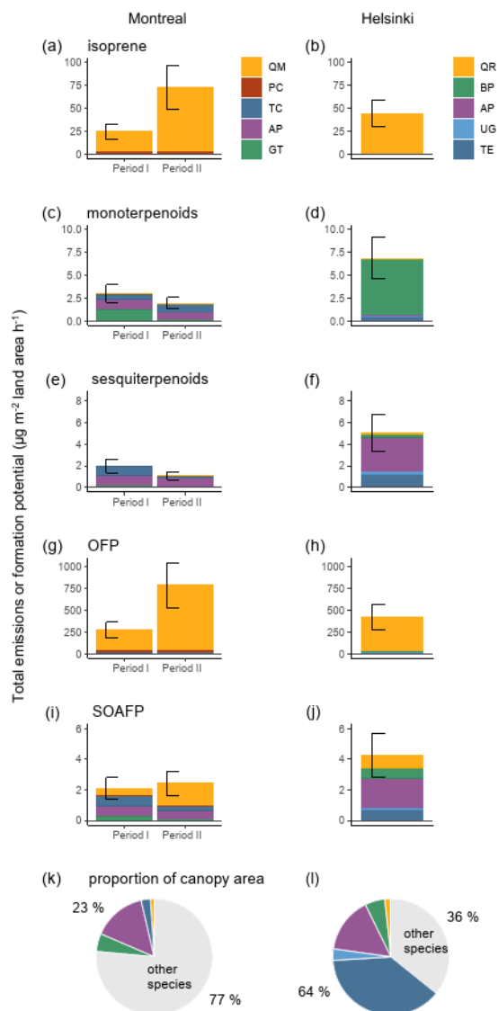
455 Figure 6. Upscaled total emission potential per land area for isoprene (a–b), monoterpenes (c–d), and sesquiterpenoids (e–f), as well as for their O 3 formation potential (OFP, g–h) and SOA-formation potential (SOAFP, i–j) of the study species within the upscaling test area in Montreal in June and August (periods I and II: a, c, e, g and i) and Helsinki in July 2022 (b, d, f, h and j). The BVOC emission, OFP, and SOAFP intensity estimates only include the individuals from our study species, whereby their proportions of the entire canopy area within the upscaling test areas are listed for Montreal (k) and Helsinki (l). The vertical brackets show the 460 estimated total emissions or formation potentials without correction for shading (upper limit) and a stronger correction for shading (lower limit).
