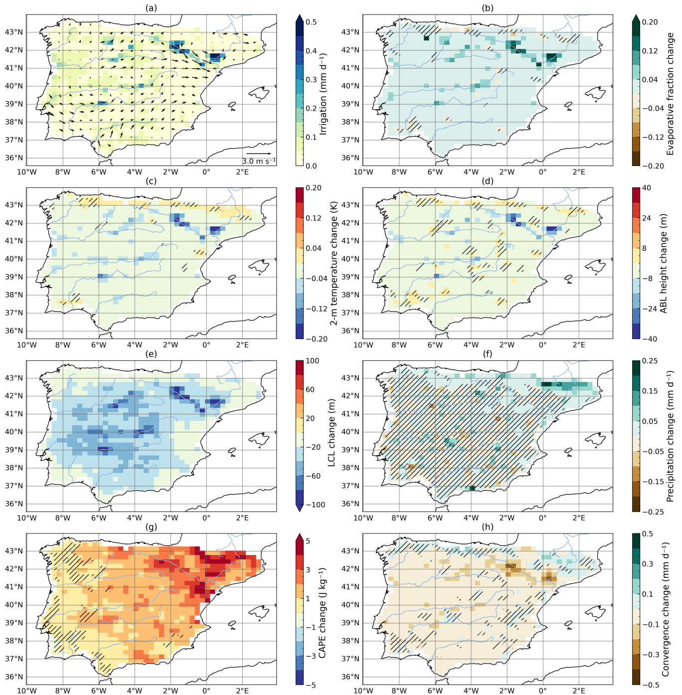
Figure G3. Autumn irrigation and its impacts (SON, 2010-2022). (a) Irrigation ( \text{mm d}^{-1} ) and 10 m wind ( irr simulation). Mean changes in the presence of irrigation ( irr - no_irr ): (b) evaporative fraction, (c) 2 m temperature (K), (d) atmospheric boundary layer height (m), (e) lifting condensation level (m), (f) precipitation ( \text{mm d}^{-1} ), (g) convective available potential energy ( \text{J kg}^{-1} ), (h) moisture convergence ( \text{mm d}^{-1} ). Hatching indicates areas where the change is not statistically significant.
