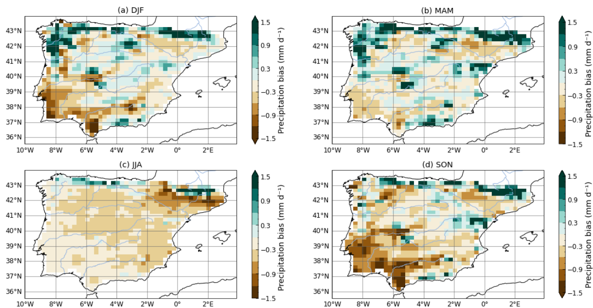
Figure D1. Seasonal mean biases of precipitation (mm d -1 ) in the no_irr simulation compared with the GPCP product (2010-2019).
