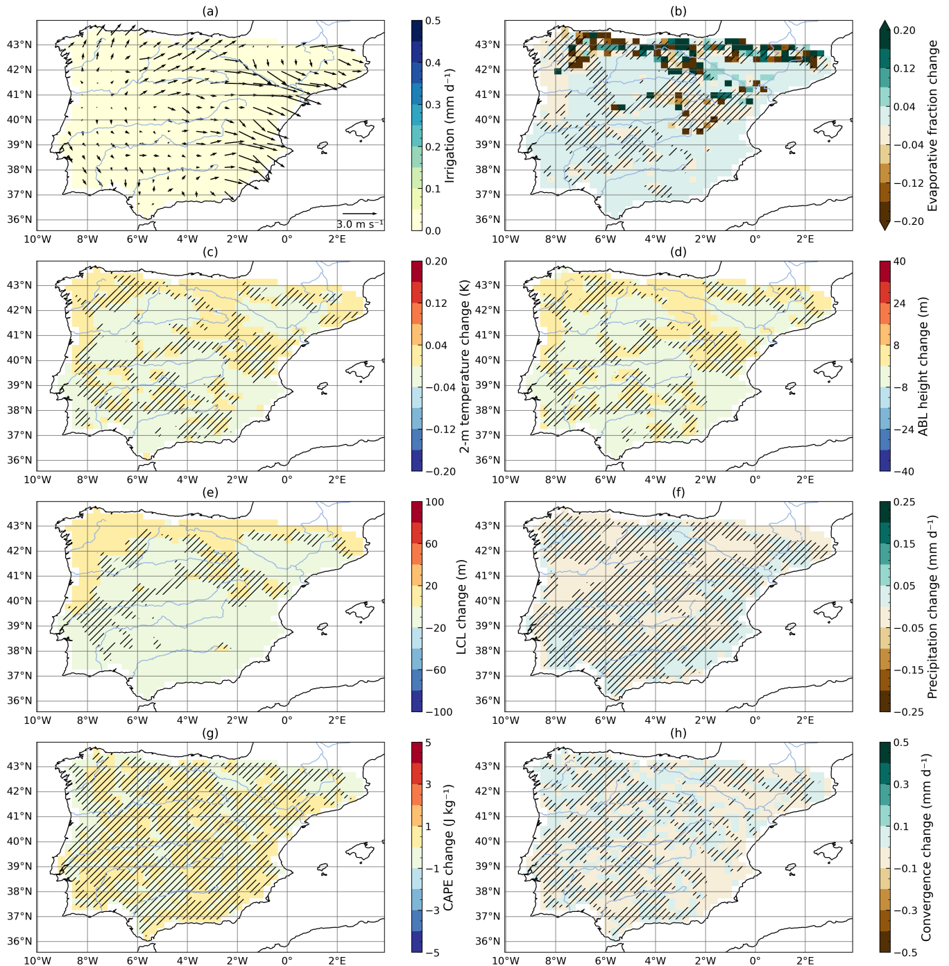
Figure G1. Winter irrigation and its impacts (DJF, 2010-2022). (a) Irrigation ( \text{mm d}^{-1} ) and 10 m wind ( irr simulation). Mean changes in the presence of irrigation ( irr - no_irr ): (b) evaporative fraction, (c) 2 m temperature (K), (d) atmospheric boundary layer height (m), (e) lifting condensation level (m), (f) precipitation ( \text{mm d}^{-1} ), (g) convective available potential energy ( \text{J kg}^{-1} ), (h) moisture convergence ( \text{mm d}^{-1} ). Hatching indicates areas where the change is not statistically significant.
