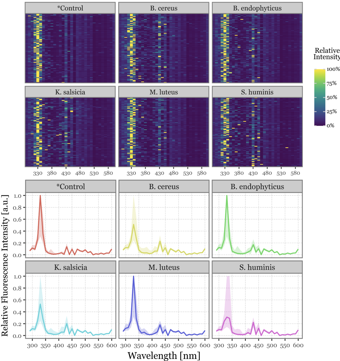
Figure 7. Fluorescence spectra for the aerosolized bacterial samples. In the top panel, heatmaps display the relative fluorescence intensity detected across all wavelengths within the detector's range for the top 100 most intensely fluorescent particles. The bottom panel shows the same data represented as line plots, with the solid line indicating the median value across all samples and the shaded area representing the interquartile range (25 th to 75 th percentiles).
