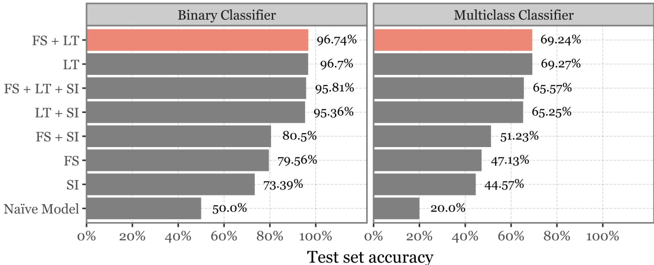
330 Figure 9. Evaluation of the predictor variables and model skill. Bar plot depicting the class-balanced accuracy of the best-performing model for each combination of model predictors (FS = Fluorescence Spectra, LT = Lifetimes, SI = Scattering Images) for both binary (left) and multiclass (right) classifiers. The bar corresponding to the overall best-performing model, which uses both Fluorescence Spectra and Lifetimes, is highlighted in red. The baseline performance of a naïve classifier, equivalent to a completely uninformed prediction is also included for reference.
