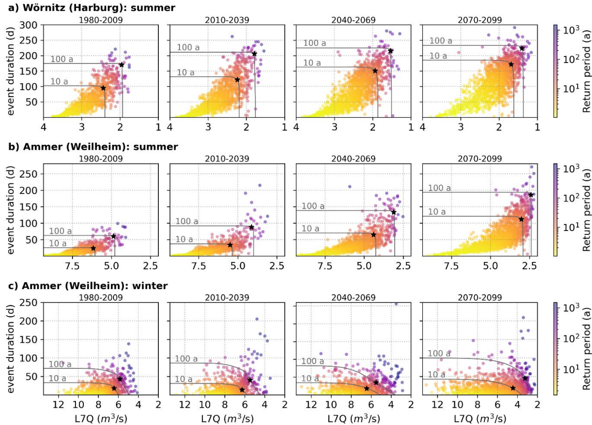
405 Figure 7: Bivariate survival Kendall's return levels of event duration and L7Q. The grey isolines show the 10-year and 100-year return levels, where the black star marker represents the most likely combination of L7Q and event duration for the respective bivariate return periods. For a direct visual comparison of the changes in the isolines between the time periods, Fig. S6 is provided.
