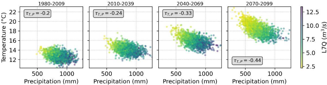
Figure 10: Bivariate scatter plots of summer (May to October) temperature and precipitation. The scatter plot shows one dot per year, adding up to a total of 1500 dots pooling the 50 members. The color scale connects the climatic conditions to the respective summer L7Q.
