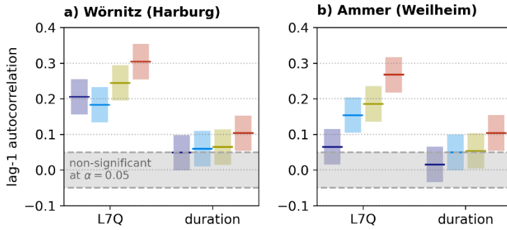
Figure 9: Lag-1-autocorrelation for L7Q and low flow duration in the summer half year for the (a) Wörnitz catchment and (b) Ammer catchment. The colours refer to the respective time periods as in the previous figures 2, 4, and 6. Per time period, all 50 members are pooled to a total of 1500 years. The lag relates to the previous summer half year. The coloured transparent ranges provide 95% confidence intervals for the autocorrelation, while the grey transparent range represents no significant autocorrelation ( \alpha = 0.05 ).
