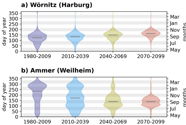
Figure 4: Seasonality of the annual L7Q events. The violin plots provide kernel density estimates, where the grey line shows the median of all events in the respective 30-year period. Per time period, all 30 years times 50 members are pooled, allowing the kernel density estimate to be based on 1500 years.
