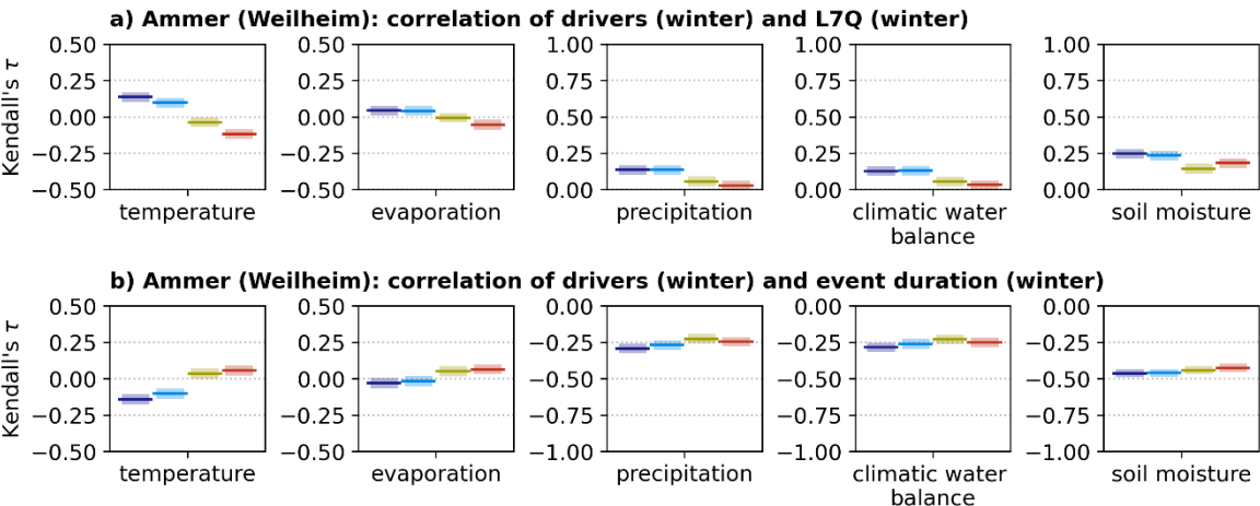
Figure 12: Kendall's rank correlation between winter climatic drivers and (a) winter low-flow intensity L7Q, as well as between winter climatic drivers and (b) winter low-flow event duration. The colours refer to the respective time periods as in the previous figures 2, 4, and 6. Per time period, all 50 members are pooled to a total of 1500 years. The transparent ranges provide 95% confidence intervals for Kendall's \tau .
