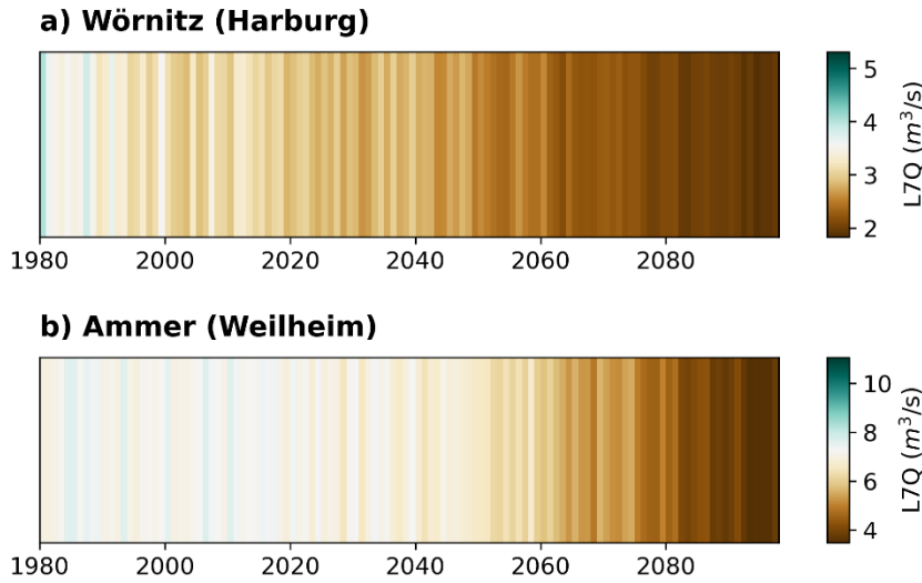
Figure 3: “Drying stripes” (inspired by the warming stripes by Hawkins, 2018): With the ML7Q of 1980 – 2009 as reference, the temporal course of the annual L7Q visualizes the projections of low flow intensity. Each annual stripe pools all 50 members and represents the median of these 50 years.
