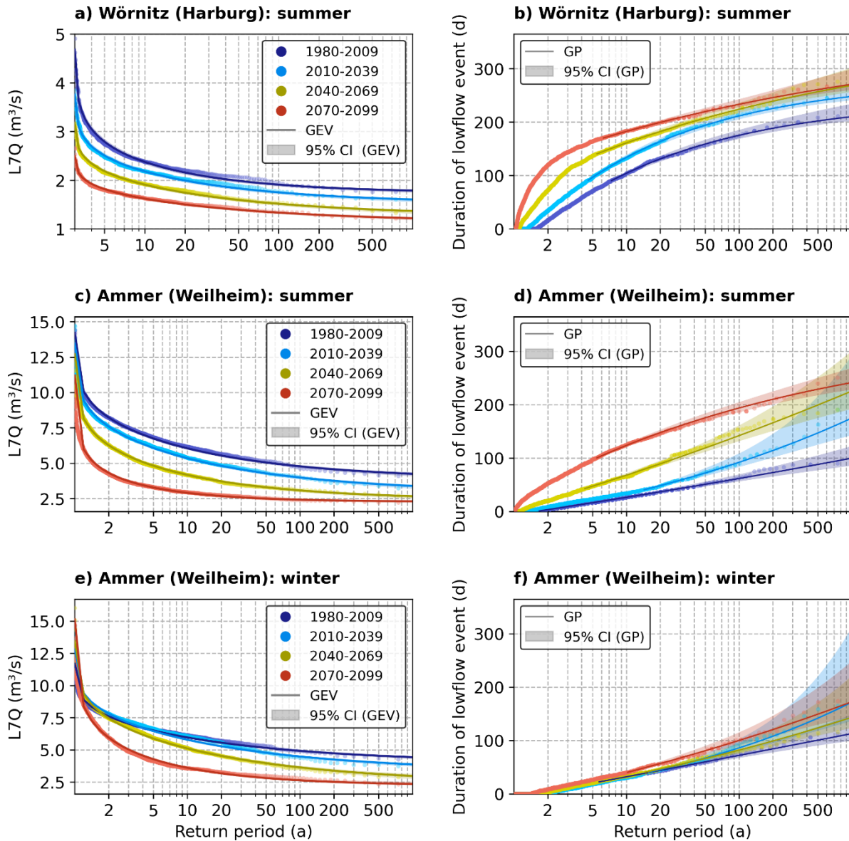
Figure 6: Univariate return levels of 7-day low-flow discharge peaks L7Q (a, c, e) and event duration (b, d, f) for both study catchments. Per time period, all 50 members are pooled to a total of 1500 years. The coloured dots are plotted via Weibull plotting positions.
