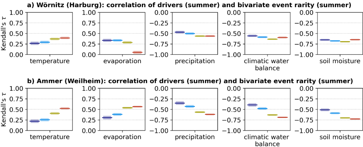
425 Figure 8: Rank correlation between climatic and hydrological drivers and the bivariate event rarity in the summer half year for the (a) Wörnitz catchment and (b) Ammer catchment. The colours refer to the respective time periods as in the previous figures 2, 4, and 6. Per time period, all 50 members are pooled to a total of 1500 years. Drivers are averaged over the summer half year. The climatic water balance is defined as precipitation minus potential evaporation. The transparent ranges provide 95% confidence intervals for Kendall's \tau .
