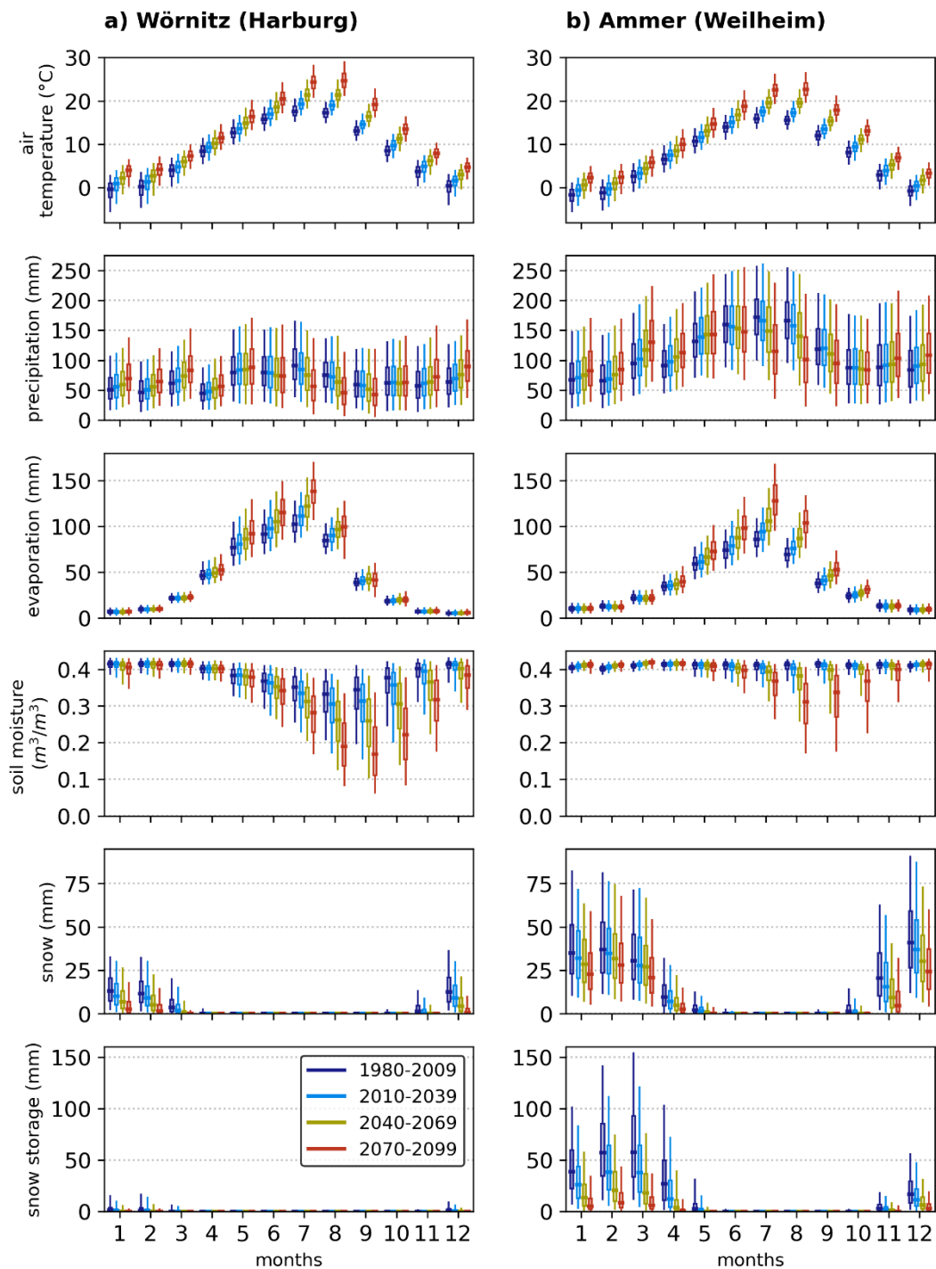
320 Figure 2: Climatic and hydrological drivers in the (a) Wörnitz and (b) Ammer catchments. The centerline of the boxplots shows the median over all 50 members and 30 years per period. The boxes represent the inter-quartile range of the 1500 years, where the
