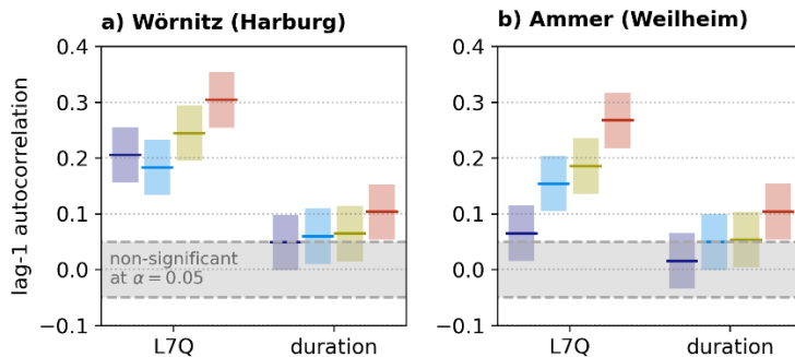
430 Figure 9: Lag-1-autocorrelation for L7Q and low flow duration in the summer half year for the (a) Wörnitz catchment and (b) Ammer catchment. The colours refer to the respective time periods as in the previous figures 2, 4, and 6. Per time period, all 50 members are pooled to a total of 1500 years. The lag relates to the previous summer half year. The coloured transparent ranges provide 95% confidence intervals for the autocorrelation, while the grey transparent range represents no significant autocorrelation ( \alpha = 0.05 ).
