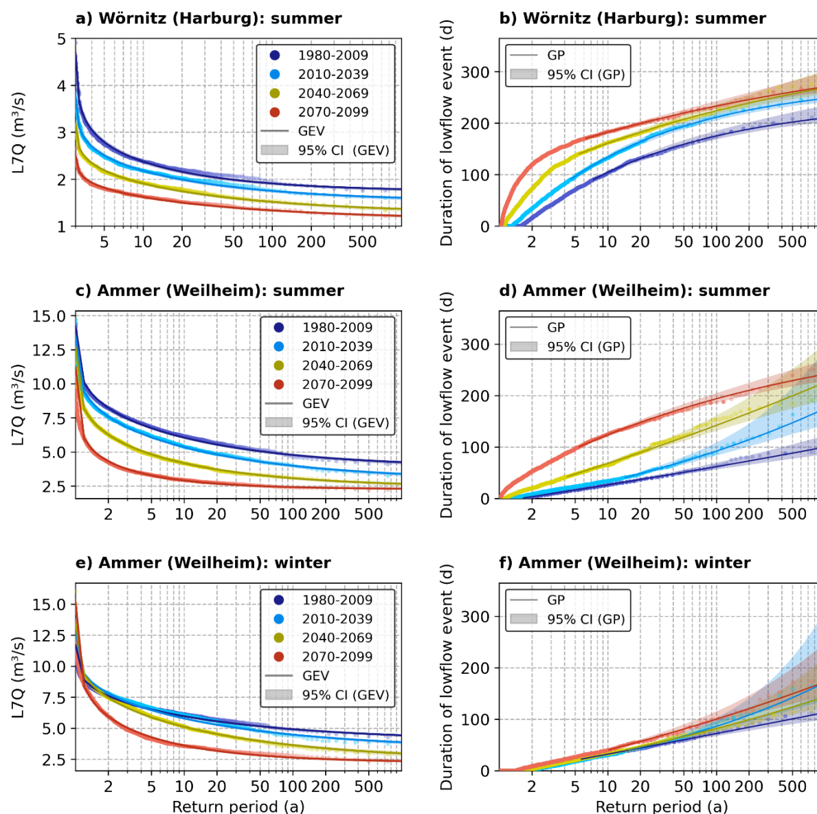
Figure 6: Univariate return levels of 7-day low-flow discharge peaks L7Q (a, c, e) and event duration (b, d, f) for both study
