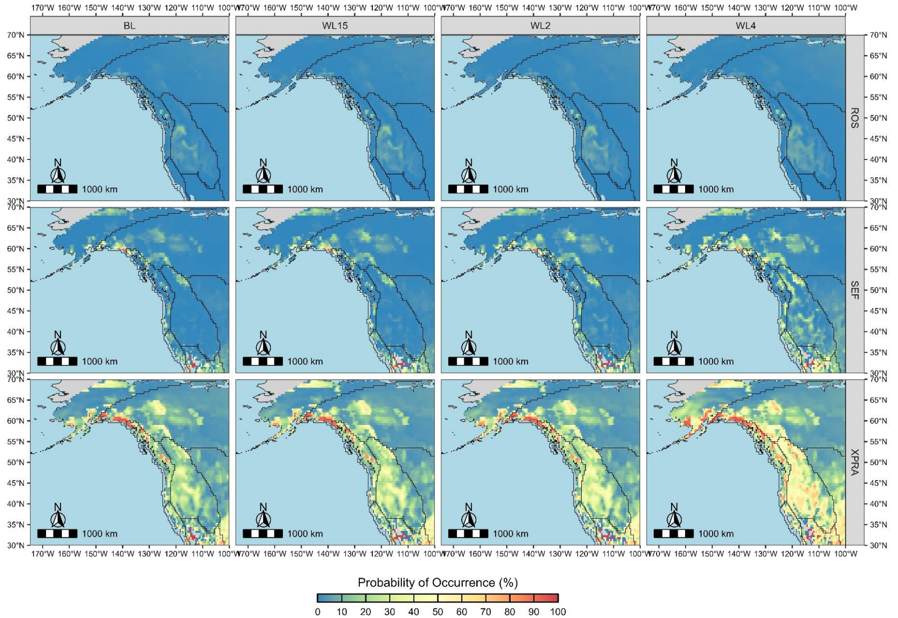
Figure S2. Spatial plot of probability of occurrence of ROS, SEF and XPRA events are occurring. Statistically significant results are represented by areas with stippling.
