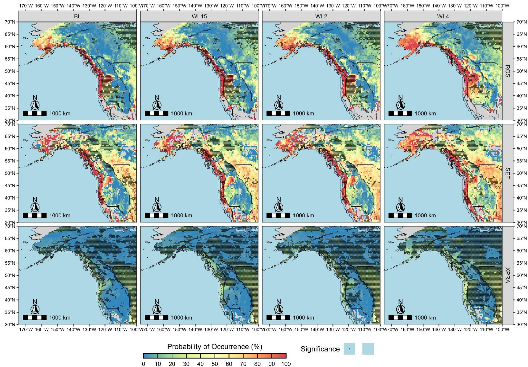
Figure S1. Spatial plot of probability of occurrence of an AR event given that ROS, SEF and XPRA events are occurring. Statistically significant results are represented by areas with stippling.
