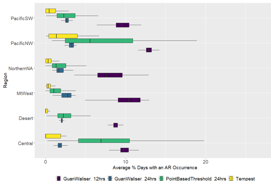
Figure 3: Average AR occurrence in the Baseline Period (1986-2016) expressed as the overall percentage of AR days detected in the 31-year period for ERA5. The distribution of days detected in each region in the current study is compared for the Guan and Waliser algorithm results represent ARs counted on a daily and sub daily scale.
