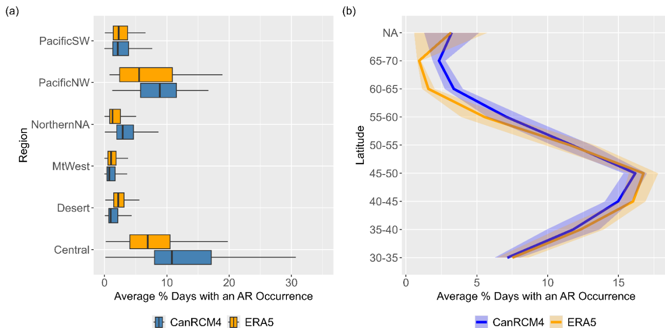
Figure 2: Average AR occurrence in the Baseline Period (1986-2016) expressed as the overall percentage of AR days detected in the 31-year period for CanRCM4 and ERA5 models. The distribution of days in each region is shown in a), while the latitudinal average for each model over the entire study area is summarized in b) with the average spread in the results.
