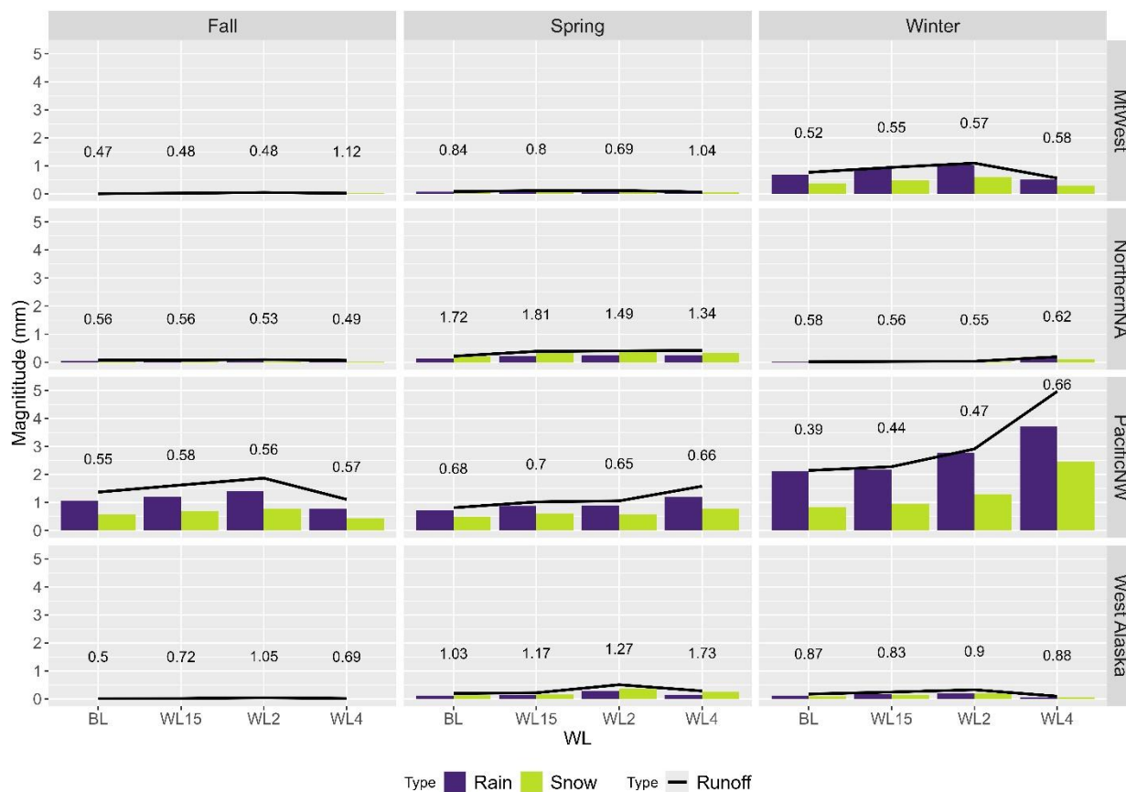
Figure 8: The spatial average of AR related ROS event magnitude expressed in terms of millimetres of runoff, rainfall and snowmelt generated on the day of the event for each season and region. The left, middle and right columns depict results from fall, spring, and winter respectively. From the top, the first, second, third and fourth rows depict the MtWest, NorthernNA, PacificNW and West Alaska regions respectively.
