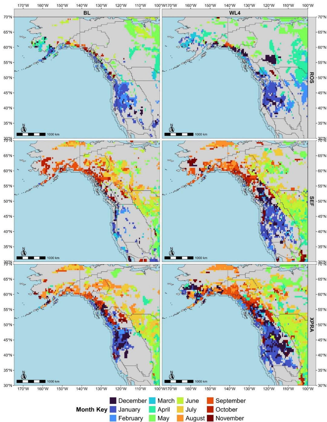
Figure 10: Spatial map showing the month with the highest ROS(top), SEF(middle) and XPRA(bottom) event magnitude in terms of runoff for each cell in the BL(left) and WL4(right) periods.
