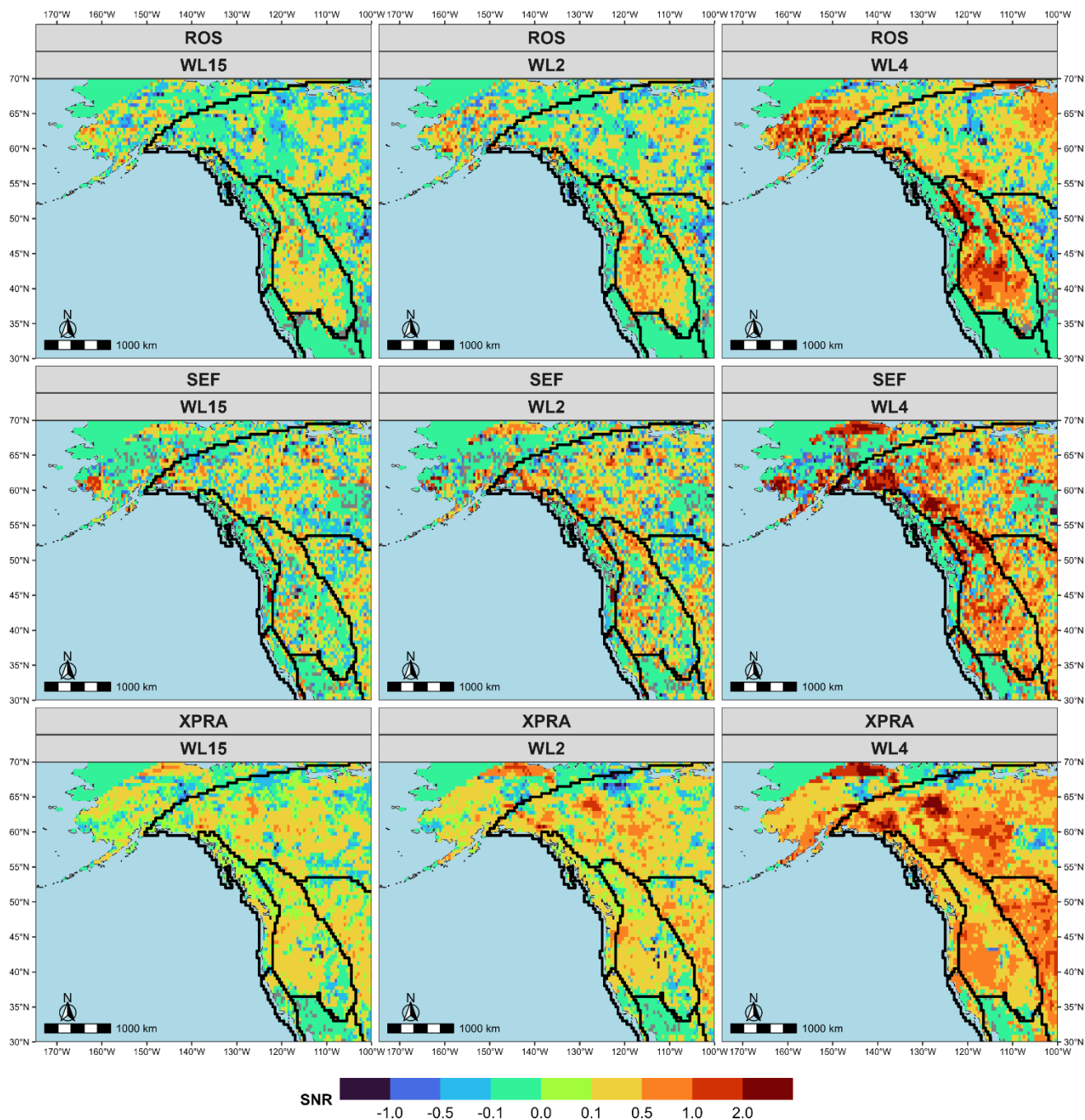
Figure 11: Signal to Noise Ratio for the probability that an event is AR related for each CIF event and extreme precipitation event. The SNR relative to the baseline period is shown for ROS, SEF and XPRA events in the top, middle and bottom rows respectively. Each column depicts a depicts a different warming level for each event, with the WL15, WL2, and WL4 being represented in the left, middle and right columns of plots respectively.
