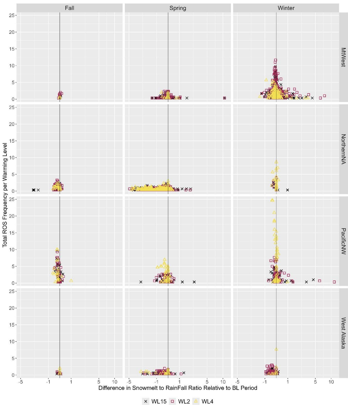
Figure 9: The regional and seasonal difference in snowmelt to rainfall ratio for WL15 ,WL2, and WL4,relative to the baseline period versus ROS event frequency at each grid point. The left, middle and right columns depict results from fall, spring, and winter respectively. From the top, the first, second, third and fourth rows depict the MtWest, NorthernNA, PacificNW and West Alaska regions respectively. The black line in the center of each plot marks zero.
