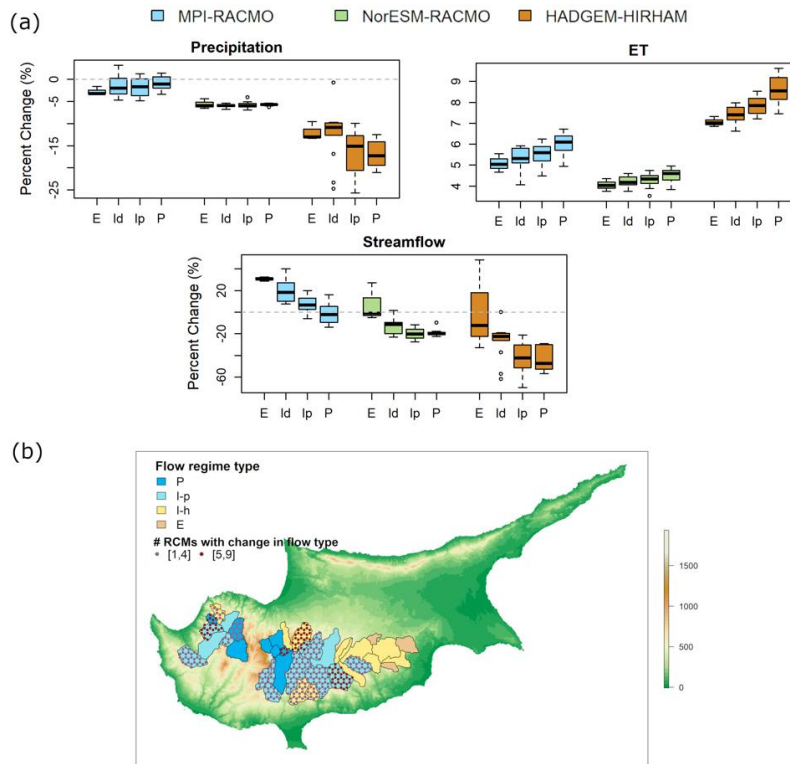
460 Figure 4. (a) Boxplots for the per cent changes in annual precipitation, reference evapotranspiration (ET) and streamflow in the 2030-2060 period relative to the 1980-2010 period simulated by three RCMs (corresponding to minimum, median and maximum streamflow change among nine RCMs) for 38 watersheds grouped by their flow regime type (E-Ephemeral, 3 watersheds, Ih – Intermittent harsh, 13 watersheds, Ip – Intermittent pools, 14 465 watersheds, P – Permanent, 8 watersheds). (b) Elevation map of Cyprus (m) with the flow regime type of the 38 watersheds in the reference period (1980-2010) and the number of models out of the nine RCMs projecting a change in the flow type in the future period (2030-2060).
