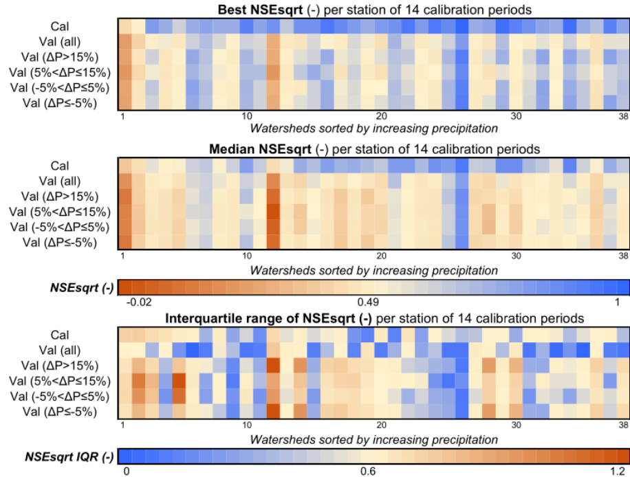
Figure 3 Heatmap with the best (top), median (middle) and interquartile range (IQR) (bottom) of NSEsqr t (-) for each watershed, sorted by increasing long-term annual average precipitation (columns) and each calibration-validation set of runs (rows). The values of NSEsqr t or the IQR for each cell in the heatmap are computed as averages of the values from the 14 5-year calibration runs, the 13 validation runs for each of the 14 calibration runs. i.e., Val (all), and the validation runs corresponding to each of the four precipitation change classes, as specified in Table 1.
