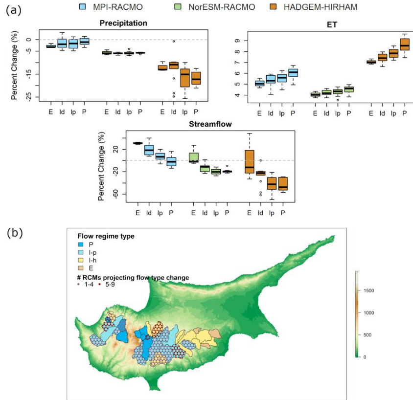
Figure 4. (a) Boxplots for the per cent changes in annual precipitation, reference evapotranspiration (ET) and streamflow in the 2030-2060 period relative to the 1980-2010 period simulated by three RCMs (corresponding to minimum, median and maximum streamflow change among nine RCMs) for 38 watersheds grouped by their flow regime type (E-Ephemeral, 3 watersheds, Ih – Intermittent harsh, 13 watersheds, Ip – Intermittent pools, 14 watersheds, P – Permanent, 8 watersheds). (b) Elevation map of Cyprus (m) with the flow regime type of the 38 watersheds in the reference period (1980-2010) and the number of models out of the nine RCMs ( i.e. 1 up to 4 (1-4) and 5 up to 9 (5-9) ) projecting a change in the flow type in the future period (2030-2060).
